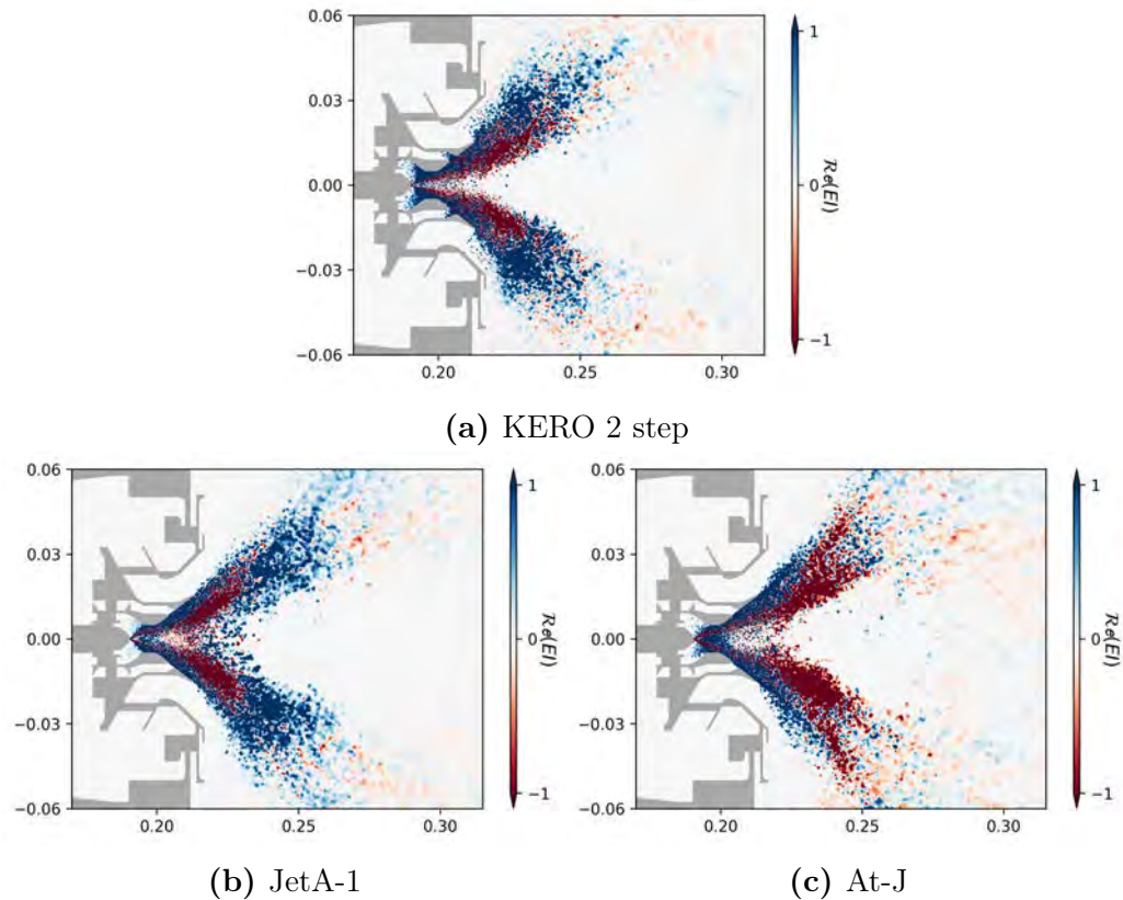
Figure 10.7: Real component of the Evaporation Index.
