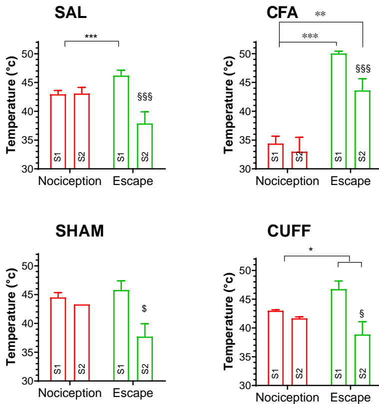
Supplementary figure 2: Nociceptive and escape threshold of Saline-injected (SAL), inflammatory (CFA), sham-operated (SHAM) and cuff-operated (CUFF) animals. Mann Whitney, (***,SSS) p < 0.001 , (**) p < 0.001 , (*;S) p < 0.005 .
