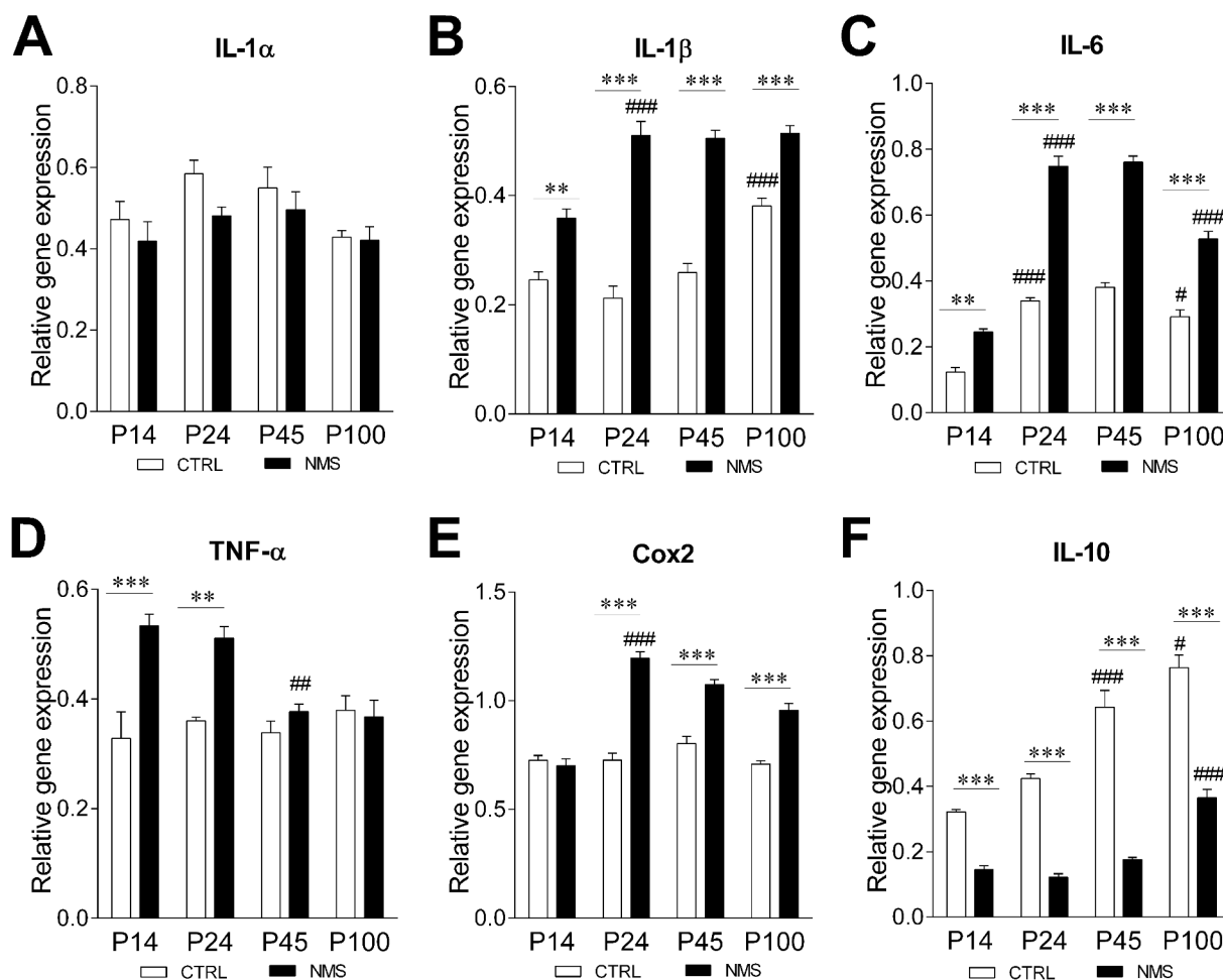
Fig. 6. Relative gene expression (gene of interest / housekeeping gene HPRT) of several inflammatory mediators in the spinal cord of CTRL and NMS rats as measured by RT-qPCR: interleukin-1 \alpha (A, n = 4 per group), interleukin-1 \beta (B, n = 5 per group), interleukin-6 (C, n = 5 per group), tumor necrosis factor \alpha (D, n = 4 per group), cyclooxygenase-2 (E, n = 5 per group) and interleukin-10 (F, n = 5 per group). Statistical significance was assessed with Tukey's multiple comparison post-hoc test, illustrated as follows: p < 0.01 (**), p < 0.001 (***) for CTRL vs NMS and p < 0.05 (#), p < 0.01 (##) or p < 0.001 (###) for intragroup comparison vs preceding time point.
