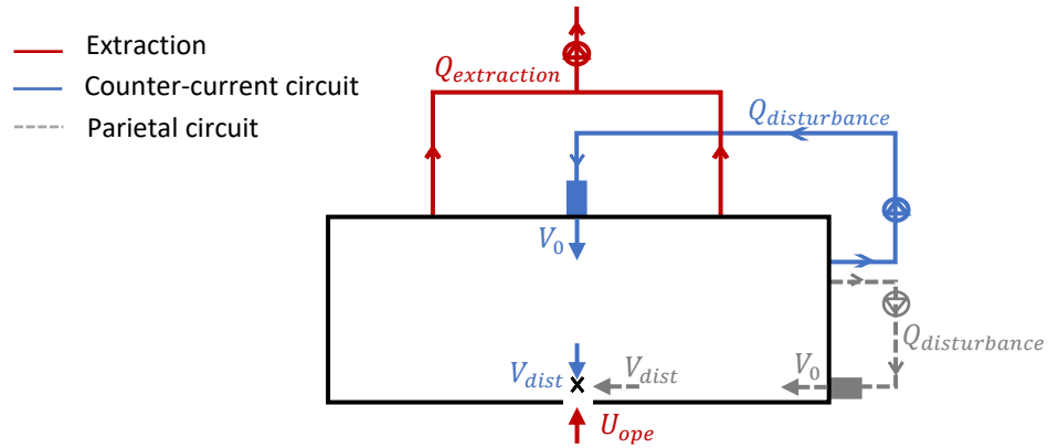
Figure 3-4 Scheme of the two disturbance configurations: counter-current disturbing jet and parietal transverse disturbing jet
