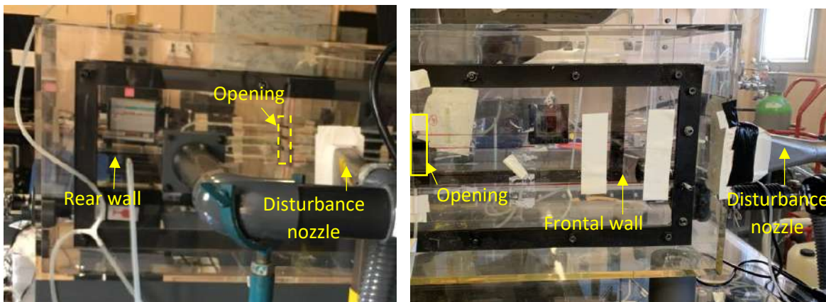
Figure 3-5 Pictures for counter-current disturbance configuration (left) and parietal disturbance configuration (right)
