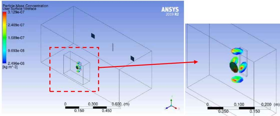
Figure 0-11 Particles mass concentration at the five discs samplers near the opening
