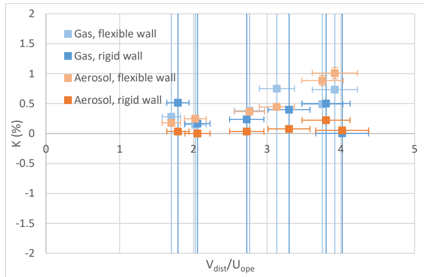
Figure 3-28 Evolution of the backflow coefficient K (%) versus V_{dist}/U_{ope} for an inflow velocity at the opening U_{ope} = 0.5 m/s in the case of an internal parietal free jet disturbance for the gaseous and 5 \mu m particulate pollutant and for the enclosure with rigid and flexible frontal walls respectively
