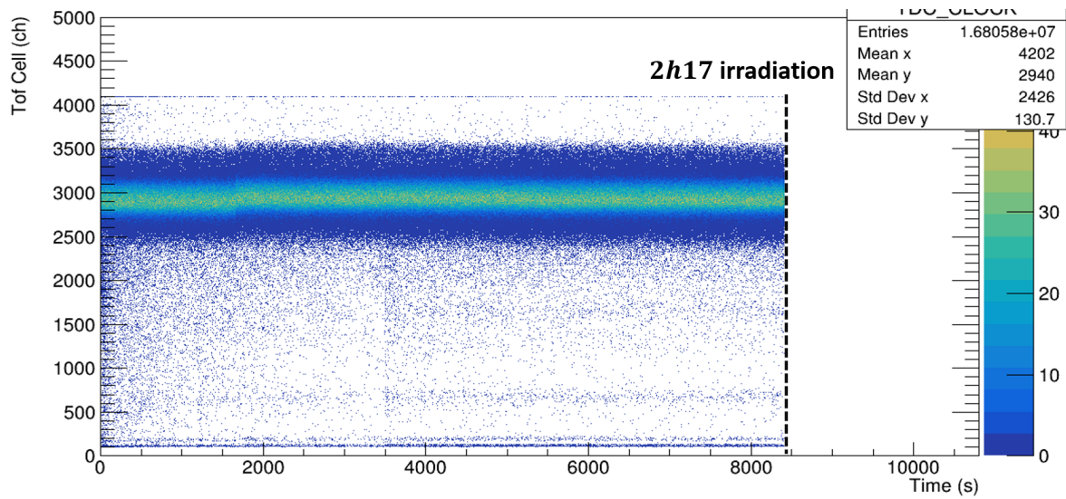
(a) Time response - Si 10 \times 10 \text{ mm}^2 .
