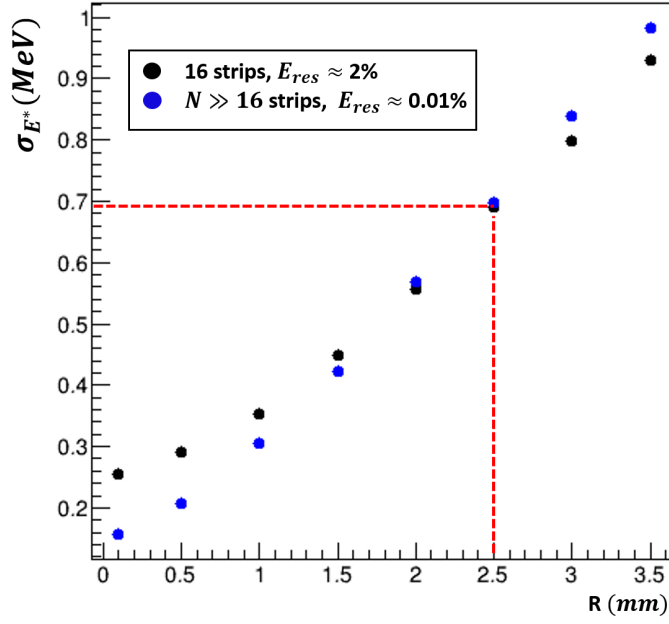
Figure 4.18: The impact of the target radius on \sigma_{E^*} is shown for an ideal set-up (blue circles) and for the set-up used during the proof of principle experiment (black circles).
