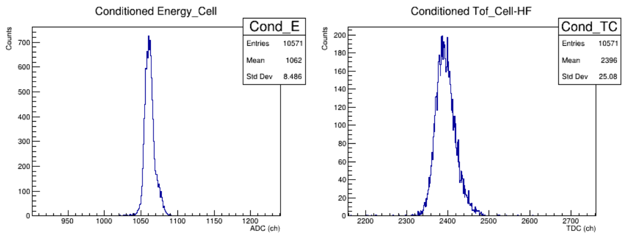
(a) Silicon detector energy spectrum
