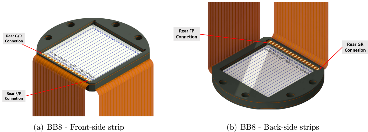
Figure 4.27: Technical drawing of BB8-DSSSD detector used during the experiment. The detectors with a thickness of 529 \mu\text{m} , consisted of 16 front and 16 back strips. The strip signal transmission outside the pocket was ensured by flexi rigid PCBs.
