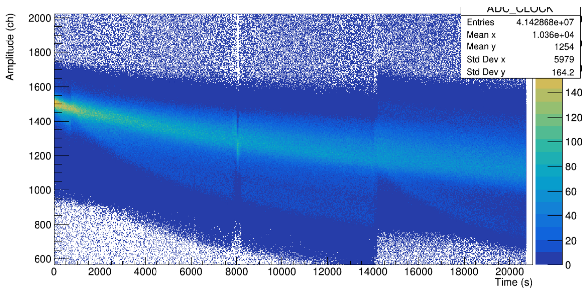
(b) Energy response - space Si 20 \times 20 mm^2 .
