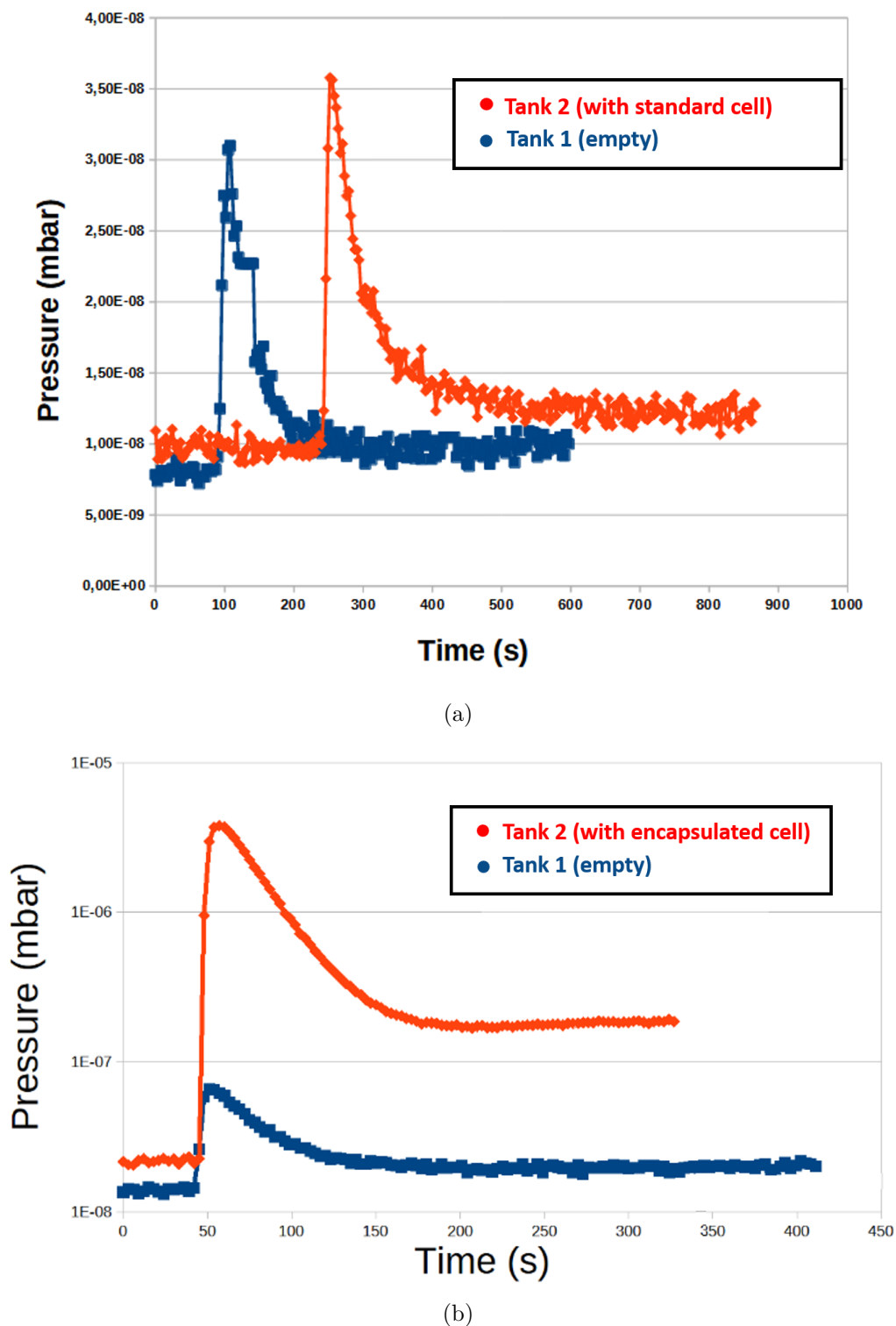
Figure 5.6: Evolution of the pressure after an accumulation of 24 h for a tank housing a sample (in red) and for an empty Tank (in blue) after a heating treatment at 100 °C. Part (a) shows the results for the standard cells and part (b) for the encapsulated cell.
