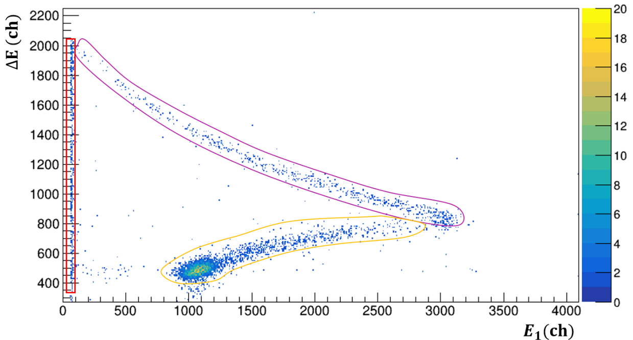
Figure 5.12: Example of identification spectrum measured for vertical strip number 3. The different contours indicate, respectively, the protons stopped in the E_1 detector (in pink), the protons punching through the E_1 detector (in orange) and the low energy protons stopped in the \Delta E DSSSD (in red).
