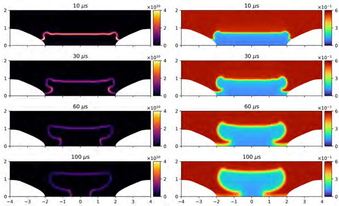
(a) Heat-release [ \text{W}\cdot\text{m}^{-3} ]
