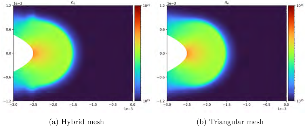
Figure 10.28: Electron density [ \text{m}^{-3} ] at the same time for two hyperbolic shape electrodes with R_c = 200 \mu\text{m} at 1000 K using a hybrid mesh/ISG-LLW hybrid scheme and using a triangular mesh/LLW scheme.
