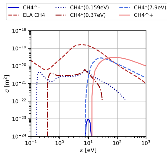
Figure 9.4: \text{CH}_4 cross-sections from the Hayashi database.
