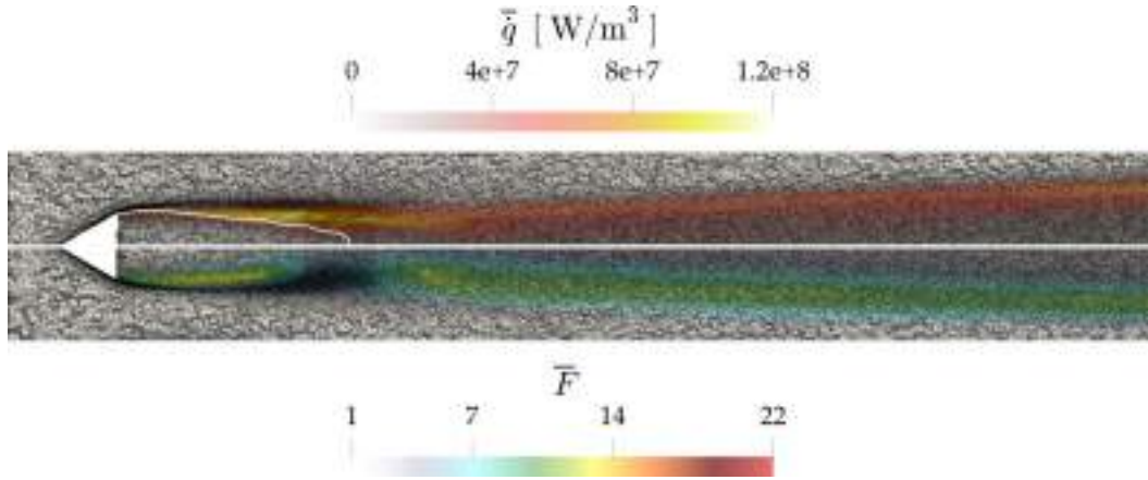
Figure 3.19: Overview of the 46M mesh obtained after the combustion refinement step mesh by using the FET criteria ( \bar{F}_{target} = 15 , \bar{S}_{limit} = 0.1 ). Averaged heat release rate \bar{q} and thickening factor field \bar{F} are superimposed to the grid. The white iso-contour delimits the recirculation zone ( U_x = 0 m/s).
