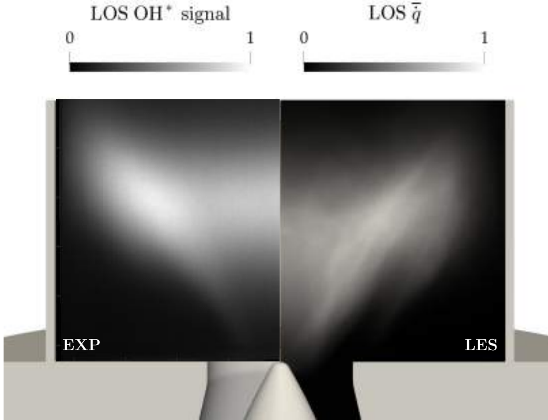
Figure 4.8: Validation of the LES simulations with HRT approach for case P10 . Comparison of experimental normalized time-averaged LOS OH* chemiluminescence image with LOS of predicted heat release rate \bar{q} .
