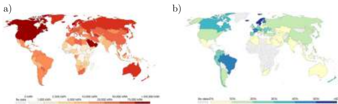
Figure 1.2: Global map presenting (a) the energy use per person and (b) the share of primary energy from low-carbon sources across countries in 2019 [1, 2].
