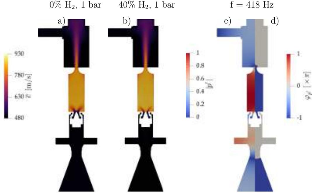
Figure 7.13: LES-predicted time-averaged sound speed field \bar{c} for Cases (a) REF and (b) 1 . (c) Amplitude and (d) phase of the first acoustic (chamber) mode at 418 Hz computed with the Helmholtz solver for Case 1 .
