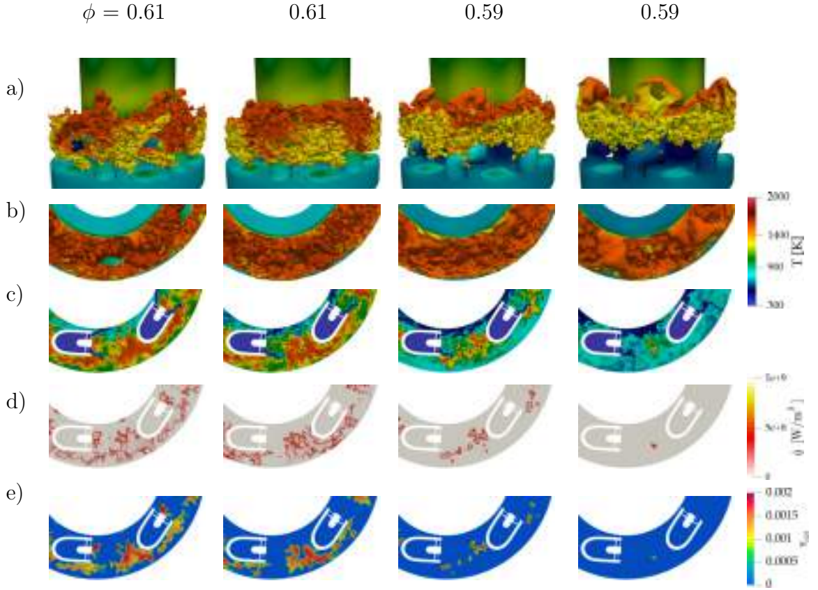
Figure 9.24: CHT LES prediction of flame shape evolution and blow out at different equivalence ratios for Configuration B . (a-b) Isosurface of heat release rate \dot{q} at 10% of its maximum value colored by temperature T . Cut plane showing (c) the temperature T , (d) the heat release rate \dot{q} and (e) the OH mass fraction fields. Images correspond to instants (a), (b), (d) and (g) of Fig. 9.21.
