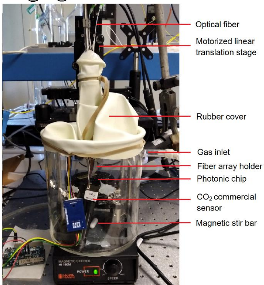
Figure 6.3: Schematic (top) and experimental setup (bottom) of the CO 2 gas sensor
