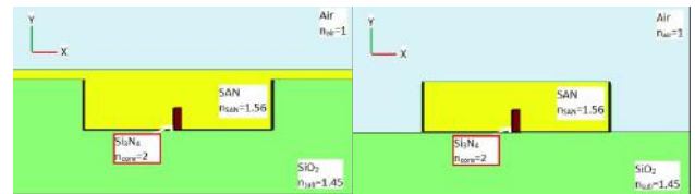
Fig. 6. (a) Rib cladding structure and (b) Strip cladding structure
