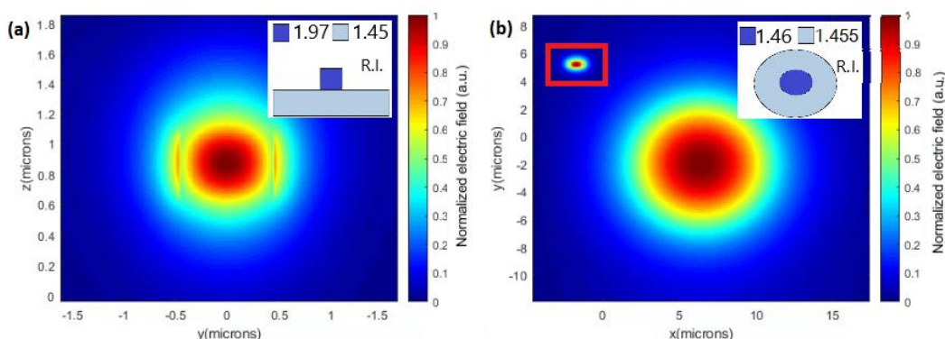
Figure 2.3: Electric field of fundamental modes of (a) 400\text{ nm} \times 800\text{ nm} SiN waveguide and (b) single mode fiber (SMF-28), with SiN waveguide mode for scale
