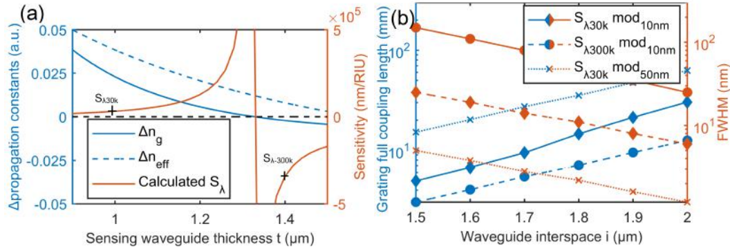
Figure 5.18: (a) GI and EI difference between coupling modes, and resulting estimated S_\lambda as a function of t ; (b) grating length for full coupling and simulated FWHM at 1550 nm (log scale)
