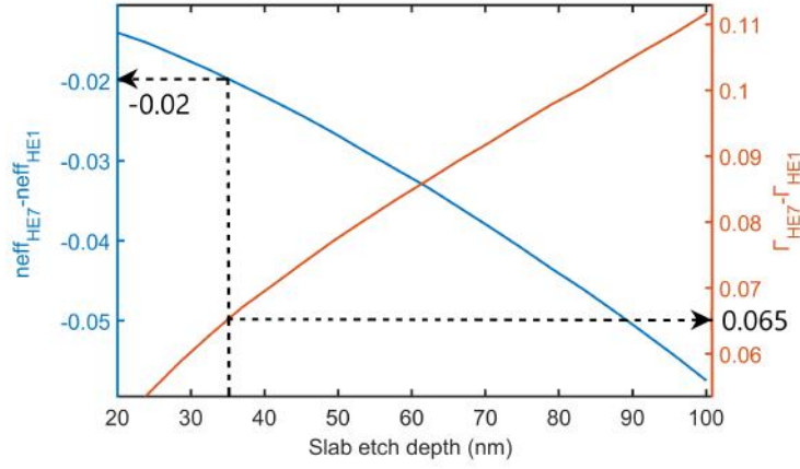
Figure 5.9: EI difference and variation of \Delta\Gamma of coupling modes as a function of slab etch depth e with w_{slab} = 30 \mu m and w_{core} = 1.65 \mu m at 1550 nm. e is set at 35 nm and h_{slab} = 365 nm. Dashed lines: selected e with corresponding \Delta n_{eff} and \Delta\Gamma .
