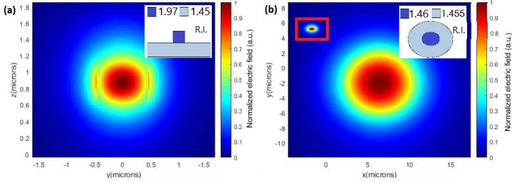
Figure 2.3: Electric field of fundamental modes of (a) 400 nm \times 800 nm SiN waveguide and (b) single mode fiber (SMF-28), with SiN waveguide mode for scale
