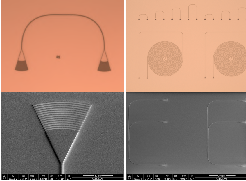
Figure 2.12: Images of fabricated devices of chips n° 1 and n° 2: (a) optical micro-scope (OM) image of grating coupler pair for chip in/out coupling, (b) OM image of spiral waveguide designed for waveguide loss measurement, (c) SEM image of fabricated grating coupler, and (d) SEM image of fabricated broadband coupler
