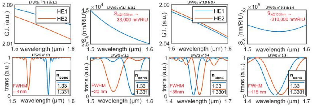
Figure 5.19: GI profiles, simulated transmission spectra (trans) and spectral sensitivities ( S_\lambda ) of different versions of LPWGs (n° 3.1-n° 3.4) for which the structure parameters are detailed in Table 5.2
