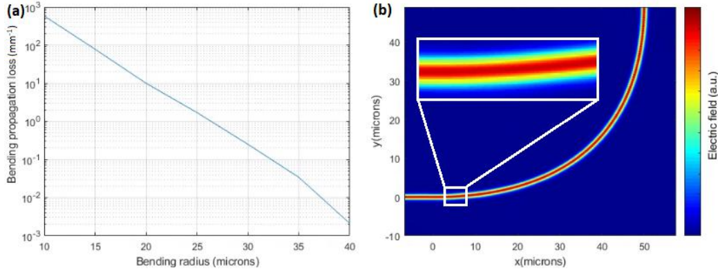
Figure 2.4: (a) Simulated propagation loss versus bend radius, simulated with FDE with conformal mapping, and (b) 2.5D FDTD simulation of Bezier-apodized waveguide curvature with 50\ \mu\text{m} average bending radius
