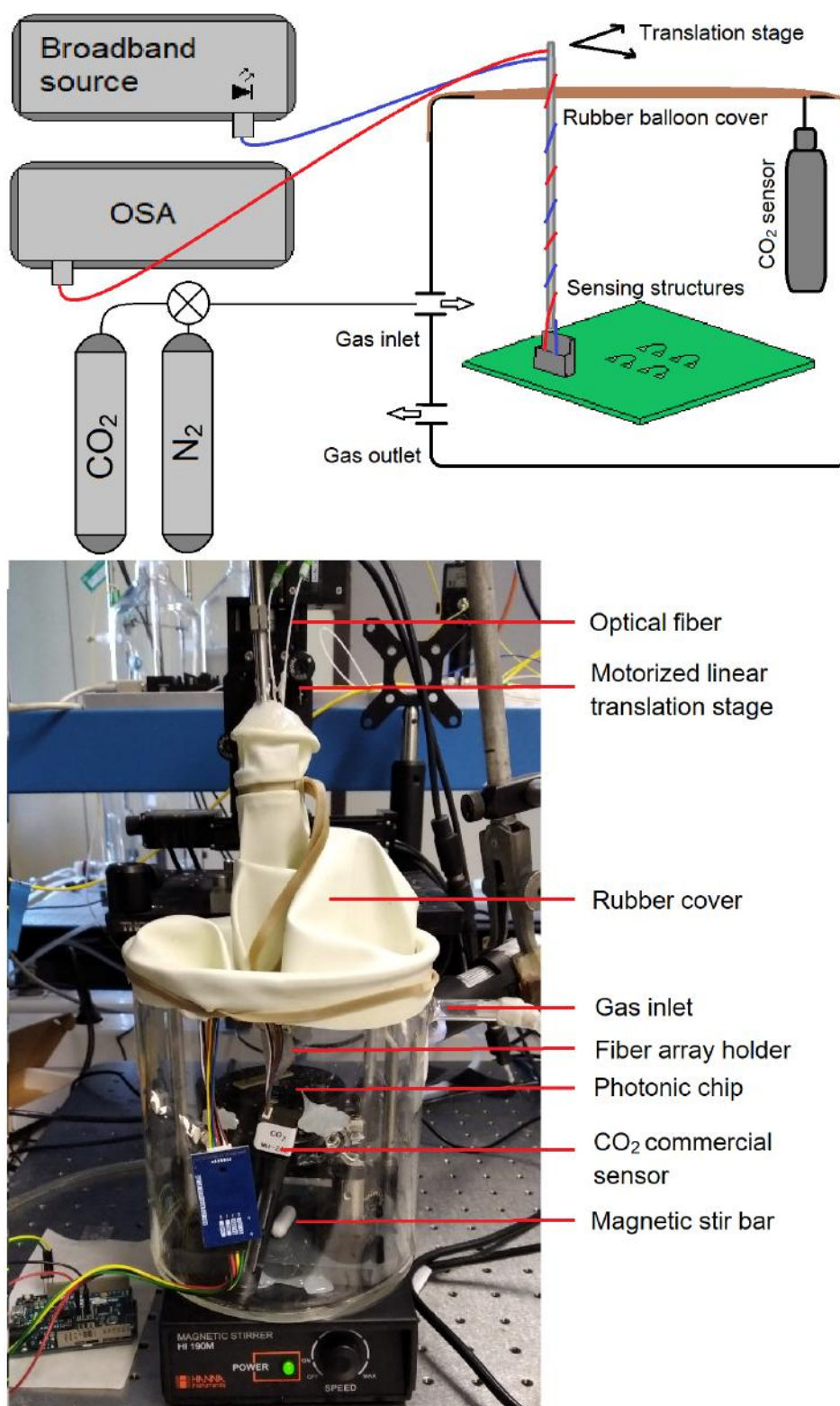
Figure 6.3: Schematic (top) and experimental setup (bottom) of the CO 2 gas sensor
