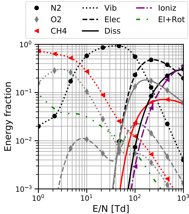
Figure 7.1: Discharge energy branching in stoichiometric methane-air mixture computed using BOLSIG+ [72]
