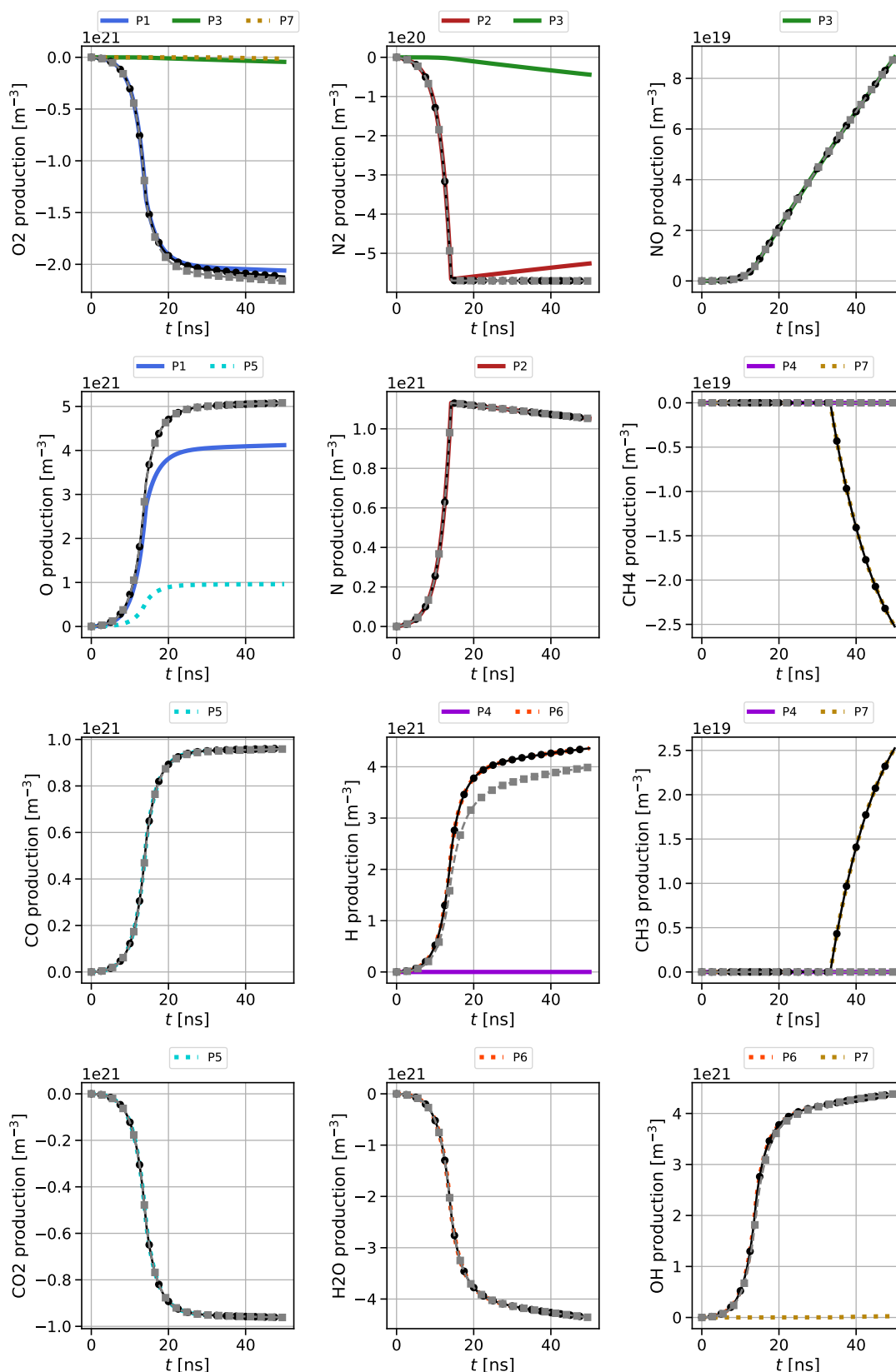
Figure 10.8: Comparison of the species production predicted by improved model (Black Solid) with the results of the detailed simulation (Gray Dashed) for the lean flame \phi = 0.7 at \mathbf{c} = \mathbf{1} . Colored curves correspond to the production of each global process of the improved model (see Tab. 10.1) with process number in the legend.
