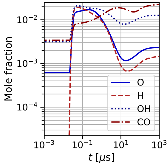
Figure 8.15: Long term evolution of the radicals produced by the discharge in Case F.
