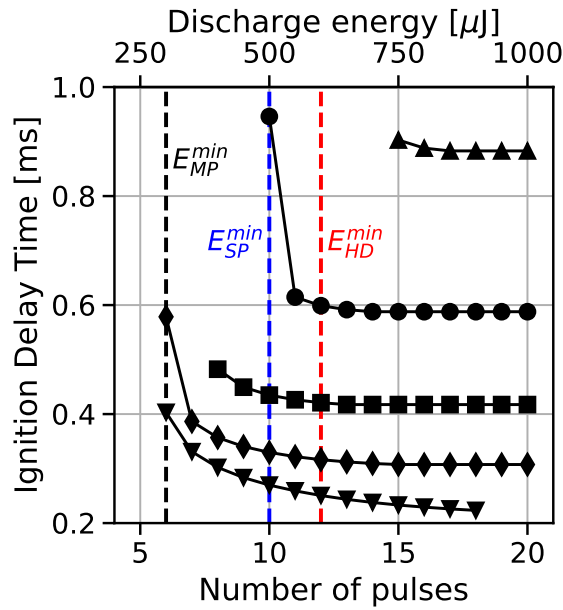
Figure 13.12: Ignition delay time depending on the number of pulses at various frequencies: ▲ 20 kHz ● 25 kHz ■ 33 kHz ◆ 50 kHz ▼ 100 kHz. The corresponding total discharge energy is indicated on the top axis of the figure. E_{HD}^{min} , E_{SP}^{min} and E_{MP}^{min} correspond respectively to the minimum energy ignition of the HD, SP and MP cases.
