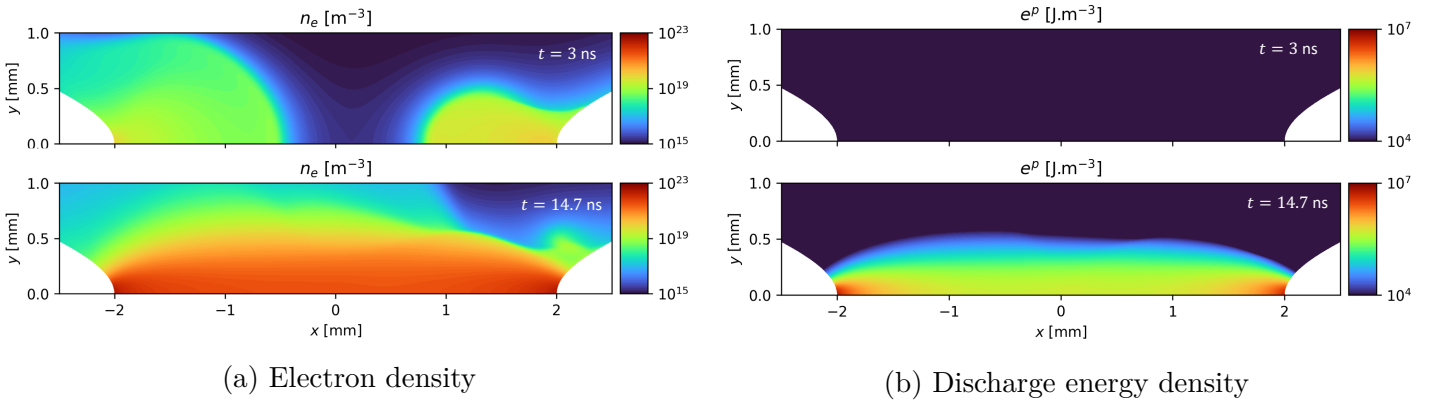
Figure 13.3: Two-dimensional fields for the single-pulse discharge at different instants.
