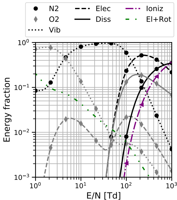
Figure 6.1: Discharge energy branching in air ( X_{O_2} = 0.2 , X_{N_2} = 0.8 ) computed with BOLSIG+ [72].
