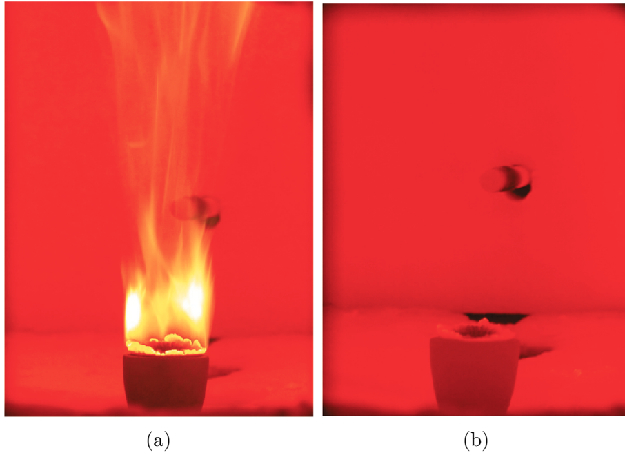
Figure 1.7: Combustion furnace operating on natural gas with a 10 kW heat input for (a) conventional combustion and (b) MILD combustion [Reproduced from [50]]
