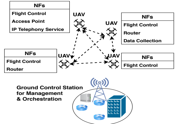
Figure 4.6: UAVs with diverse network functions
