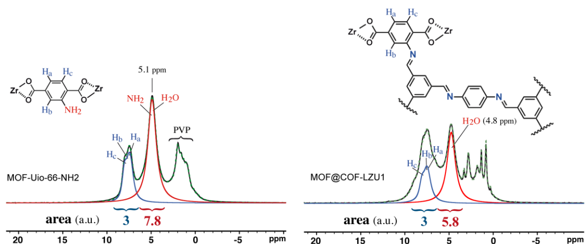
Figure 3-15 Ultra-Fast MAS 1 H NMR of MOF-Uio-66-NH 2 (left) and MOF@COF-LZU1 (right). For the sake of clarity, only CHs and NH 2 /H 2 O components are shown. Black: experimental, dotted green: calculated spectrum, blue: sum of fitted CHs, red: H 2 O+NH 2 or H 2 O.
