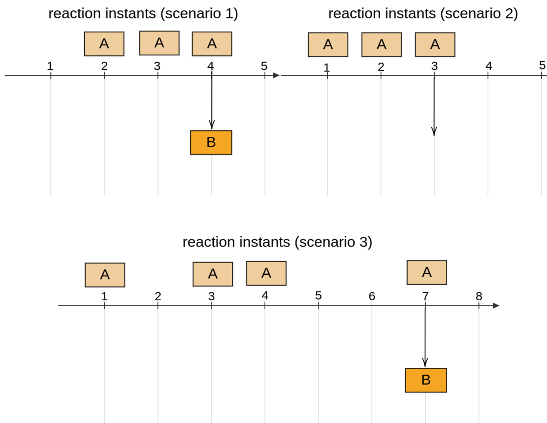
Figure 2.15: await count example timeline.
