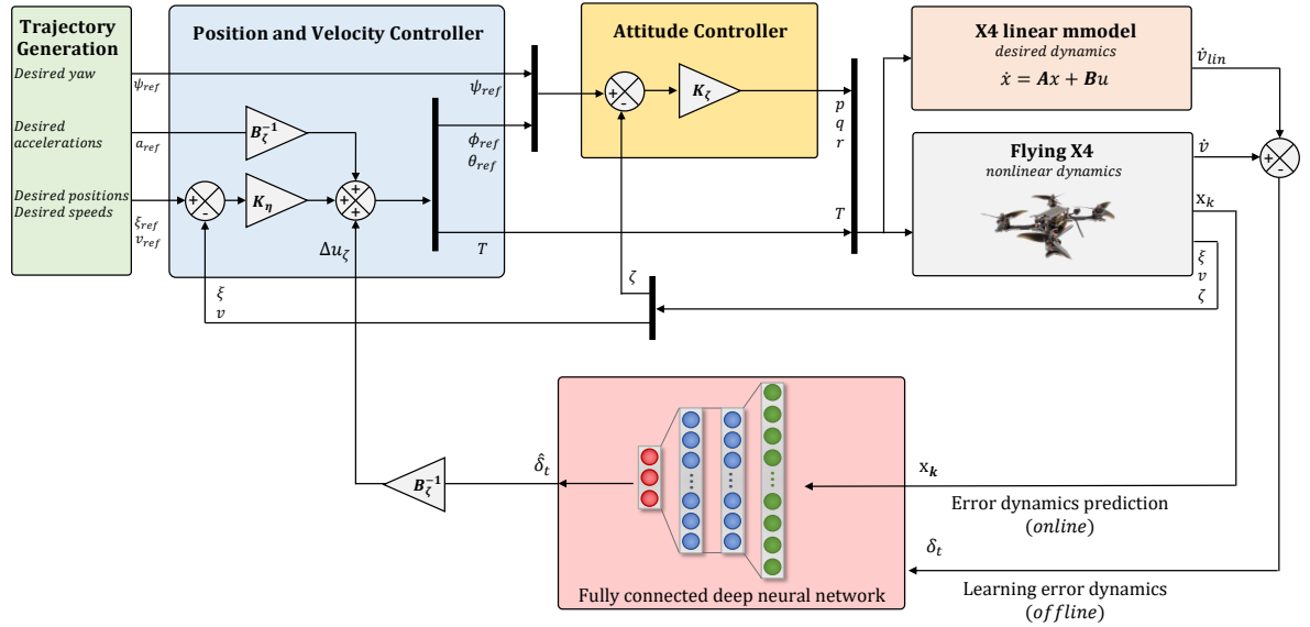
Figure III.5: DNN-enhanced linear controller architecture
