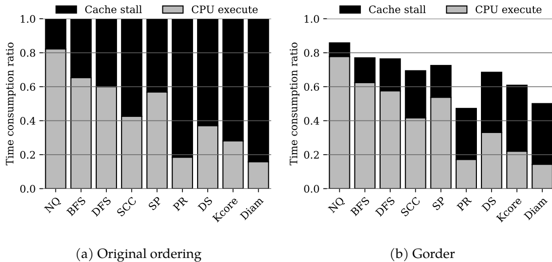
Figure 4.2: CPU execution and cache stall. Original ordering and Gorder are compared for all algorithms on the sdark dataset. Grey bars are time spent on CPU operations, black bars represent time spent waiting for data retrieval. Times are normalised by the total runtimes with the original ordering. Figure (a) shows the share of CPU execution and cache stall for the original ordering, figure (b) shows them when the network has been reordered following the Gorder procedure. While both need about the same CPU time, the latter is significantly faster due to cache stall reduction. Compare to Figure 1 in Wei et al. [2016].
