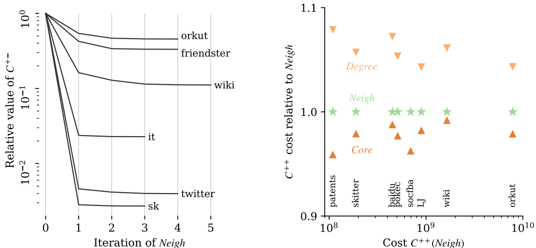
(a) Convergence of Neigh heuristic for cost C^{+-} on the biggest datasets. Each line shows the relative reduction of C^{+-} after a certain number of iterations. They stop when relative improvement is under 10^{-2} . (b) Value of Neigh heuristic applied on C^{++} cost function, compared to degree and core orderings. Values are normalised by C^{++}(\textit{Neigh}) . Observe that Neigh is always between core and degree.
