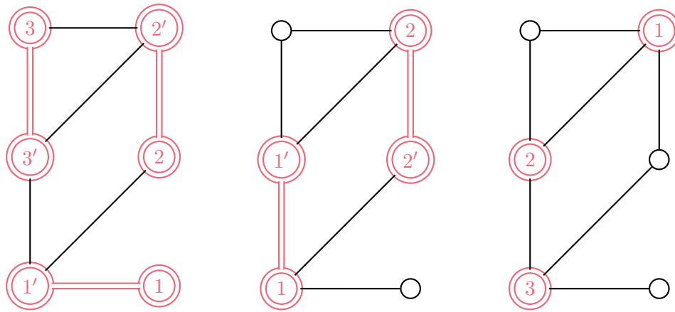
Figure 6.1: Greedy heuristics for vertex cover. On a toy example, we show the vertex covers obtained from different greedy heuristics. In all cases, the numbers indicate the step at which a node has been selected by the corresponding algorithm. On the left and middle cases, the red double lines indicate the matching that produced the cover. Left: edge-greedy (Algorithm 6) with low-degree first \eta_{low} leads to a maximum matching. Middle: edge-greedy with high-degree first \eta_{high} gives a matching with 4 nodes. Right: node-greedy (Algorithm 7) with high-degree first \nu_{high} gives a cover of 3 nodes; it is optimum because the left cover has 6 nodes and is a 2-approximation.
