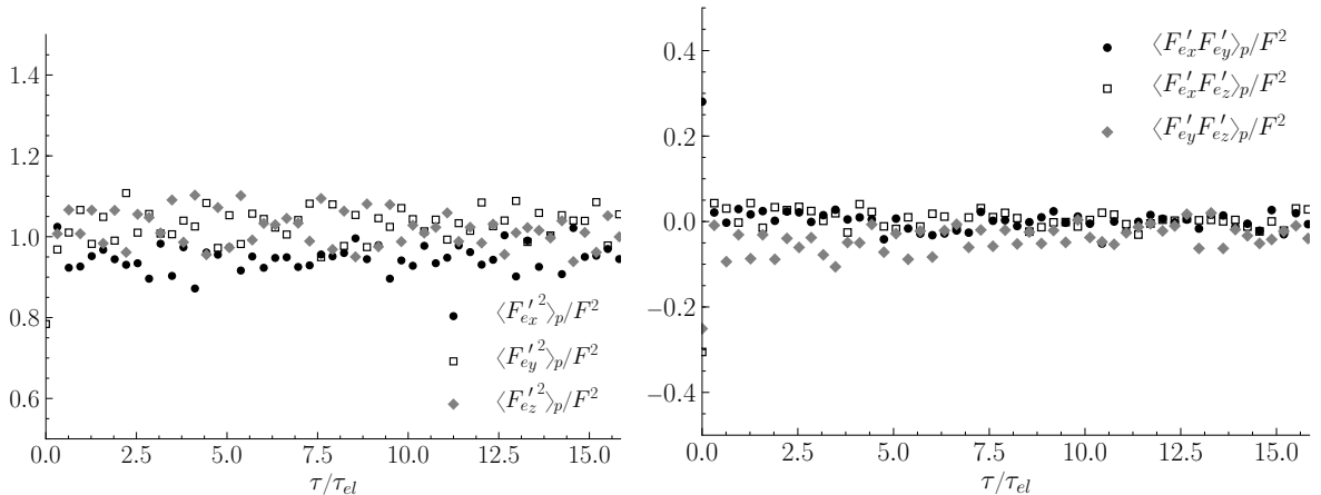
(a) Diagonal elements Eq. (4.6a).
