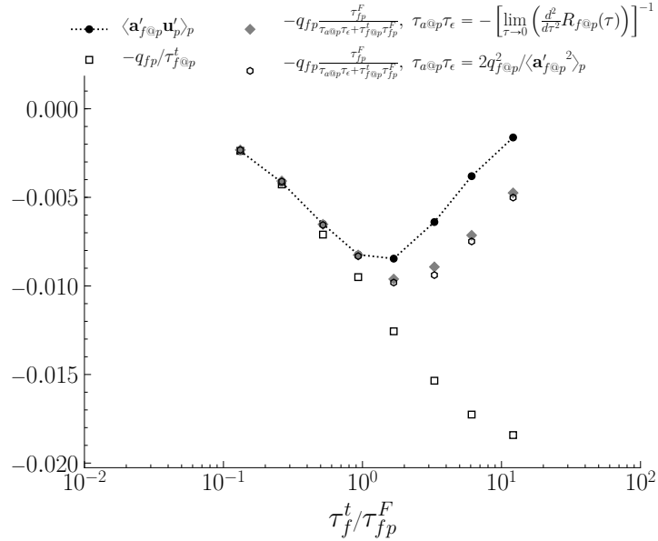
Figure 5.9: Comparison between DNS results ( \bullet ) and the predictions of the Langevin model ( \square ) and the introduced stochastic model ( \blacklozenge , \circ ) of the fluid acceleration - particle velocity covariance \langle \mathbf{a}'_{f@p} \mathbf{u}'_p \rangle_p with regard to particle Stokes number for Q_p = 5Q_0 .
