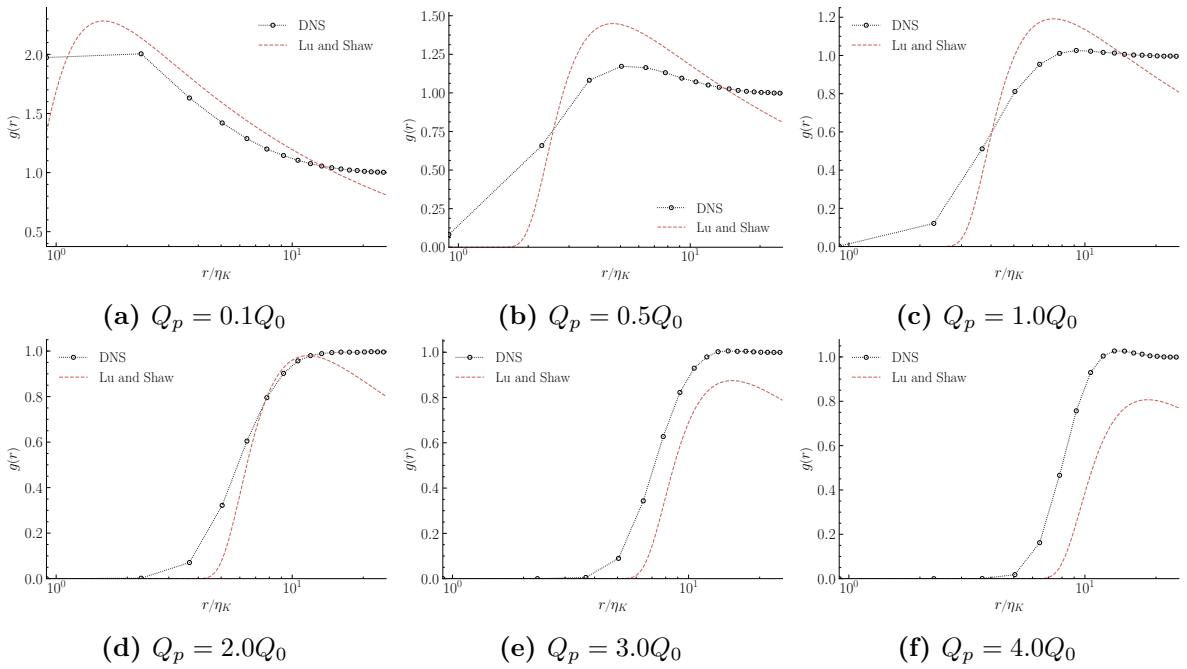
Figure 5.44: RDFs of the lighter particles compared with Lu & Shaw (2015) model of Eq. (5.17) for various levels of electric charges. We observe an agreement on the trend of the evolution of RDFs for weak electric charges, one of the hypotheses of the cited model.
