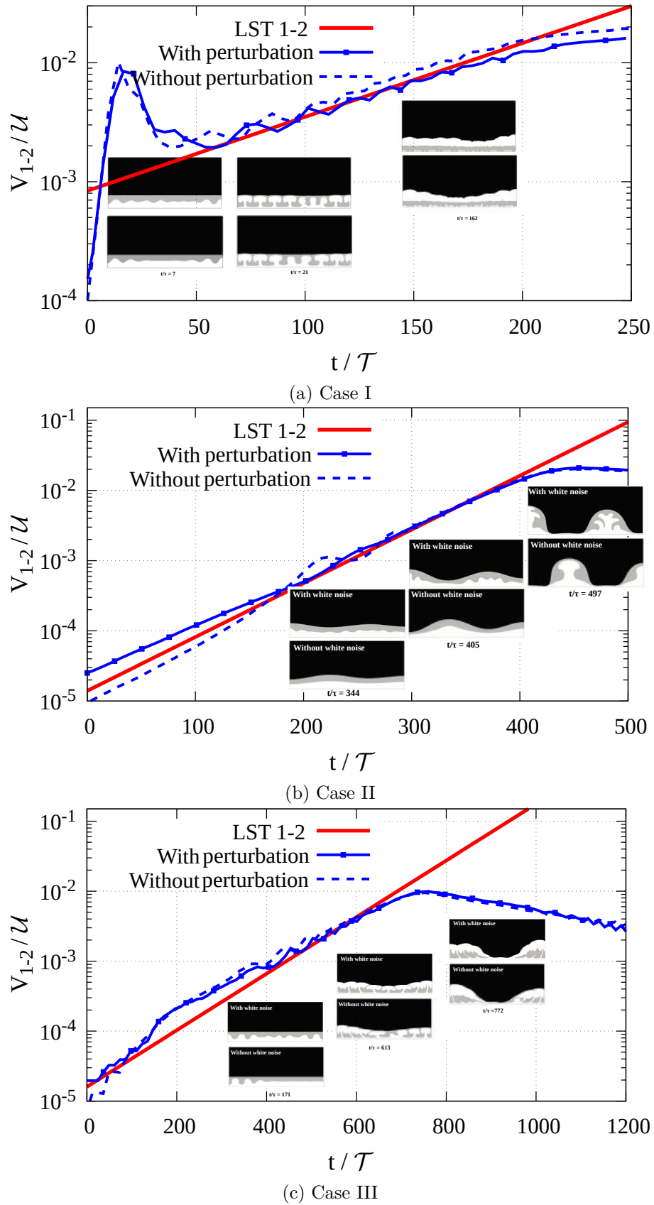
FIGURE 2.1.19 – Case I (a), II (b) and III (c) of WEINBERG et SCHMELING [1992] : time evolution of the velocity of the maximum height of interface 1-2 : with or without an initial random perturbation at interfaces (JADIM code, harmonic viscosity averaging), compared to linear stability theory (RAMBERG [1981a]). Time is scaled by \mathcal{T} and t/\mathcal{T} = 0 is set as the time when one of the interface has raised by a distance of 3 \times 10^{-5}H .
