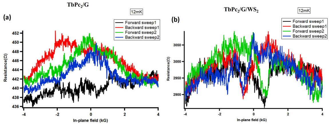
Fig. 6.5.1 The magnetoresistance of \text{G}/\text{TbPc}_2 by sweeping in-plane magnetic field four times between \pm 4000 Gauss at 12 mK. (b) Same measurement in \text{WS}_2/\text{G}/\text{TbPc}_2 sample.
