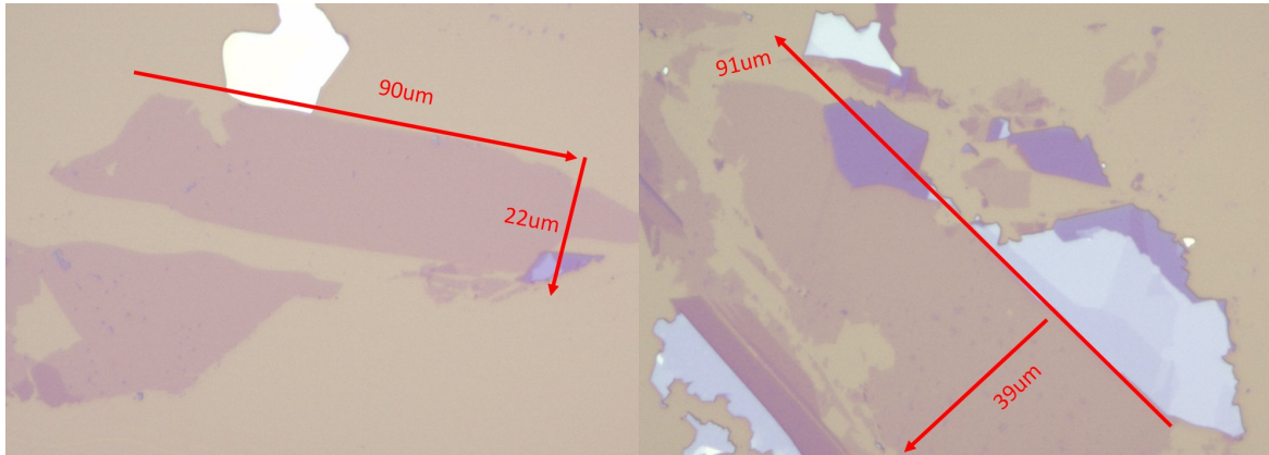
Fig. 3.2.2 Au-assisted exfoliation result of the two different tungsten disulfide ( \text{WS}_2 ) monolayers with large size.
