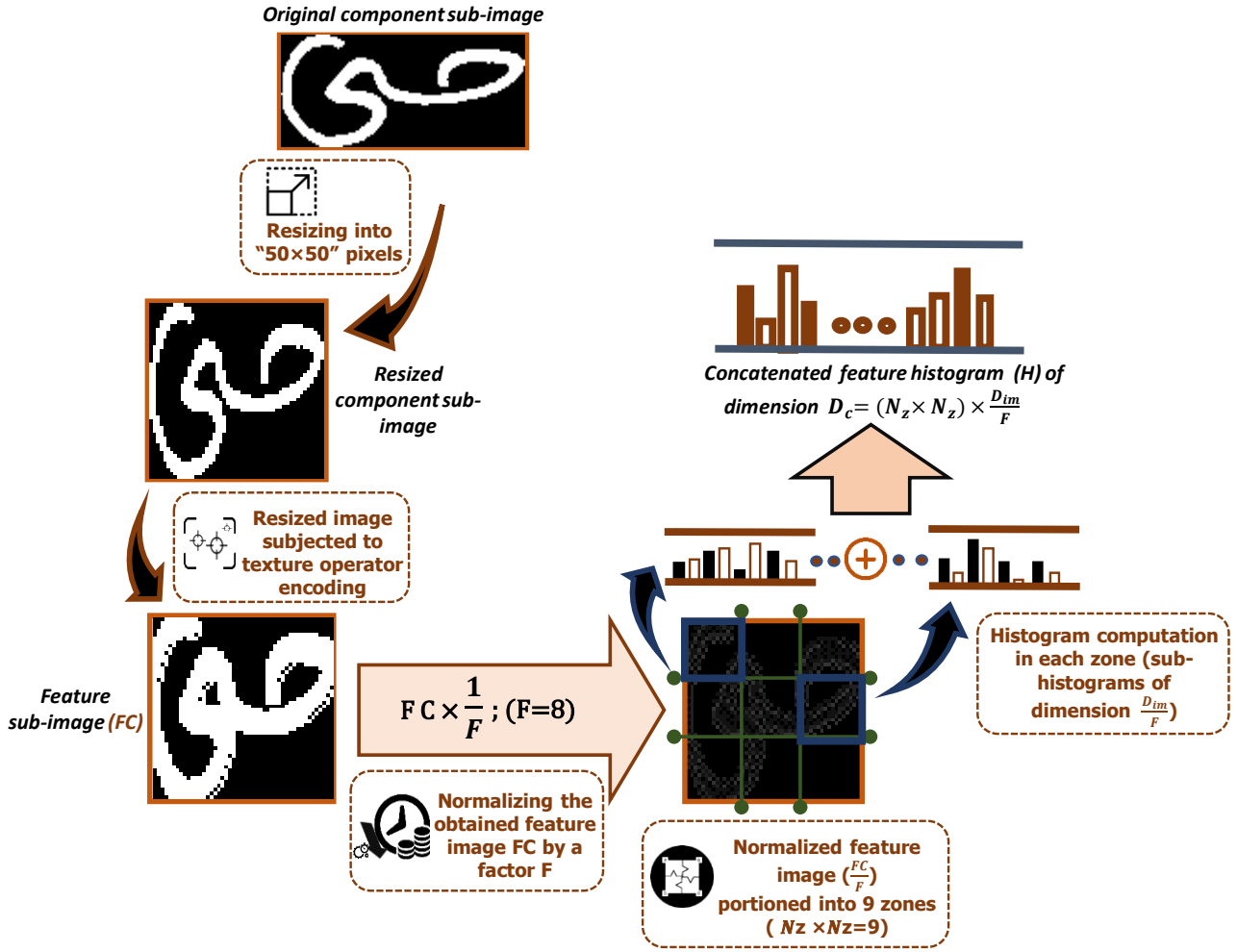
Figure 3.8: The proposed feature extraction process.
