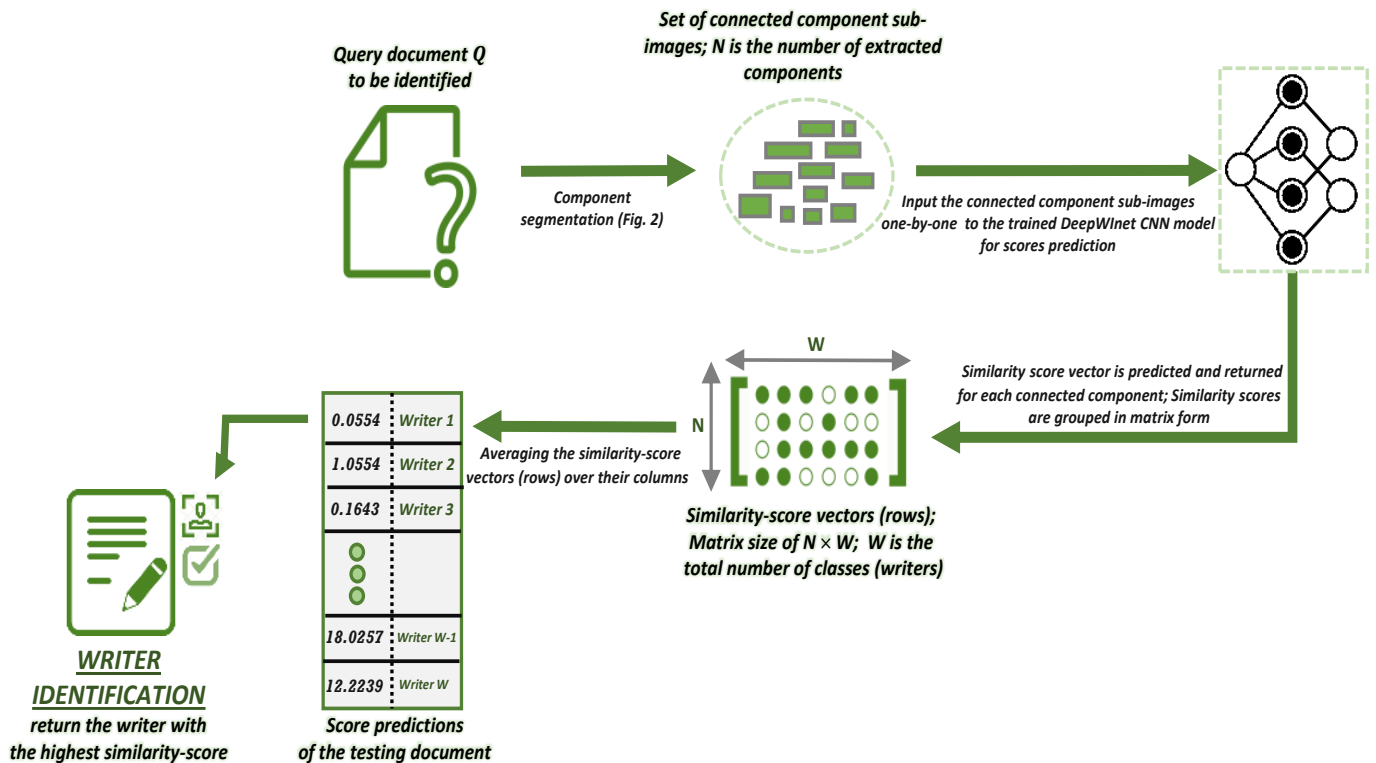
Figure 4.10: Writer identification using scores averaging.
