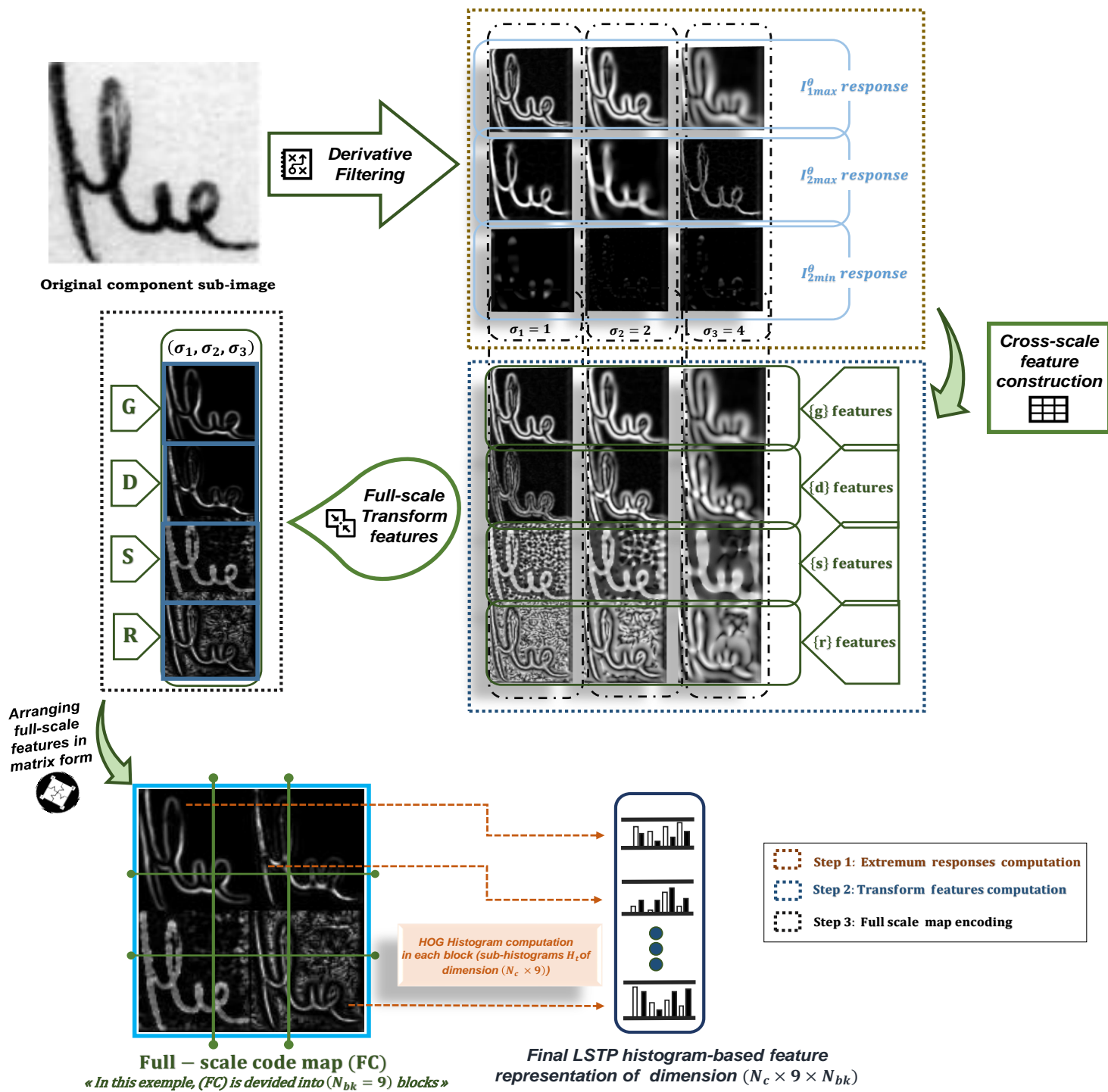
Figure 3.10: The proposed LSTP feature extraction method.
