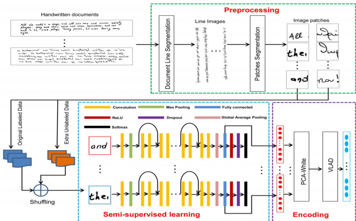
Figure 2.31: The pipeline of semi-supervised feature learning, which consists of three parts: preprocessing (green dotted box), semi-supervised learning (blue dotted box) and encoding (purple dotted box) (Chen et al. (2019)).
