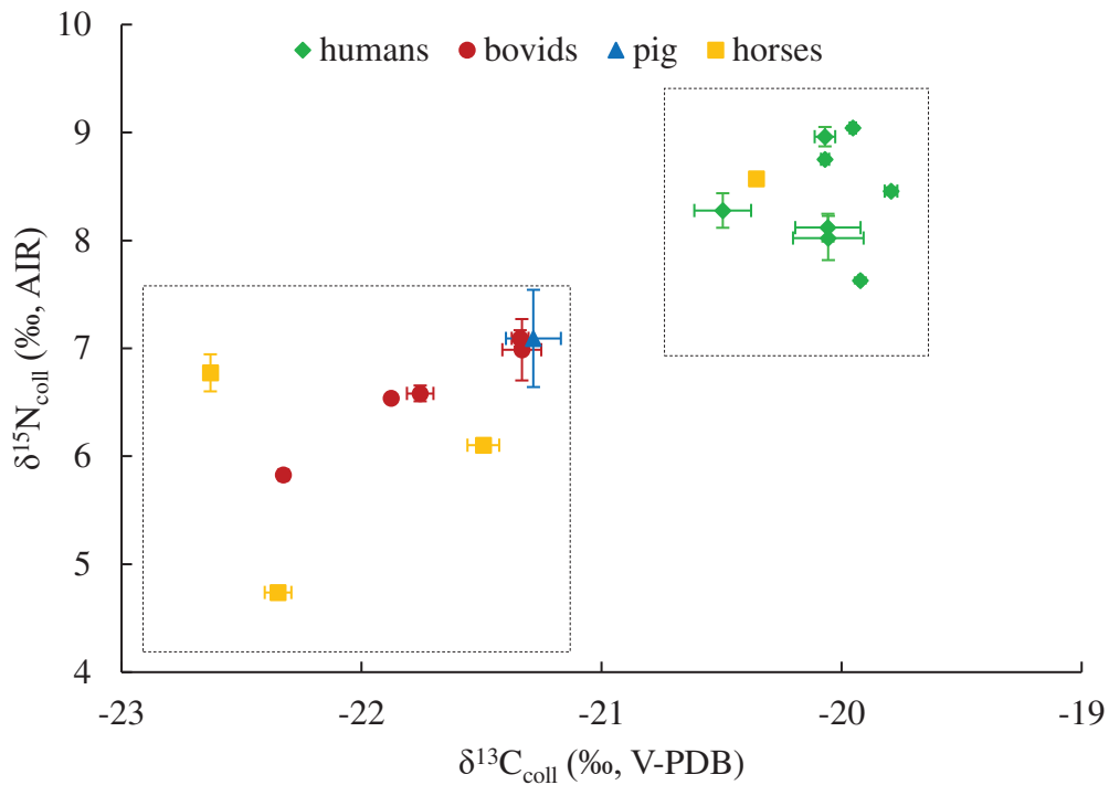
Fig. 3: \delta^{15}\text{N} Nitrogen (‰, AIR) and \delta^{13}\text{C} carbon (‰, V-PDB) isotope values of the bone collagen from humans and animals found at Thézy-Glimont. Humans, bovinds and horses are represented on the x-axis by increasing sample number from left to right. The two squares distinguish between the main herbivores (bovinds, horses, pig) and omnivores (humans).
