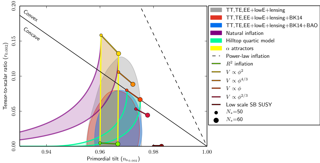
Figure 2.10: Planck 2018 results on single field slow-roll inflationary models from the Planck Image Gallery . It displays the posterior distribution of the primordial tilt n_s on the horizontal axis and of the tensor-to-scalar ratio r on the vertical axis. The grey, red and blue contours are the 1\sigma and 2\sigma allowed region of parameter space from CMB and LSS (when BAO are included) datasets. If some models are excluded from the data, current observations are far from singling out a single inflationary models.
