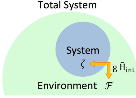
Figure 3.4: Schematic setup of the OQS considered. The system, made of the degree of freedom \zeta , evolves freely according to \hat{H}_S and is embedded in the environment made of \mathcal{F} controlled by \hat{H}_E . Their interaction is specified by g\hat{H}_{\text{int}} . From the point of view of the system, this interaction renormalizes its energy level, generates energy losses and gains described by dissipation and information exchanges captured by decoherence. Figure adapted from [253].
