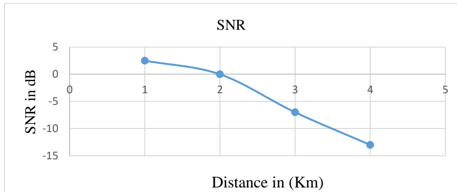
Figure 3-15: SNR Variation
