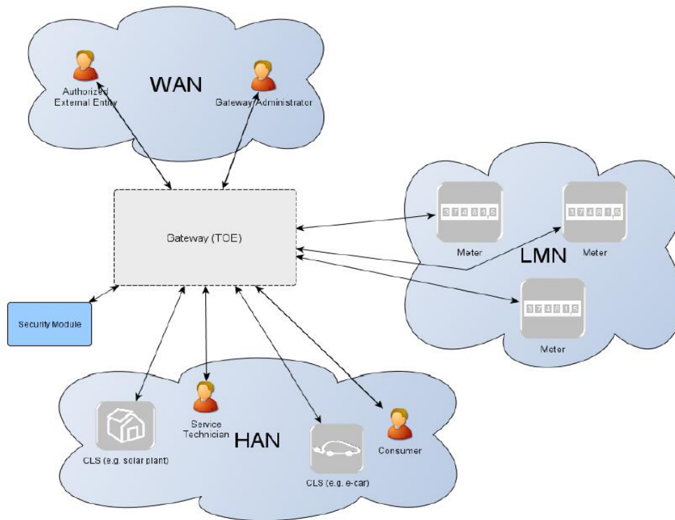
Figure 2-9: iMSys Functional Units [43].
