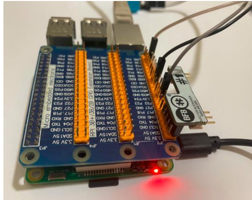
Figure 5-15: Hardware Connectivity
