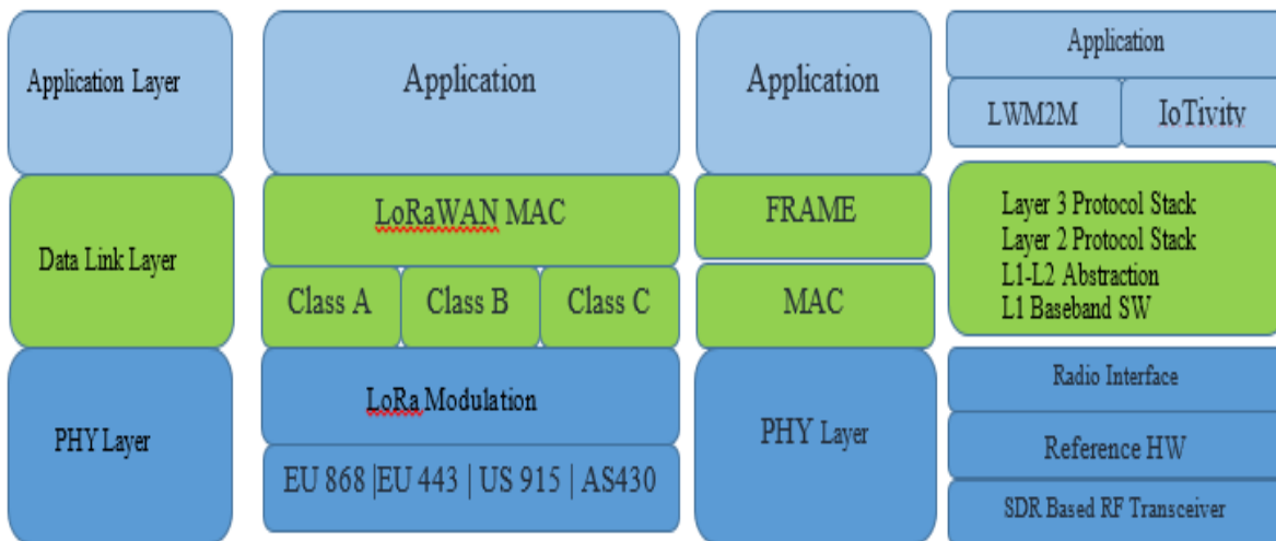
Figure 1-8: Wireless M-bus, LoRaWAN, Sigfox, and NB-IoT Protocols Stack.
