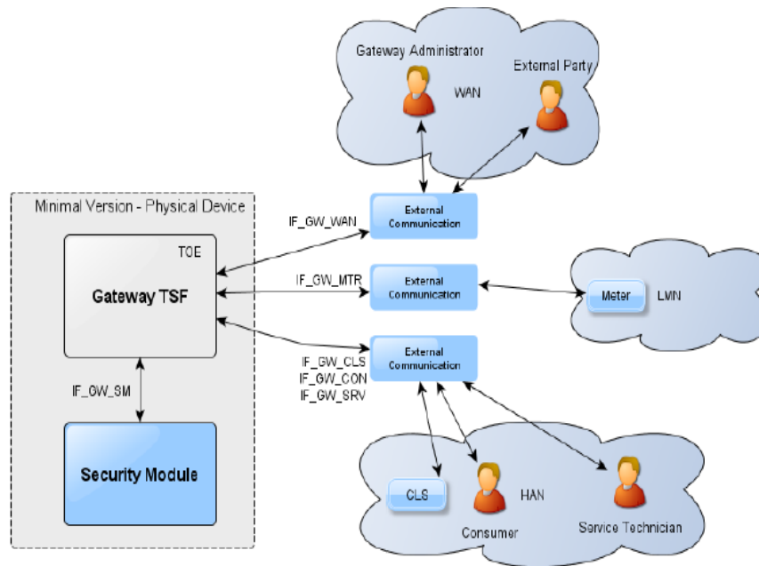
Figure 2-12: Minimal Implementation [43]
