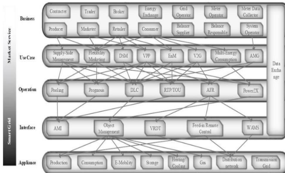
Figure 2-3 IoE Architecture [9]
