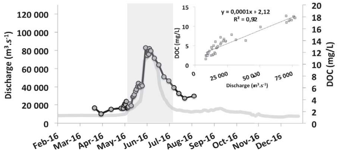
Figure 2. 7 DOC concentrations (mg/L) along with daily discharge. Grey dots are point measurements, grey line represents daily discharge ( m^3.s^{-1} , source: Roshydromet), grey rectangle delimitate freshet periods. Right side graph shows the relationship between daily discharge and DOC concentration.
