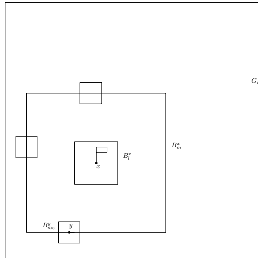
Figure 6.2 – Idea of proof of Lemma 6.15: if a vertex x is connected to a fixed finite cycle of weight larger than 1, vertices which are far enough from this cycle are not connected to x .
