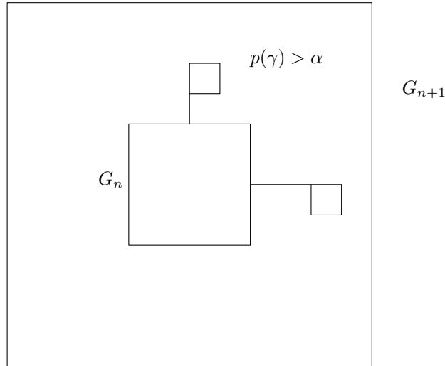
Figure 5.2 – Assumption 5.1
