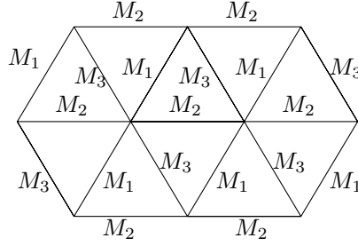
Figure 4.2 – Triangular planar lattice endowed with a periodic connection h .
