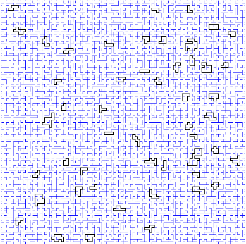
Figure 5.1 – Simulation of an ECRSF for p : \gamma \mapsto 0.75 and c = 1 .
