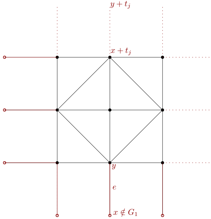
Figure 4.1 – G_1 contains all solid edges and all full vertices. Once the boundaries are glued on the torus, red vertices are glued to corresponding black vertices and the connection is multiplied by z_j on red edges.
