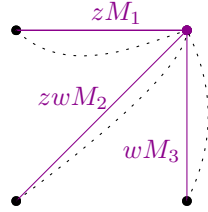
Figure 4.3 – The fundamental domain on the torus \tilde{G}_1 endowed with the connection h(z, w) .
