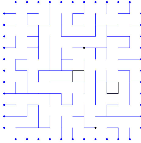
Figure 2.1 – Simulation of an EVCRSF for c = 1, p = 0.75, m = 0.01 and W the boundary of the square grid.
