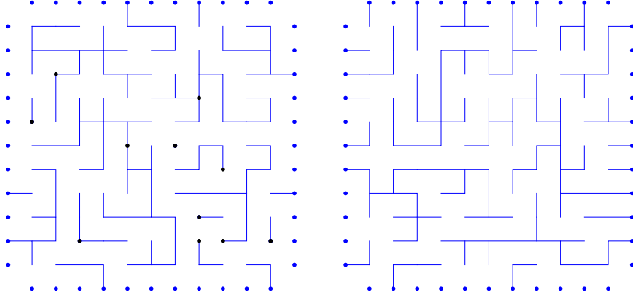
Figure 2.2 – Simulation of an ERSF for p = 0, m = 0.01 and of an ESF for p = 0, m = 0 . The marked points inside are the roots of the configuration.
