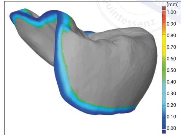
Fig 6 Marginal area inspection of the CAD model.
