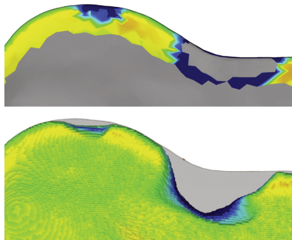
Figure 7. Map of peripheral region of interest projected on computer-aided design presenting one "undefined" defect at top and global mapping projected on mesh of corresponding prosthesis at bottom.
