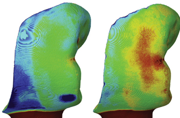
Figure 6. Comparison of marginal limit region of interest on specimen of Tetric CAD (left) and e.max CAD (right).
