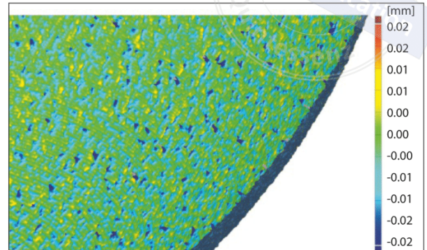
Fig 3 Enlargement of the form deviation map of the digitized ceramic ball.
