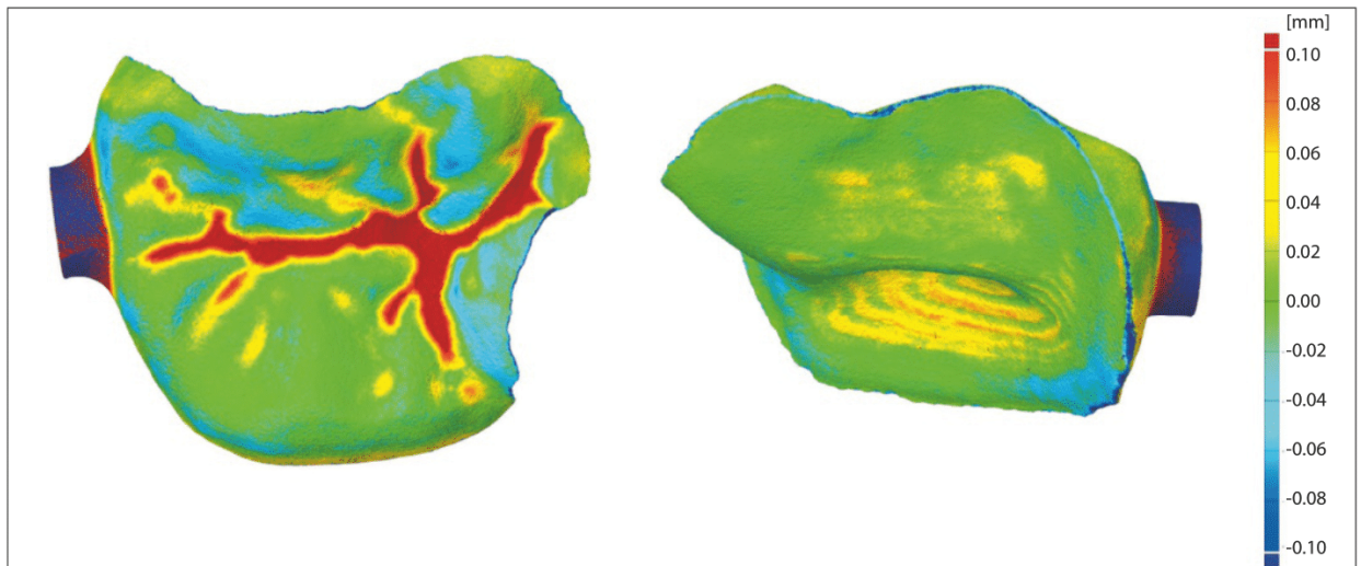
Fig 4 Analysis of distances between the CAD model and the digitized prosthesis.
