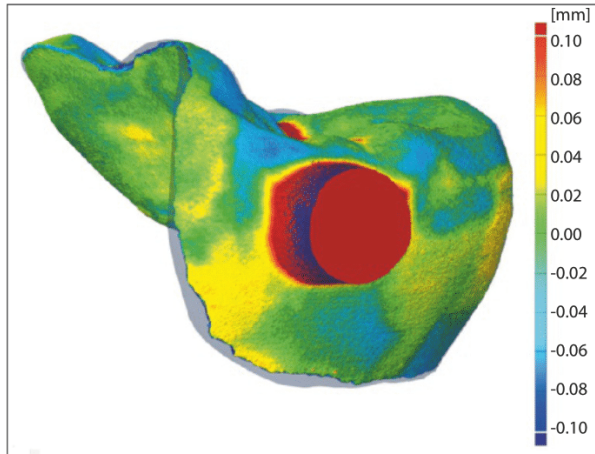
Fig 5 Marginal surface analysis of the superposition of the CAD model and the digitized prosthesis.
