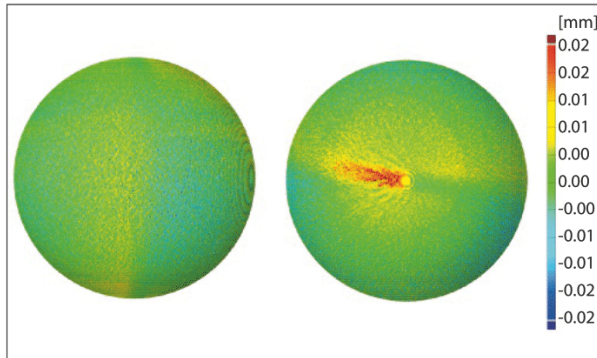
Fig 2 Form deviation map of the digitized ceramic ball.
