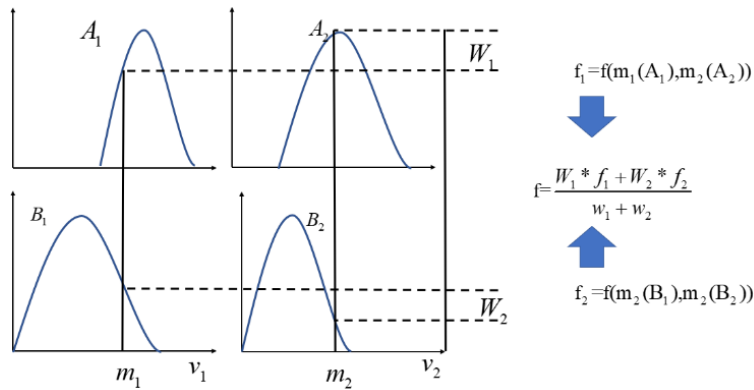
FIGURE 4.4 – Defuzzification de Takagi Segino
