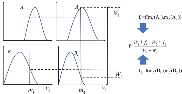
FIGURE 4.4 – Defuzzification de Takagi Segino
