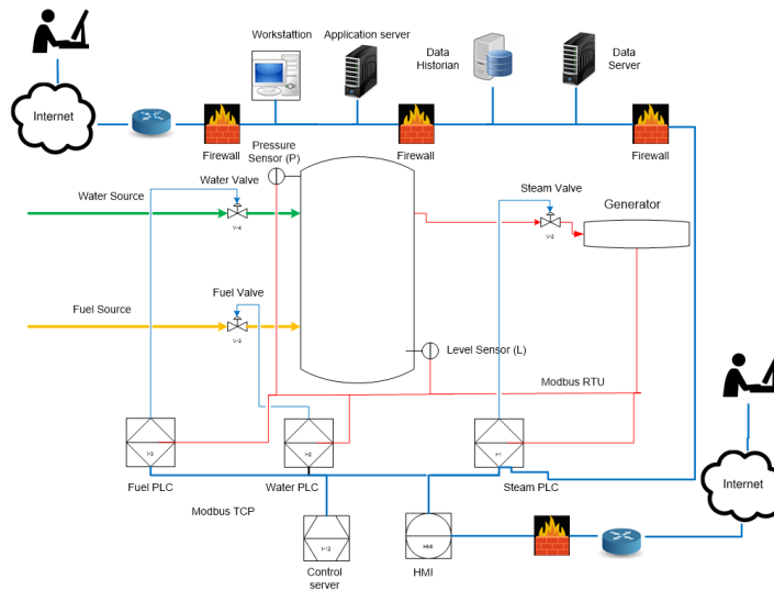
FIGURE 4.12 – Architecture 2 : The boiling water power plant without demilitarized zone (DMZ)
