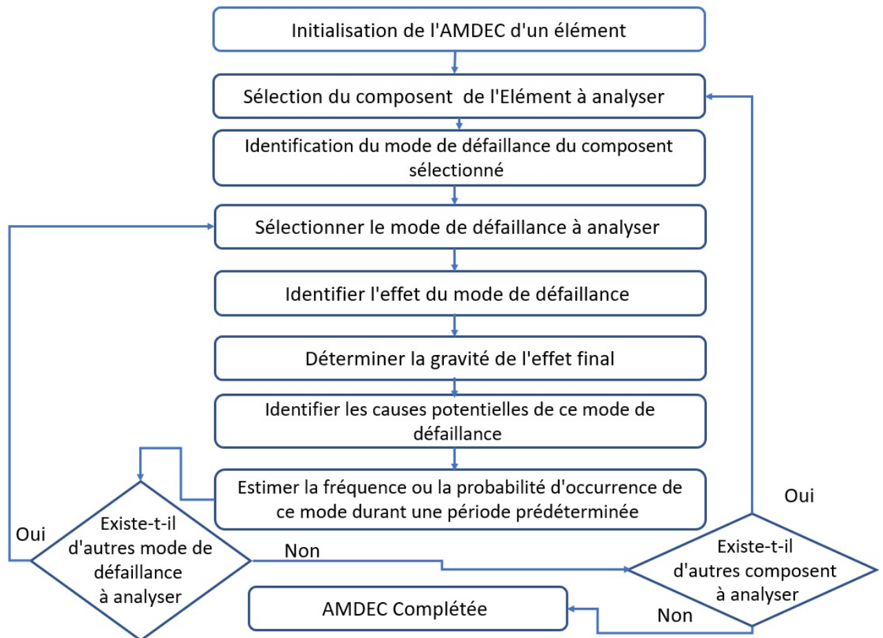
FIGURE 5.6 – AMDEC - diagramme d'analyse (Schmittner et al., 2014a)
