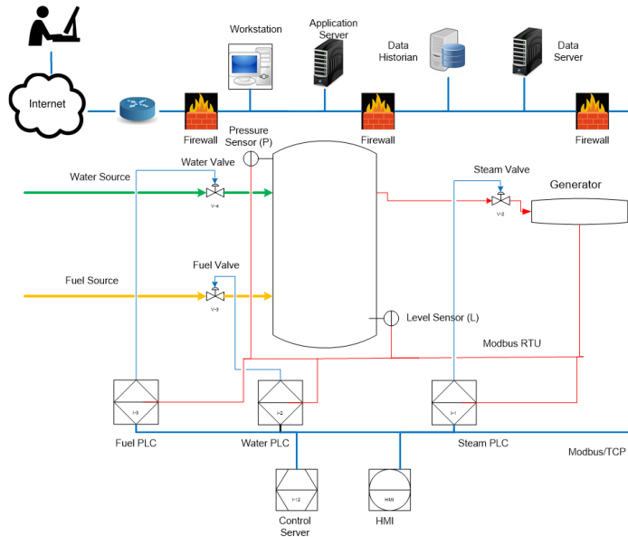
FIGURE 4.11 – Architecture 1 : The boiling water power plant with demilitarized zone (DMZ)
