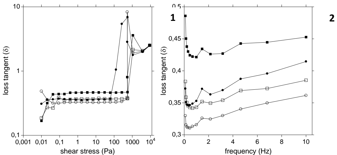
Figure 4. (1) Shear stress sweep of the four hydrogel samples. (2) Frequency sweep of the four hydrogel samples. Samples designation: Casein micelles without transglutaminase or jacoboticaba extract ( \square ), Casein micelles with transglutaminase but without jacoboticaba extract ( \circ ), Casein micelles without transglutaminase but with jacoboticaba extract ( \blacksquare ), Casein micelles with transglutaminase and jacoboticaba extract ( \bullet ).
