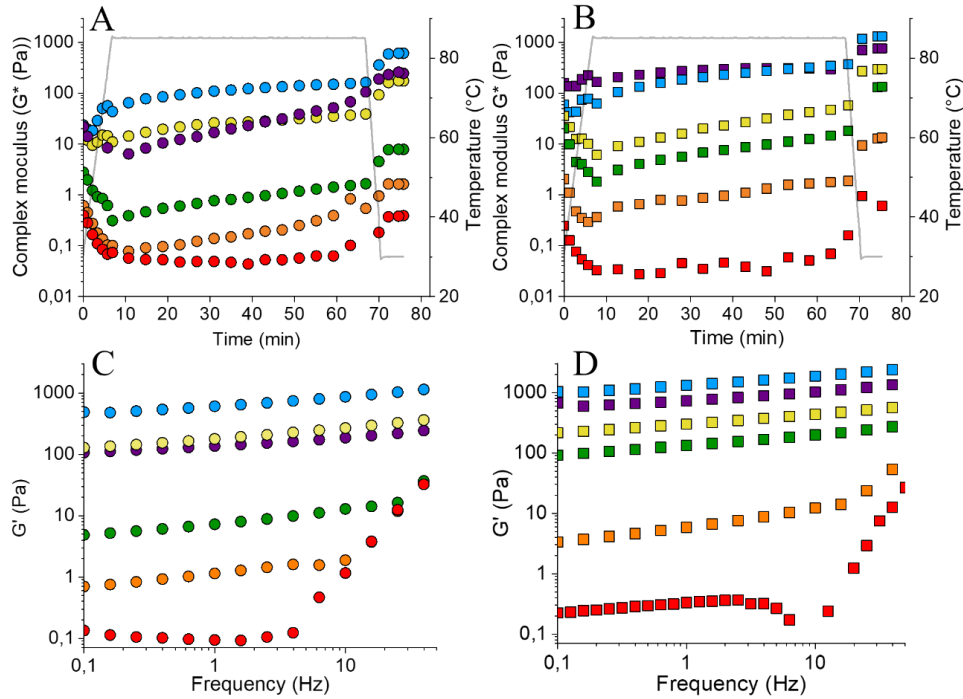
Figure 2. G^* as a function of thermal treatment for casein micelle: pea protein suspensions at 12 (○A) and 16% (□B). Frequency dependence of mixed casein micelle: pea protein suspensions at 12 (○C) and 16% (□D). CMs: pea protein ratios: (— red) 100:0; (— orange) 80:20; (— green) 60:40; (— yellow) 40:60; (— blue) 20:80; (— purple) 0:100.
