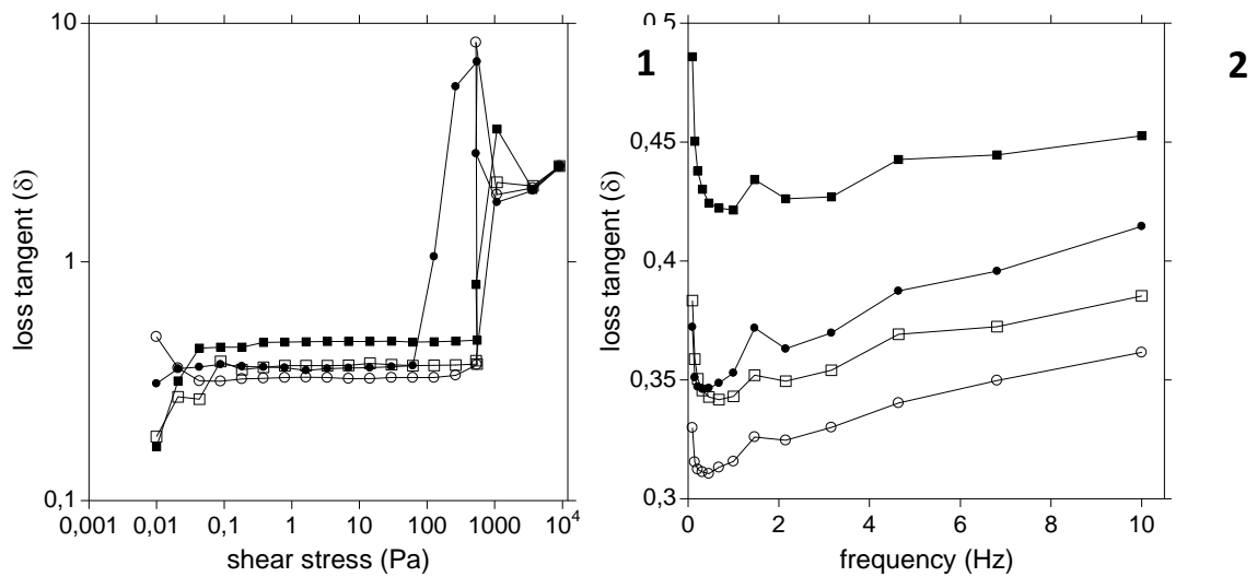
Figure 4. (1) Shear stress sweep of the four hydrogel samples. (2) Frequency sweep of the four hydrogel samples. Samples designation: Casein micelles without transglutaminase or jaboticaba extract (□), Casein micelles with transglutaminase but without jaboticaba extract (○), Casein micelles without transglutaminase but with jaboticaba extract (■), Casein micelles with transglutaminase and jaboticaba extract (●).
