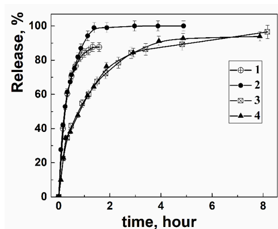
Figure 1. In vitro release of 2-PAM (1, 2) and 3-HPA (3, 4) using the dialysis bag method (n = 3). 1: 2-PAM-loaded SLNs; 2 and 4: 2-PAM+3-HPA-loaded SLNs; 3: 3-HPA-loaded SLNs. The concentration of 2-PAM and 3-HPA is 0.1% (w/w). Phosphate buffer, 0.025 M (1), methanol-phosphate buffer (50% v/v) (2, 3, 4), pH = 7.4, 37 °C.
