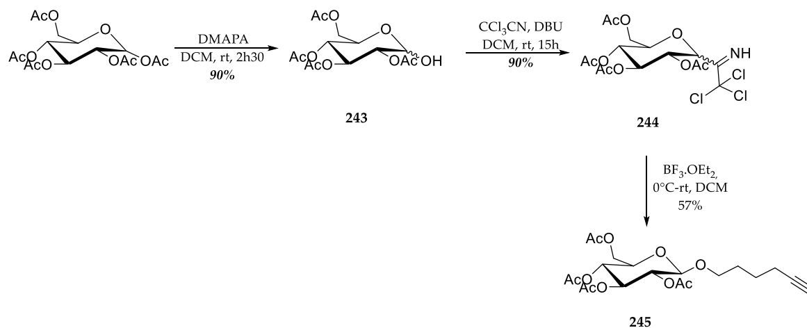
Figure 222. O-glycosylation testée
