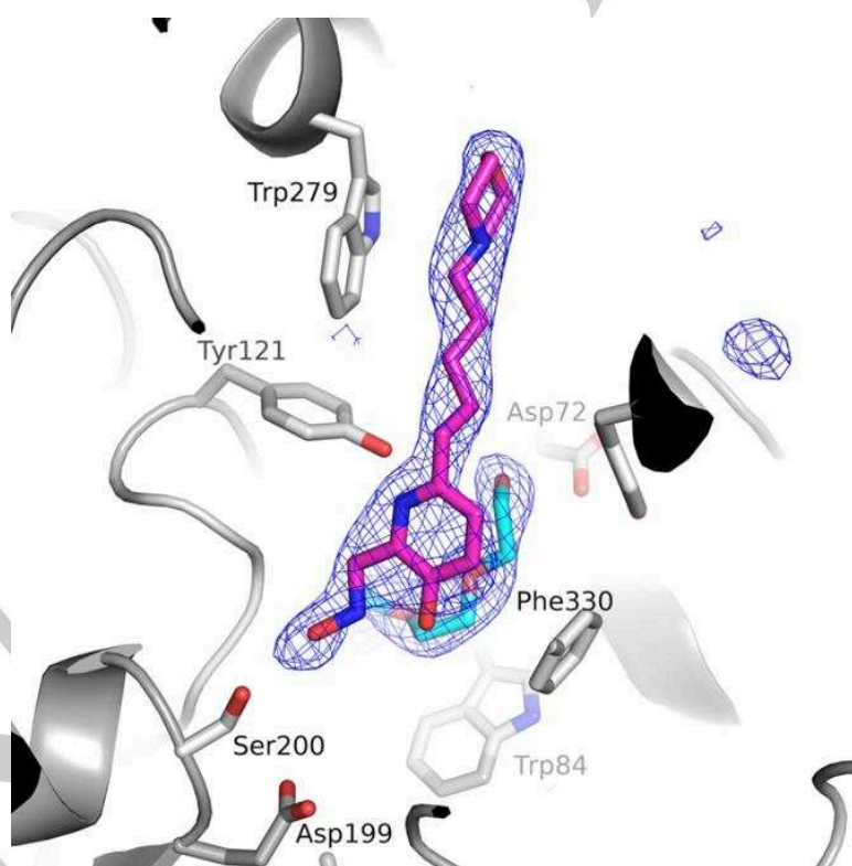
Figure 5. Crystal structure of the 17 /TcAChE complex. The oxime moiety is at 3.5 Å from Ser200Oy. The omit map Fo-Fc (blue mesh), shown around oxime 17 (magenta) and a PEG molecule (cyan) positioned between the oxime and Trp84 (not shown), is contoured at 3.5 \sigma .
