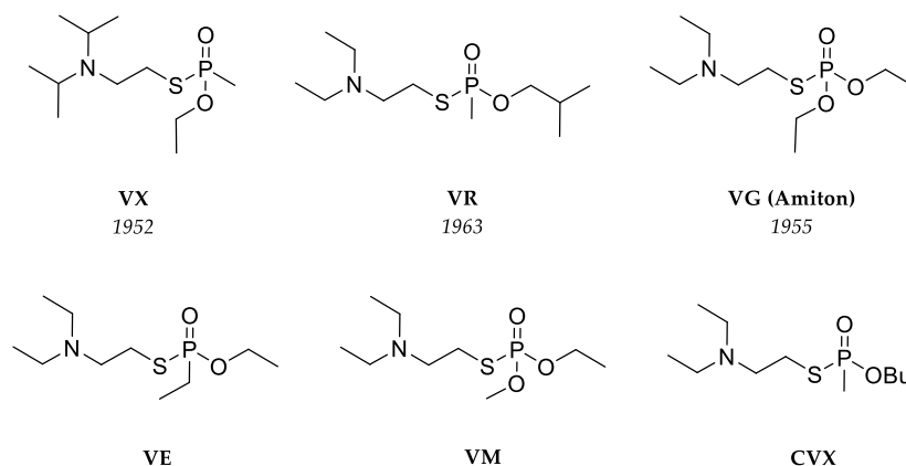
Figure 20. Structures des agents V
