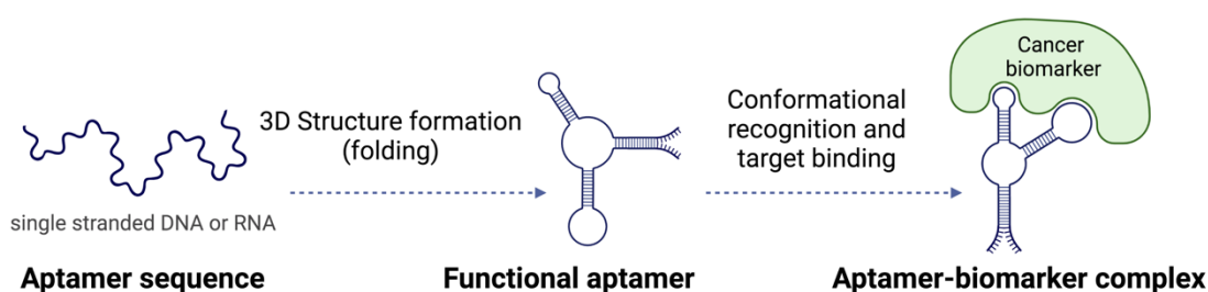
77 78 Figure 9. Aptamer structure and the conformational target binding.
