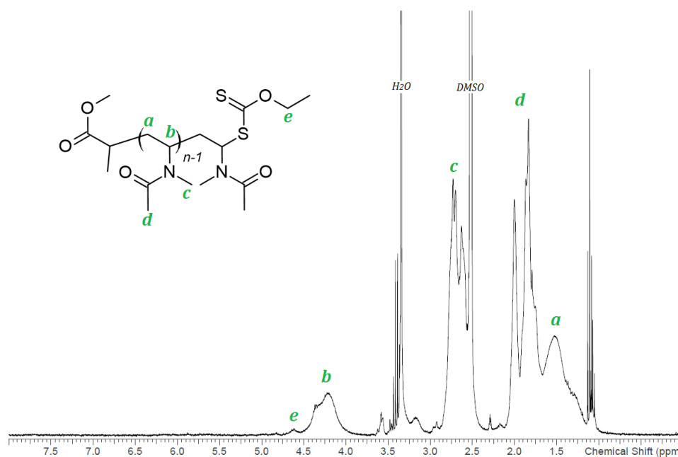
Figure 1-7. ^1\text{H} NMR spectrum of PNMVA-CTA1. M_{n,\text{SEC}} = 7000 \text{ g mol}^{-1} , D = 1.05 . Measured on a 300MHz apparatus.
