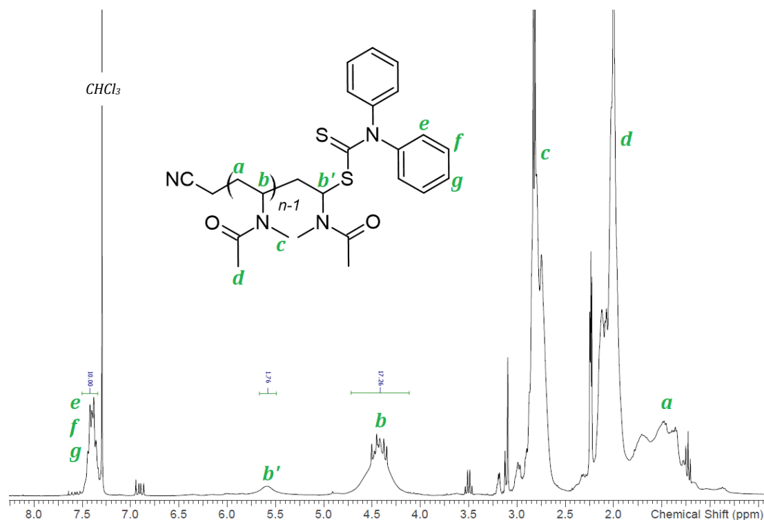
Figure 1-9. ^1\text{H} NMR spectrum of PNMVA-CTA4. M_{n\text{NMR}} = M_{\text{CTA4}} + \frac{10 \cdot (b+b')}{(e+f+g)} \times M_{\text{NMVA}} with M_{\text{CTA4}} = 284 \text{ g mol}^{-1} ; M_{\text{NMVA}} = 99 \text{ g mol}^{-1} . Measured on a 300MHz apparatus
