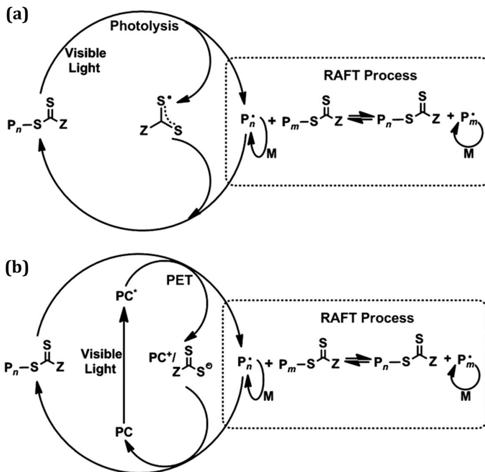
Scheme 3. General mechanism for RAFT polymerization initiated via (a) photodissociation of the CTA or (b) photoinduced electron transfer (PET-RAFT). PC: Photo-redox catalyst. Reprinted with permission from ref 73 . Copyright 2015 American Chemical Society.
