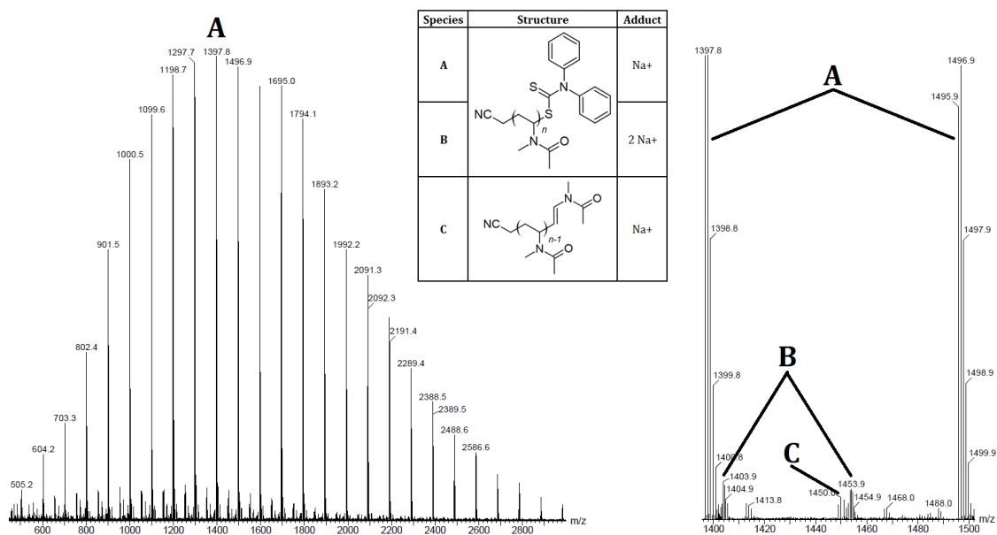
Figure 1-10. ESI-MS spectrum of PNMVA-CTA4.
