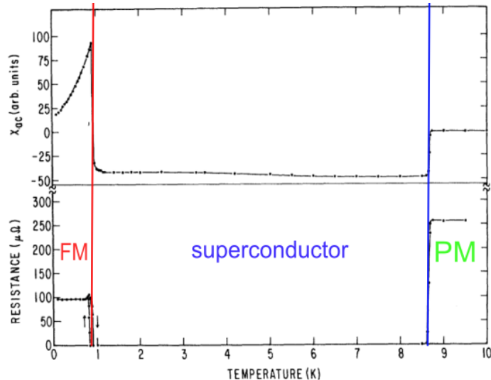
Fig. 1.1: Measurements performed on \text{ErRh}_4\text{B}_4 . Top: ac -susceptibility. Bottom: resistivity. Vertical lines has been added to separate the three different phases which are paramagnetic (PM), superconducting and ferromagnetic (FM). From ref [33].
