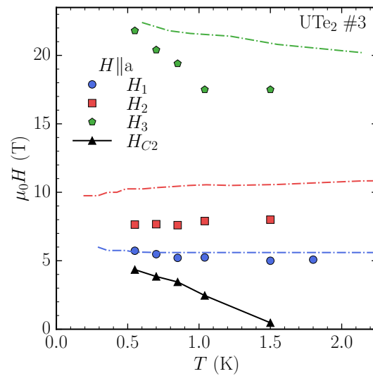
Fig. 3.9: Phase diagram obtained with the field sweeps H\parallel a . The dash-dotted lines correspond to the phase diagram from [104].
