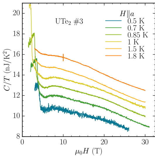
Fig. 3.8: Field sweeps H\parallel a done on sample #3. Curves have been shift of 1\text{ nJ/K}^2 from each other for clarity.
