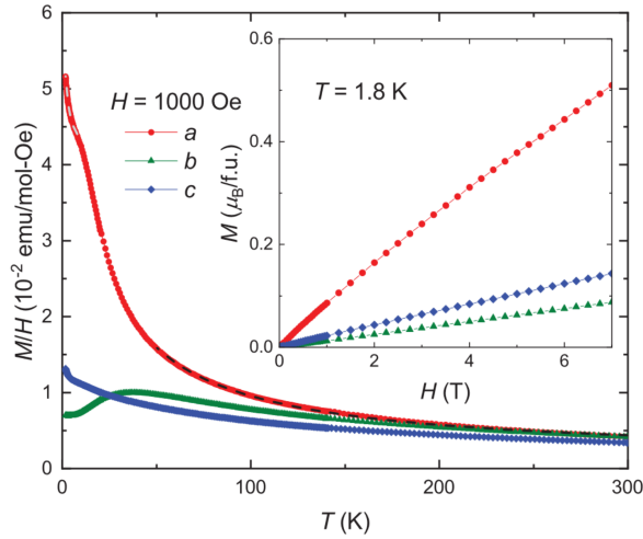
Fig. 1.23: M as a function of temperature for the three axes at 0.1 T. Inset: M as function of field at 1.8 K. Ref [113]
