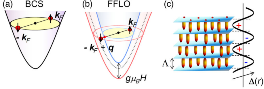
Fig. 1.10: (a) Schematic illustration of Cooper pairing [(-k_F)_\downarrow(k_F)_\uparrow] in the superconducting state and (b) [(-k_F + q)_\downarrow(k_F)_\uparrow] in the FFLO state. (c) Schematic illustration of the superconducting order parameter \Delta(r) in real space and the segmentation of magnetic flux lines by the nodal planes. From ref [64].
