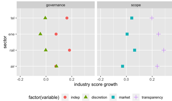
Figure 4.3: ANOVA evolution scores and residuals by sector
