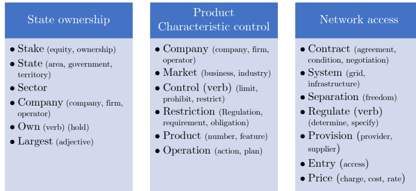
Figure 3.2: Descriptor distribution by dimension
