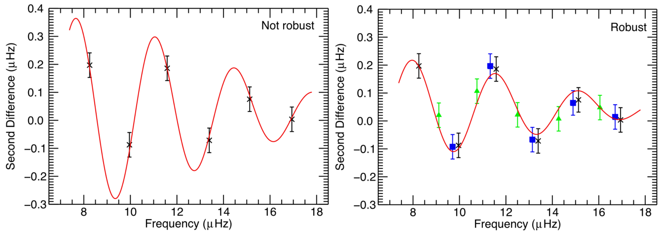
FIGURE 7.8: Fit of the glitch modulation in the second difference defined as \Delta_2\nu_{n,\ell} = \nu_{n+1,\ell} - 2\nu_{n,\ell} + \nu_{n-1,\ell} from a red-giant model with \nu_{\text{max}} = 12.71 \mu\text{Hz} , mass M = 1.5 M_{\odot} , initial helium mass fraction Y = 0.278 , and initial metal mass fraction Z = 0.020 . Radial, dipole and quadrupole modes are shown in black crosses, green triangle and blue squares, respectively. Left: only radial modes are used to fit the acoustic glitch modulation. Right: both radial, dipole and quadrupole modes are used to the acoustic glitch modulation. Credit: Broomhall et al. (2014)
