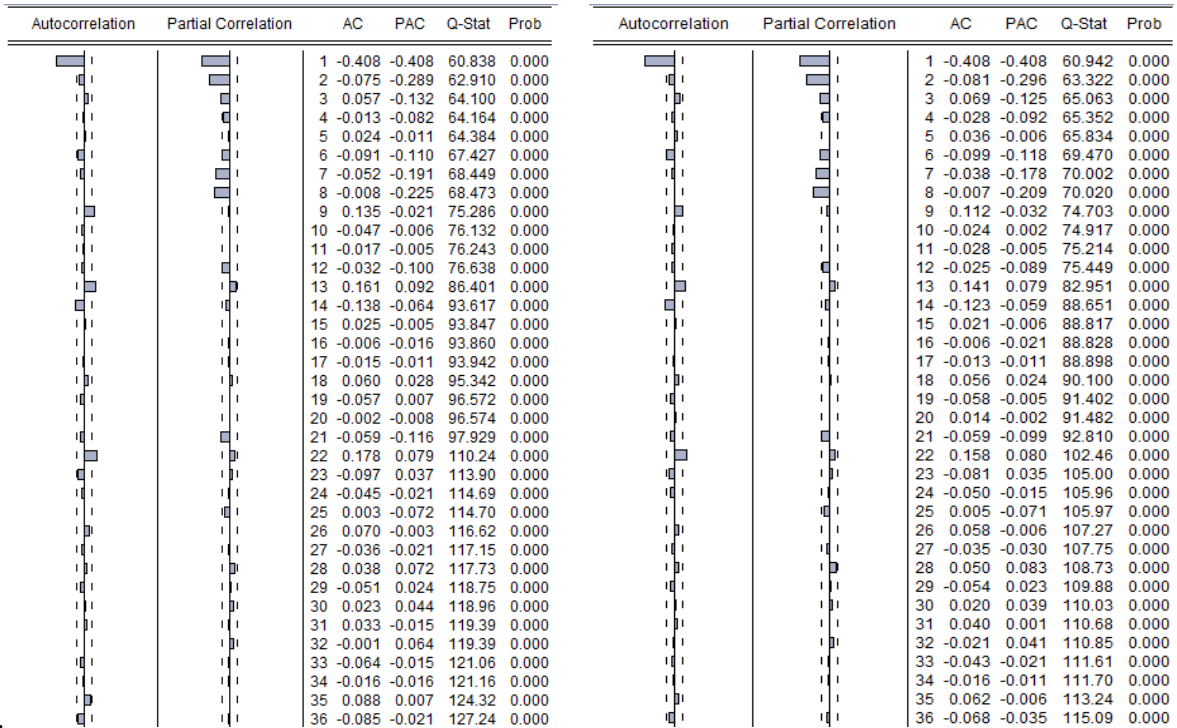
Figure 4.6 (a) POWER correlogram at first difference; (b) IRRA correlogram at first difference
