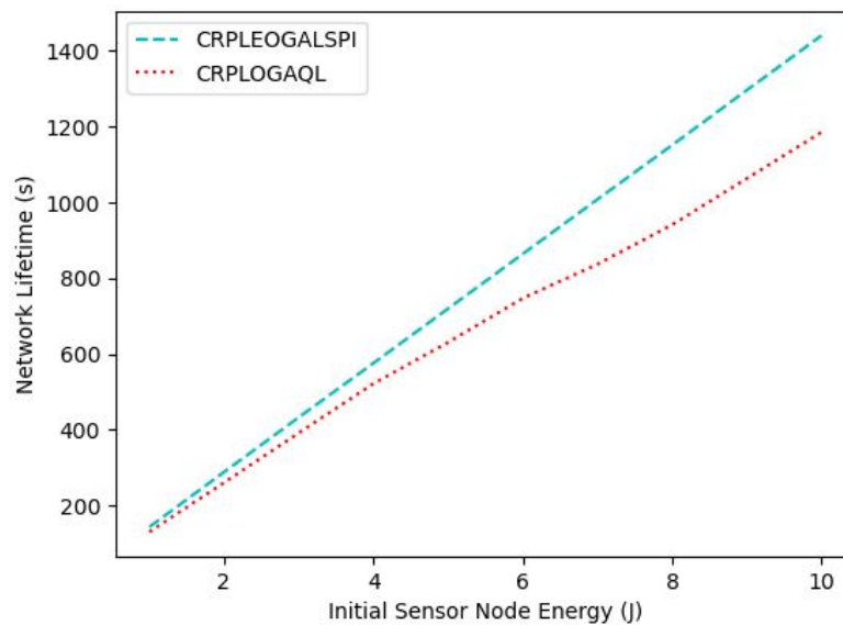
Figure 6.2: Network lifetime with Initial Node Energy.
