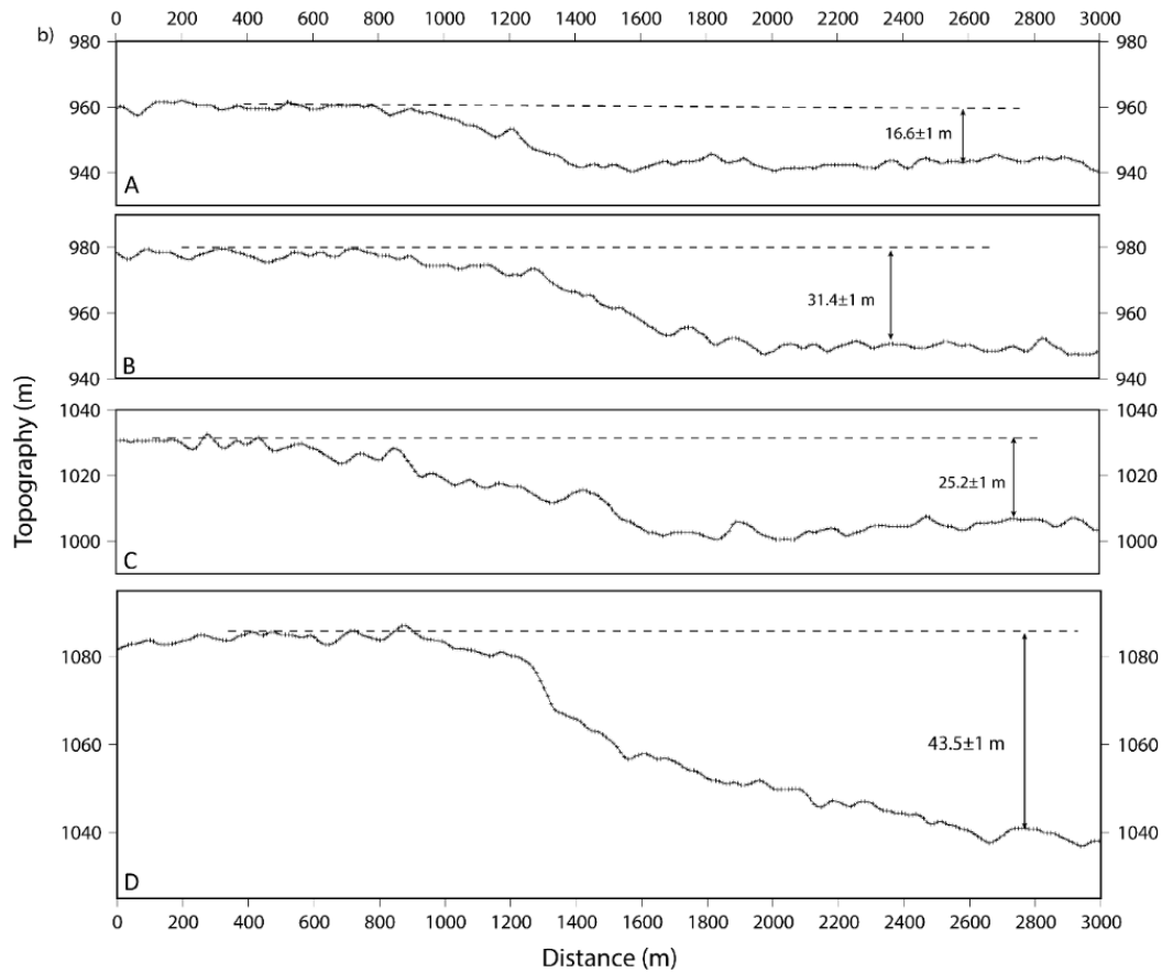
486 Figure 17. b) Khurutse fault scarp cross-sections with measured geomorphic offsets, in 487 meters.
