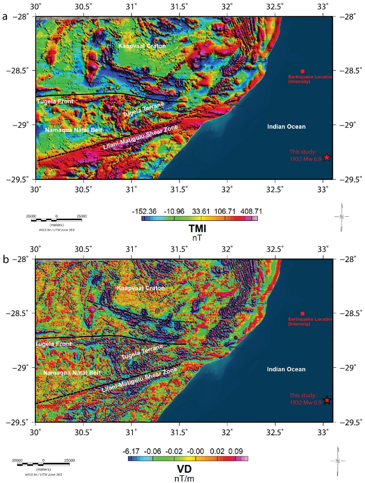
260 Figure 11: a) Interpreted total magnetic field with Tugela fault scarp as observed from 261 tectonic geomorphology and b) interpreted first vertical derivative image with Tugela and 262 Greytown fault scarps as observed from tectonic geomorphology.
