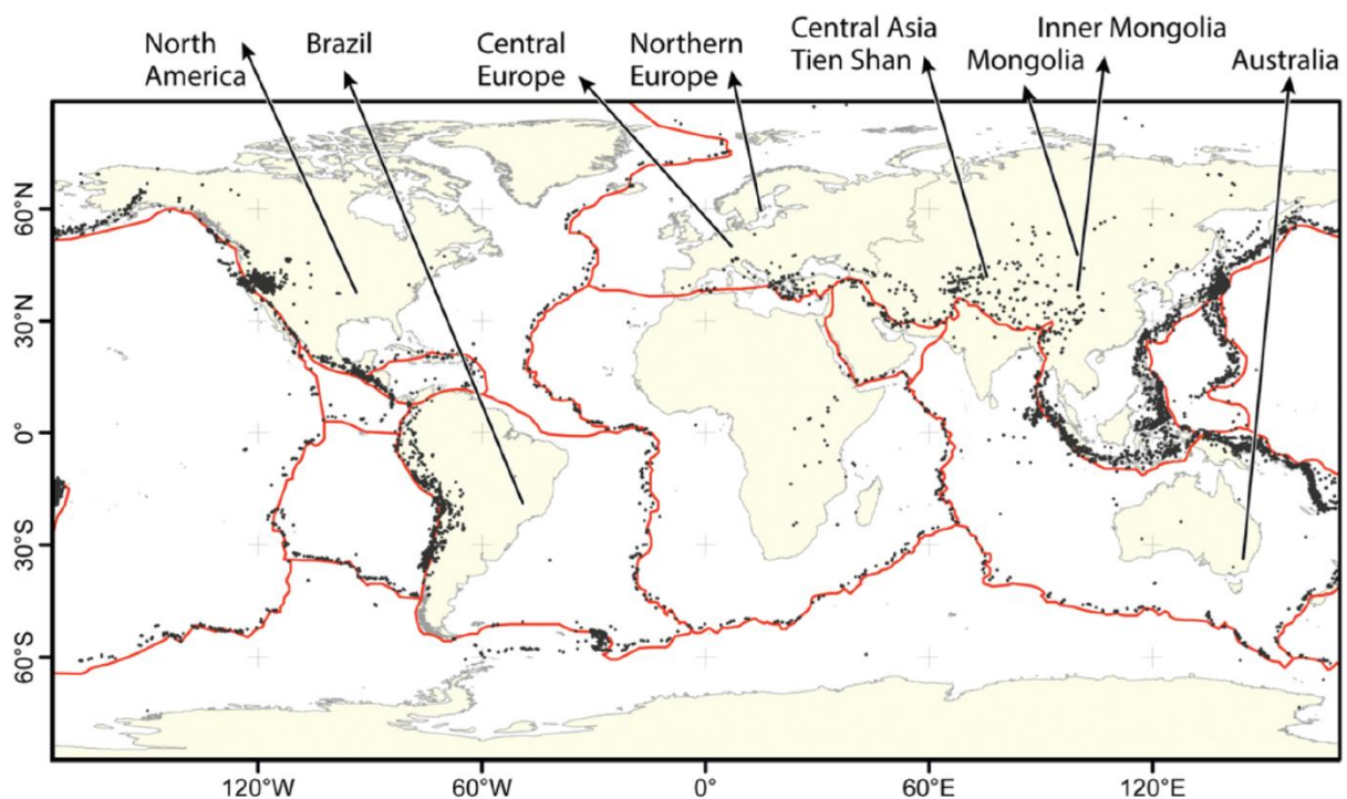
Figure 1. Intraplate earthquakes as indicated in Landgraf et al. (2017). Although several earthquakes have affected the intraplate regions (e.g., 1636, 1862, 1939 Ghana, 1809 South Africa; 1820 Congo-Angola; 1983 Guinea; 1932 South Africa, 1990 South Sudan), the African continent is not mentioned in this map.
