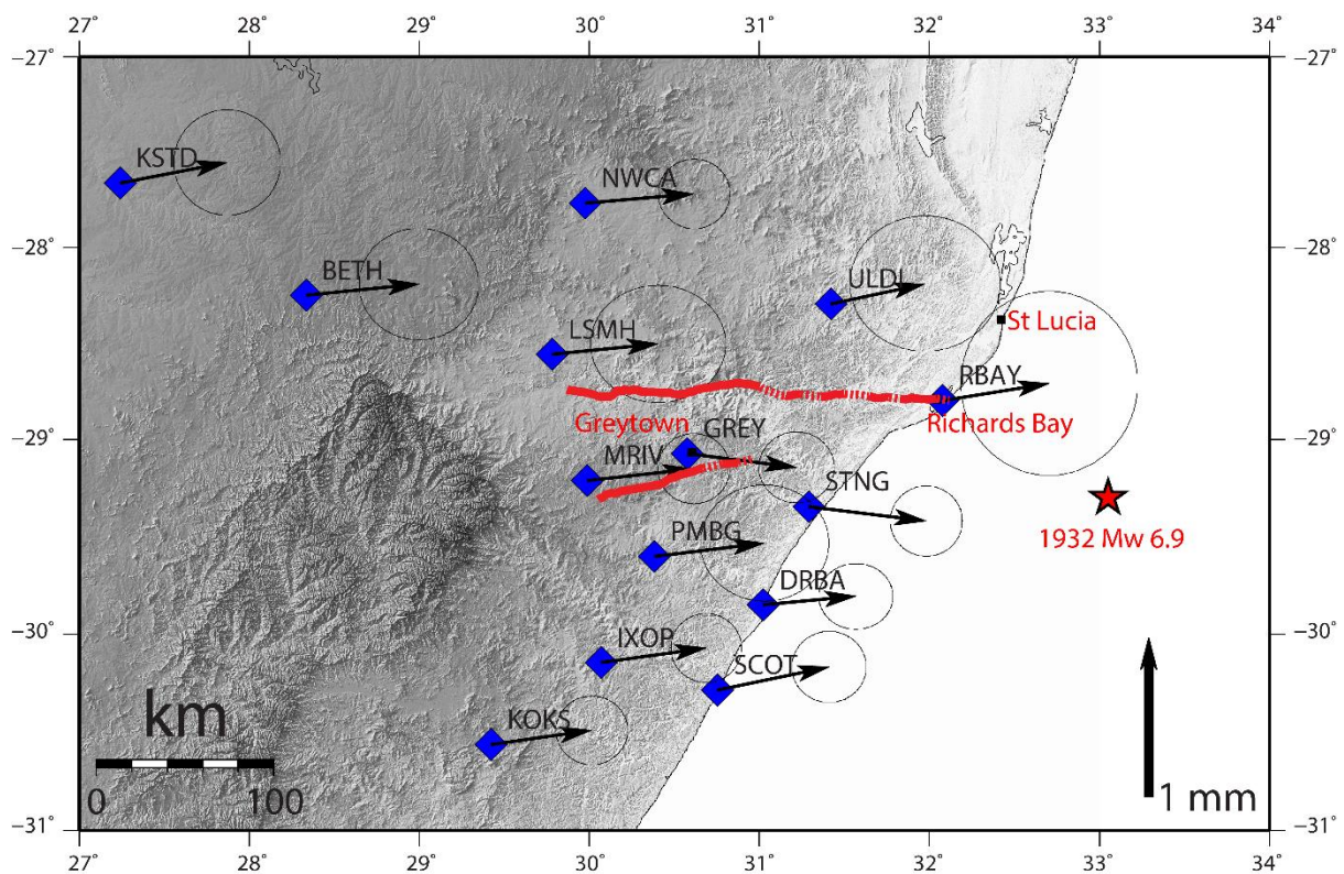
280 281 Figure 13: GPS velocities of stations in KwaZulu-Natal calculated using data from 282 http://geodesy.unr.edu/ . The ellipse errors are at 94.5 % confidence.
