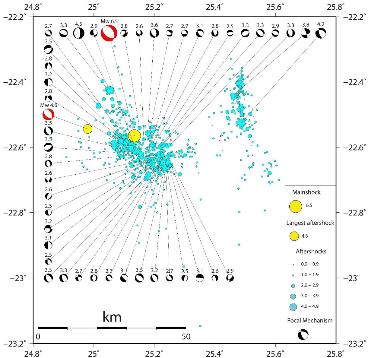
312 313 Figure 8. Focal mechanism solutions of 46 selected seismic events (see also Table SM4). 314 Solutions are Schmidt lower hemisphere, the numbers above the solutions give the local 315 magnitude. Aftershock locations are as in Fig. 5(a). Mechanism of mainshock (in red) is from 316 Harvard CMT ( https://www.globalcmt.org/CMTsearch.html ). 317
