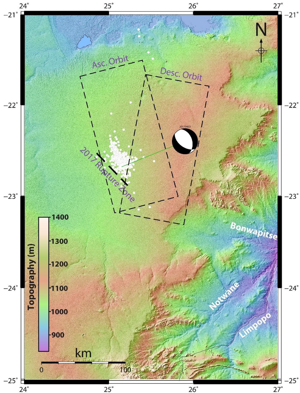
369 370 Figure 10. Frame of ascending and descending tracks of Sentinel-ESA-SAR images crossing 371 the 2017 earthquake area. We observe that only the ascending track covers the whole 2017 372 earthquake area. Thick dashed line is the inferred 2017 Moyabana earthquake rupture zone 373 and small white circles show aftershock distribution. Focal mechanism of mainshock is from 374 Harvard CMT. Background topography is from SRTM1’. 375
