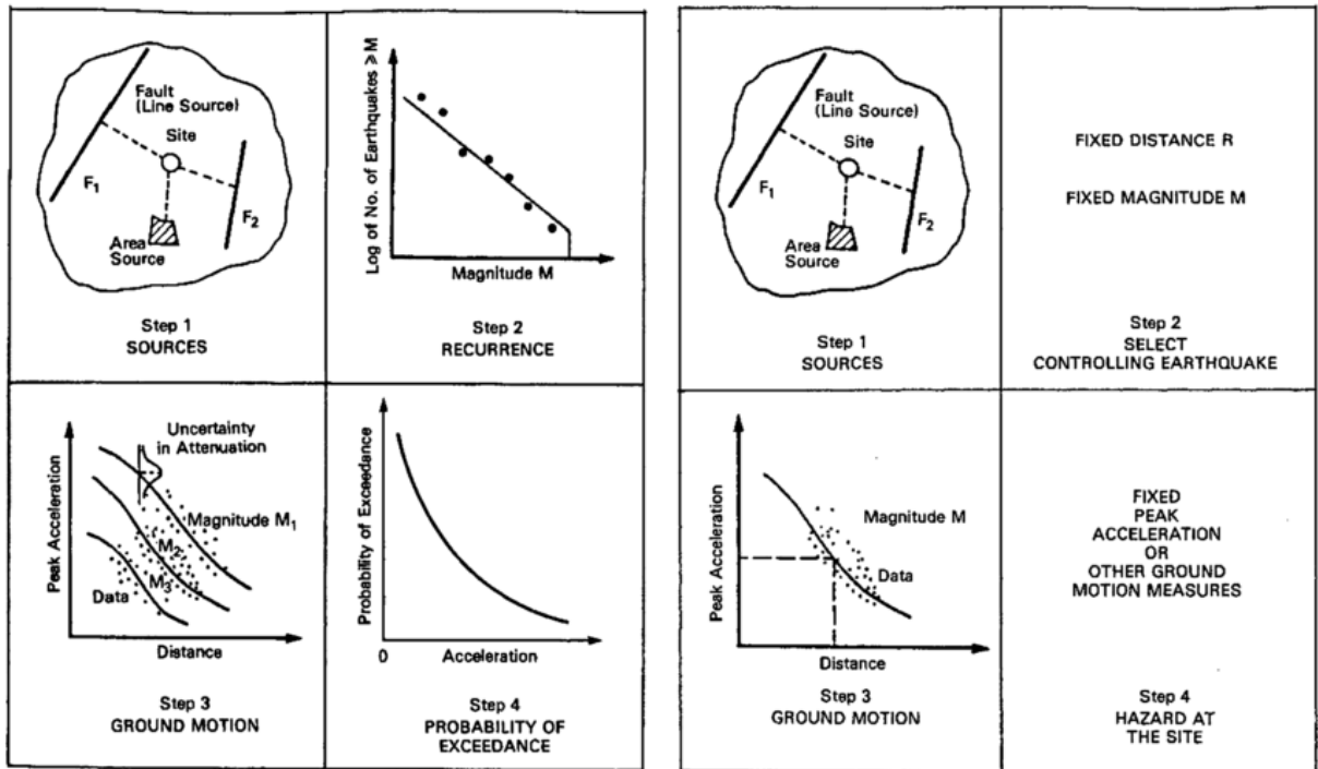
Figure 5. Probabilistic and Deterministic seismic hazard assessment as described by Reiter (1991)
