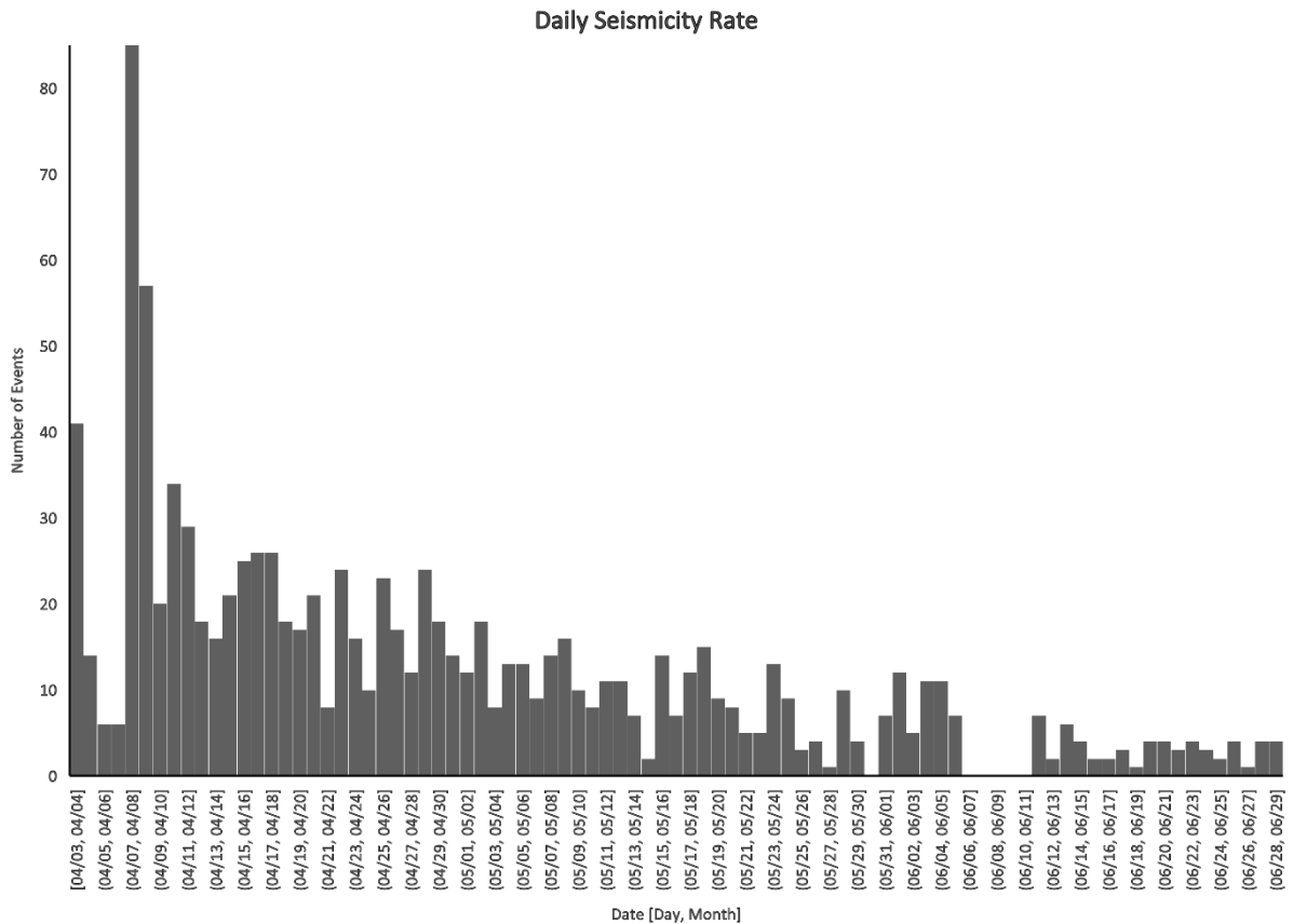
206 207 Figure 4. Daily number of seismicity recorded from the 3 rd of April to the 29 th of June 208 2017.
