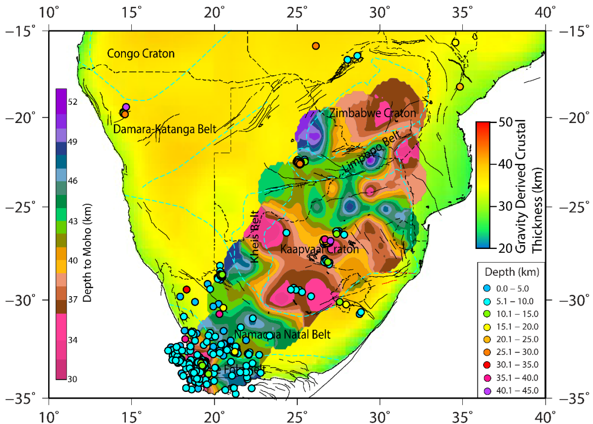
Figure 4. The depth to Moho (Youssof et al., 2013) and gravity derived crustal thickness (Tugume et al., 2013) with earthquake depths in southern Africa.
