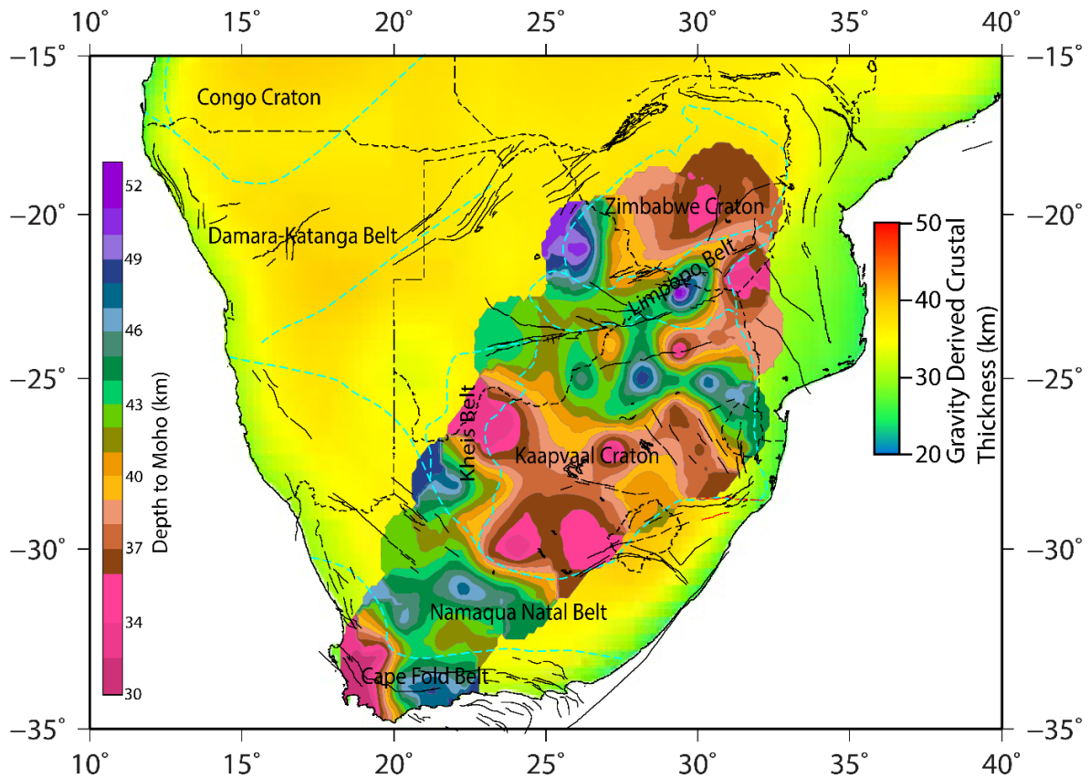
Figure 2. Depth to Moho (Youssof et al., 2013) and gravity derived crustal thickness (Tugume et al., 2013).
