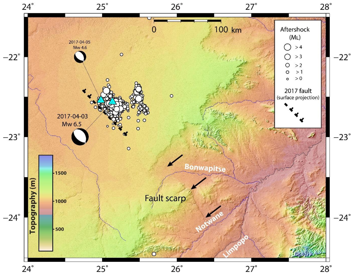
454 Figure 15: Identification of the Khurutse cumulative fault scarp (black arrows) southeast of 455 the 2017 earthquake rupture indicated using a dashed line located from the projection of 456 InSAR rupture (see Fig. 11). Also shown are the focal mechanisms of the mainshock and 457 largest aftershock as presented in Tables 1 and SM4. Details of Khurutse fault scarp 458 morphology are in landscape photos of Fig. 16 and map of Fig 17a. Background topography 459 is from Shuttle Radar Topography Mission (SRTM) 1" data.
