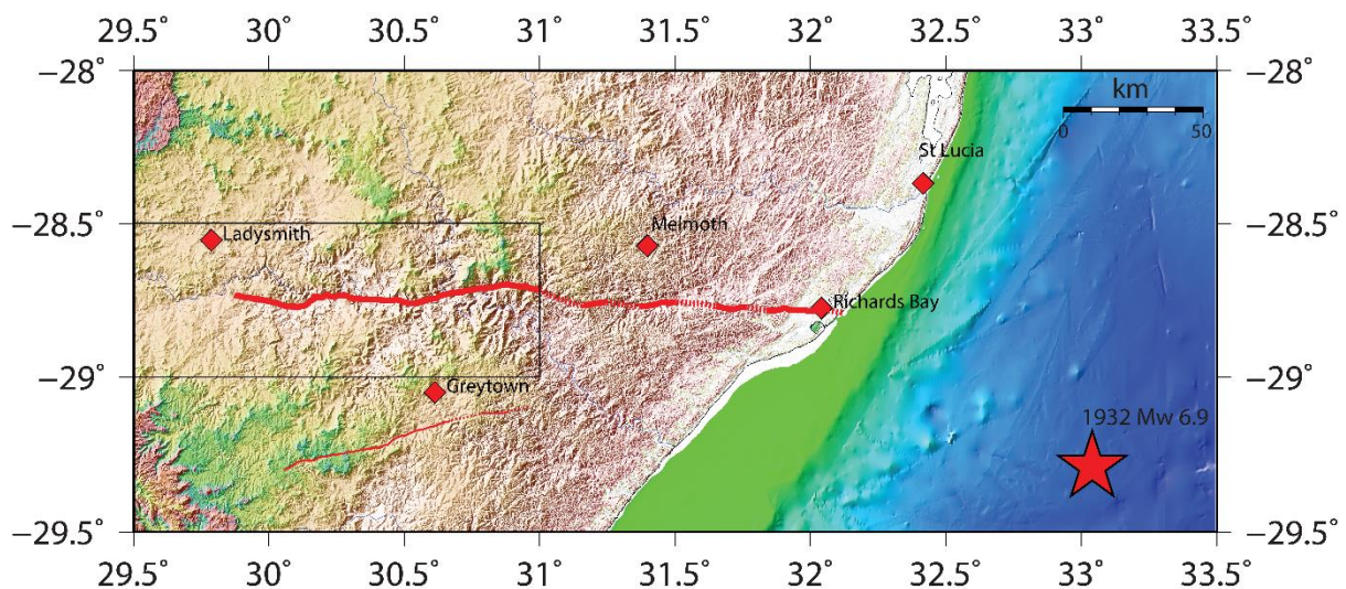
185 Figure 5: Tugela fault scarp highlighted with by a thick red line at areas where it is clearly 186 visible, the red star shows the epicentre of the 1932 M_w 6.9 St Lucia earthquake (ISC Bulletin). 187 The inset black block is the zoom in shown in Figure 4a.
