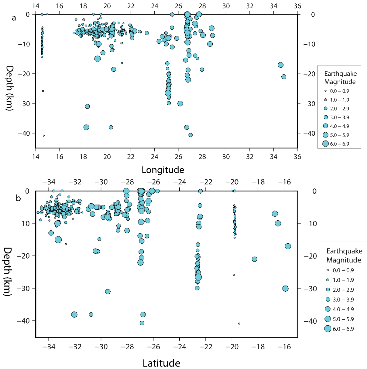
Figure 3. Earthquake depth values in southern Africa: a) EW cross section and b) NS cross section.
