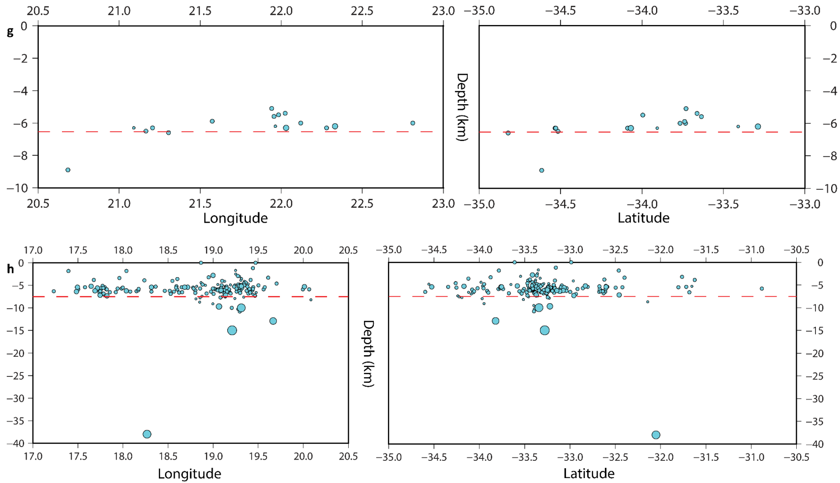
Figure 5. Seismogenic layer assessed using D90 of events located at a) NW Damara-Katanga Belt, b) west Limpopo belt, c) central Kaapvaal Craton, d) south Kaapvaal Craton, e) NW Namaqua-Natal belt, f) SW Namaqua-Natal belt, g) east Cape Fold Belt and h) west Cape Fold Belt. The layer thickness value is marked by the red broken line.
