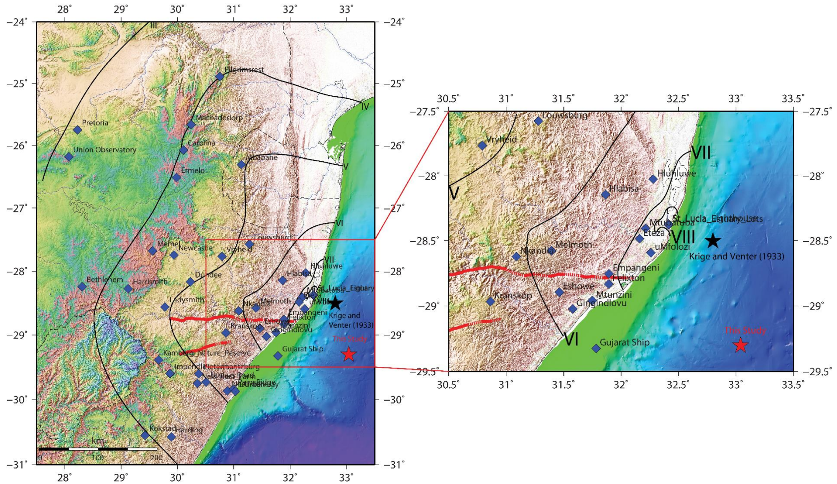
168 Figure 4: Intensity data (MMI31) of the 1932 Mw 6.9 St Lucia from Krige and Venter (1933), KwaZulu-Natal with a zoom into the area near the 169 epicentre (from Krige and Venter (1933), black star) with highest reported intensity. The red star shows the epicentre location of the 1932 Mw 6.9 170 St Lucia earthquake from this study.
