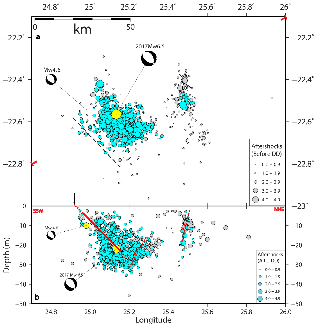
SM3: Spatial distribution of aftershock locations before and after DD relocation.
