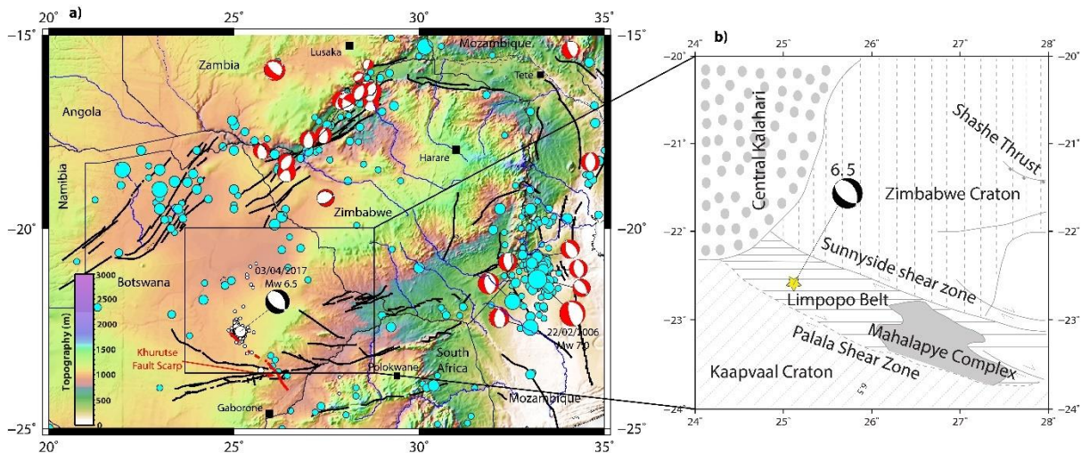
147 148 Figure 2. a) Seismotectonic framework excerpt of the Seismotectonic Map of Africa (modified from 149 Meghraoui et al., 2016) with focal mechanism (CMT-Harvard) of the 2017 Moiyabana mainshock.
