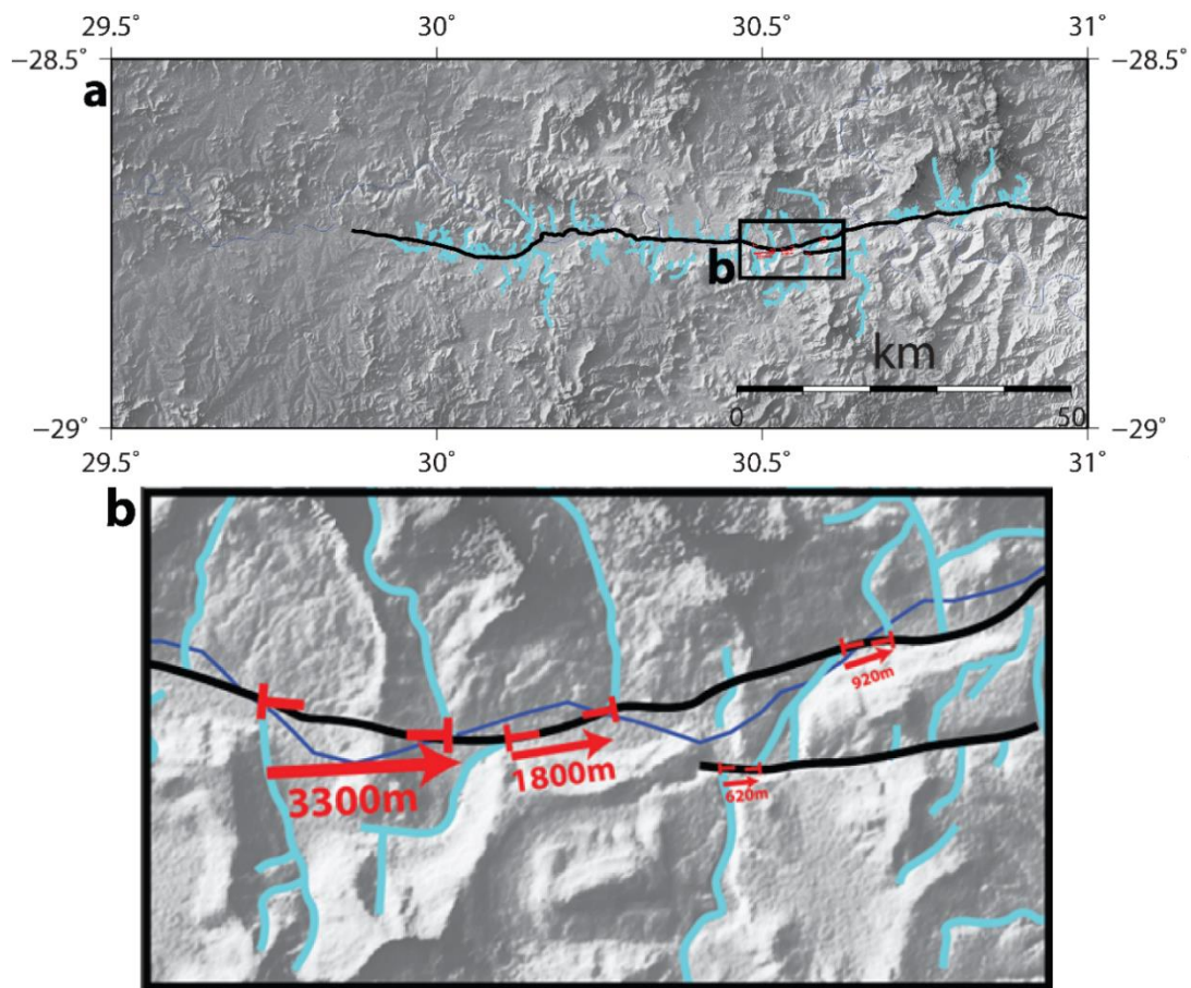
195 Figure 6: The right lateral movement (red arrows) on the western branch of the Tugela fault 196 scarp, traced from SRTM1" (Farr et al., 2007). The red T shows the beginning and end of the 197 right lateral movement of streams along the fault line with measurements in red text. The black 198 line traces the Tugela fault scarp and blue lines stream terraces which are crosscut by the fault. 199 Fault offsets are reported in Table 1.
