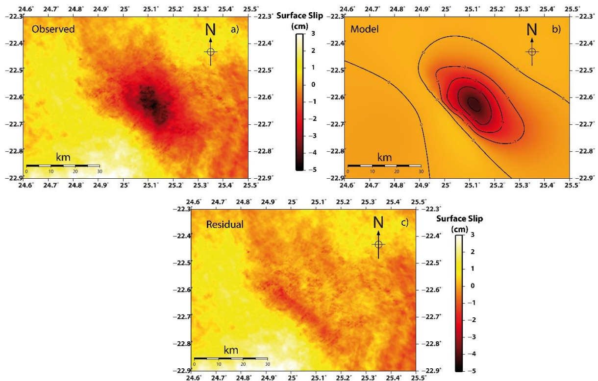
408 Figure 12 a) Unwrapped SAR data interferogram with surface slip distribution. b) Modelling 409 of surface deformation from the inversion of InSAR data. c) Residual of InSAR results versus 410 model.
