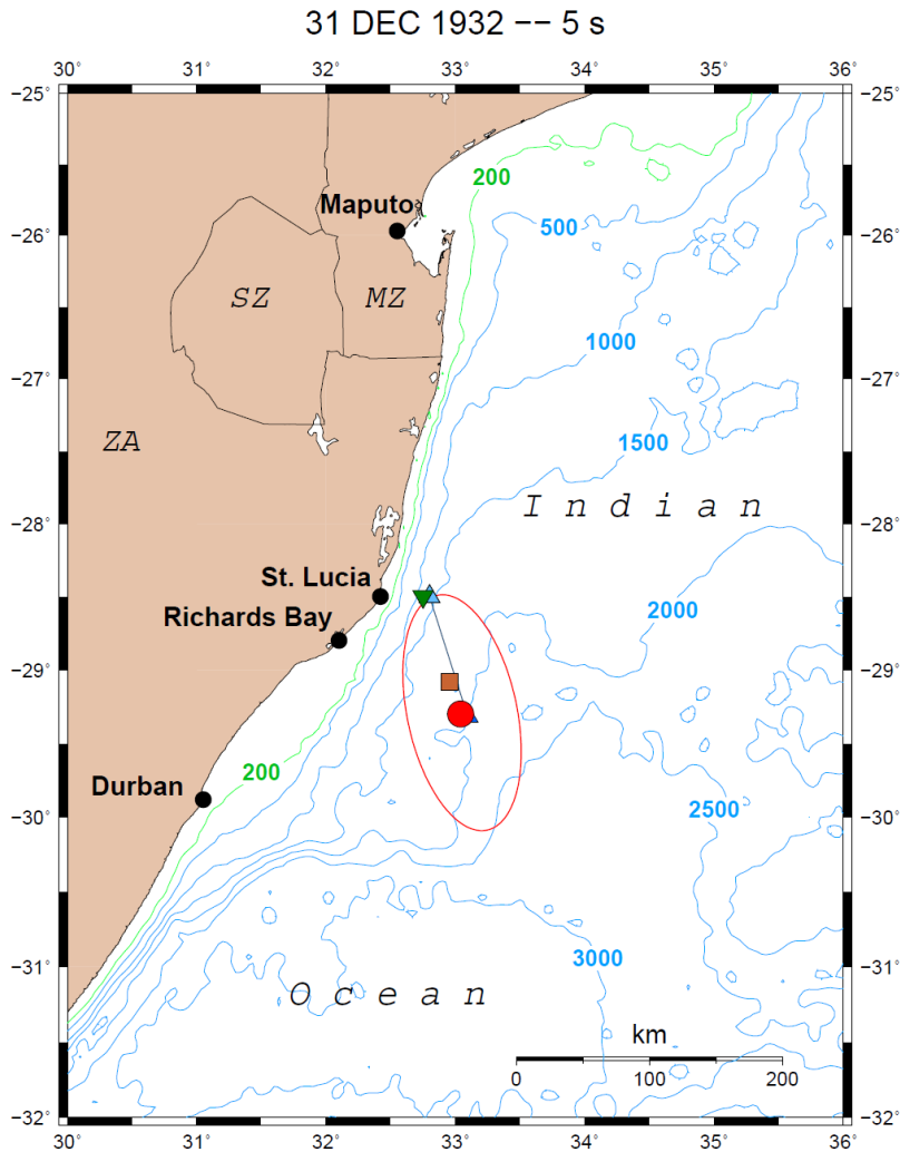
157 Figure 3. Relocations of the 1932 event: Red dot with ellipse: This study; Light blue triangle: 158 Gutenberg and Richter (1954); Brown square: Centennial Catalogue (Engdahl and Villasenor, 159 2002). Isobaths in meters.
