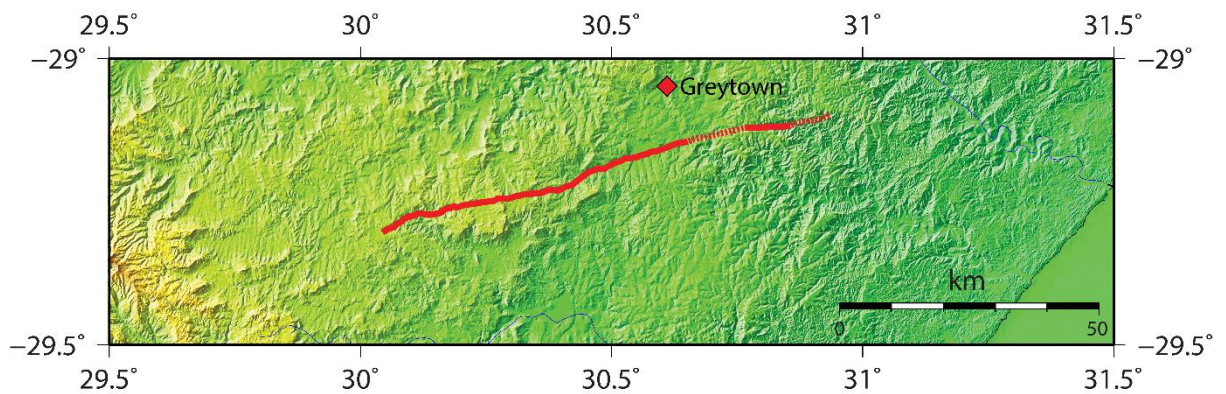
212 Figure 7: Greytown fault scarp, highlighted with a red line at areas where it is clearly visible.
