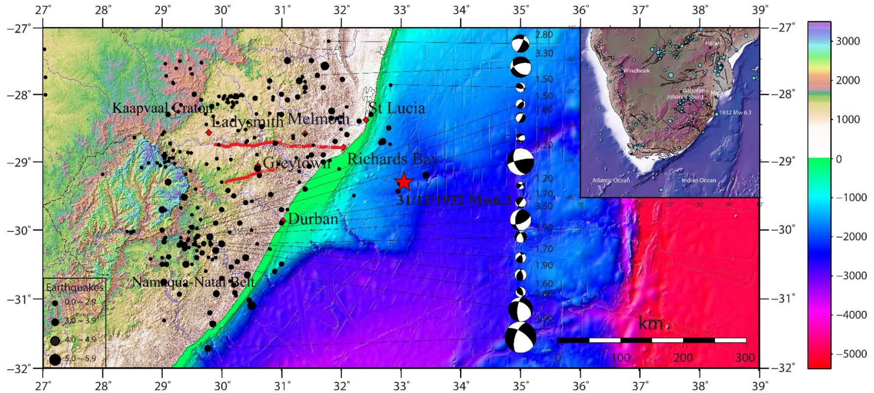
111 Figure 1: Tectonic Framework of KwaZulu-Natal showing Kaapvaal Craton and Namaqua-Natal Mobile Belt. Tugela and Greytown fault scarps 112 are shown in red lines traced from SRTM1 (Farr et al., 2007), earthquakes in black circles with focal mechanism solutions from the South African 113 National Seismic Network (SANSN) and offshore bathymetry from GEBCO Gridded Bathymetry Data Downloaded from 114 https://download.gebco.net/ . The red star shows this study's relocated epicentre of the 1932 Mw 6.9 St Lucia, KwaZulu-Natal. The southern 115 African map inset shows seismicity in cyan circles and the 1932 Mw 6.9 St Lucia, KwaZulu-Natal, is labelled in white text.
