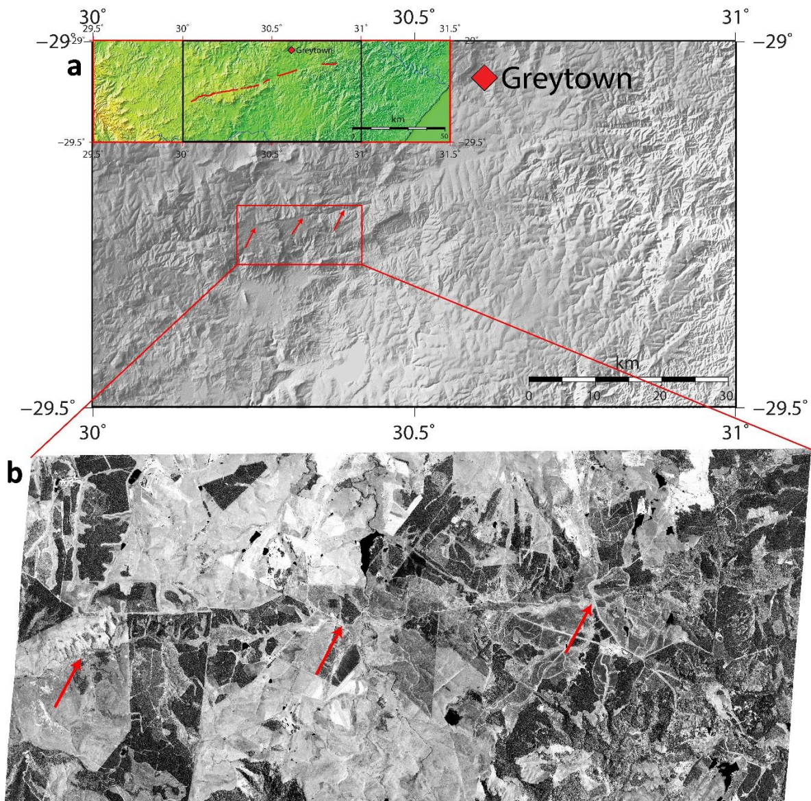
Figure 9: a) A zoomed section of the western branch of the Greytown fault scarp; b) Pleiades stereo image of western branch Greytown fault scarp; the red arrows show fault scarp visible on both a) SRTM1" and b) Pleiades stereo image.
