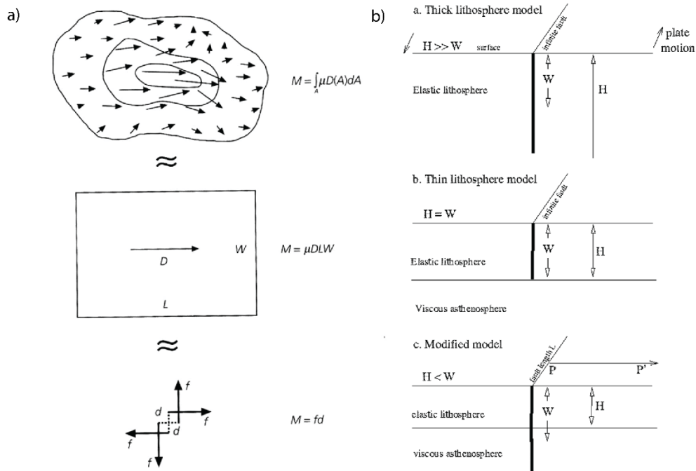
Figure 3. a) Physical parameters of an earthquake dislocation (Stein and Wysession, 2009). b) Three seismic cycle models for different elastic thicknesses (Chery et al., 2001).
