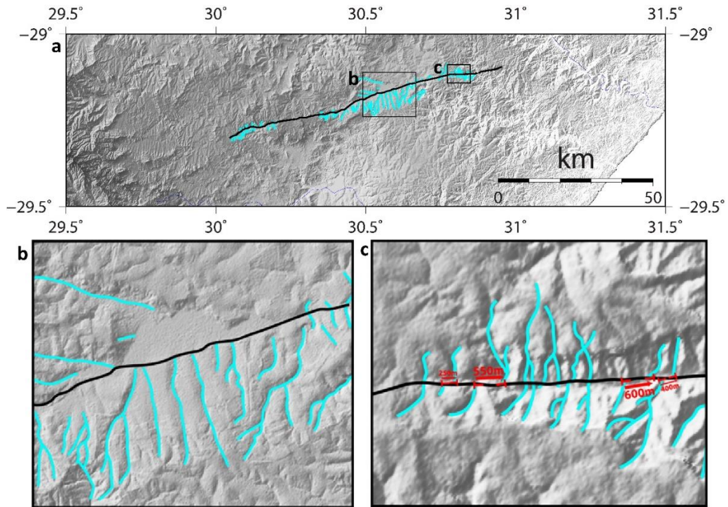
217 Figure 8: a) Terraces crosscut by the Greytown fault with detailed observations in boxes b and 218 c obtained from SRTM 1'' data; b) Quaternary basin limited on its southern edge by the fault, 219 and right lateral offset of streams located to the east; c) The fault crossing the dense 220 hydrographic system. Fault offsets are reported in Table 2.
