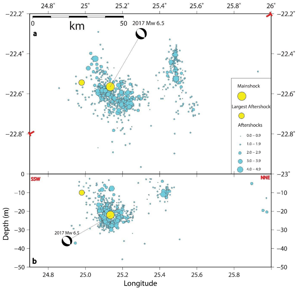
236 Figure 5. a) Mainshock and the initial aftershocks sequence location of the 2017 Moiyabana 237 earthquake with CMT-Harvard focal mechanism. b) Cross-section of the 2017 seismic 238 sequence, as indicated by the T-symbols in Fig. 5(a), recorded by temporary network from 8 239 April to 29 June 2017 (cyan circles) following the mainshock.
