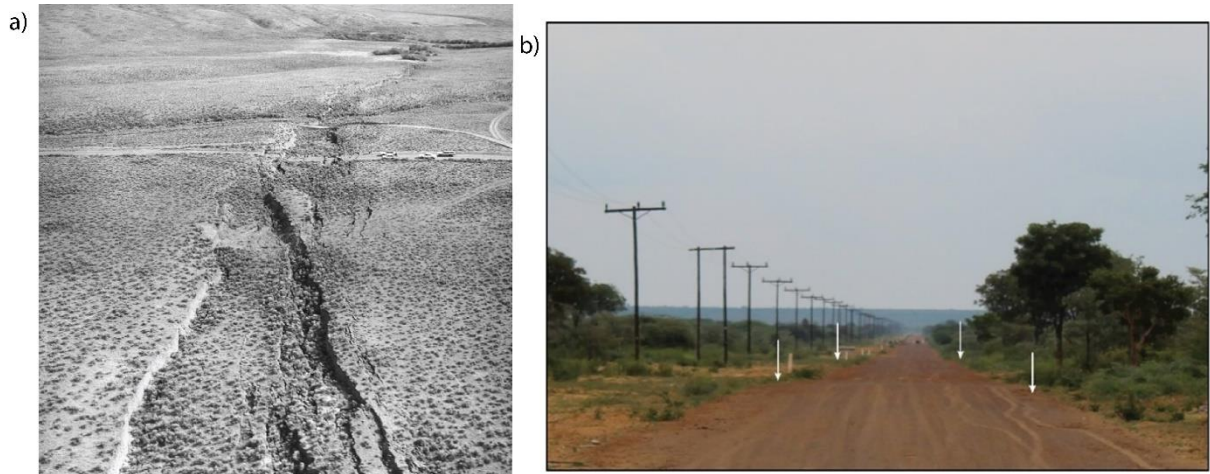
Figure 2. a) Surface faulting of 1983 Borah Peak earthquake in Basin and Range, Colorado (Crone et al., 1987). b) Escarpment of the Khurutse fault, located SE of the 2017 Moiyabana Earthquake (Mulabisana et al., 2021).
