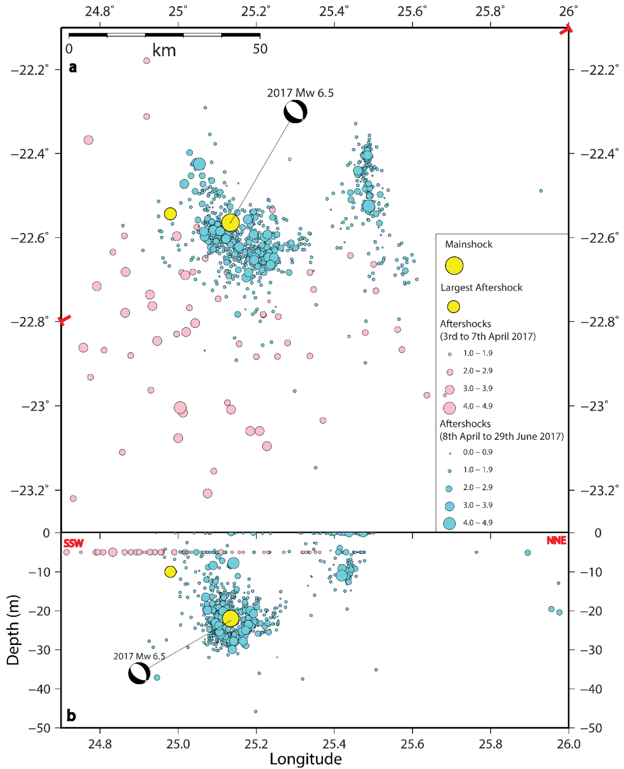
SM2: Spatial distribution and cross section of aftershock locations before and after the 8th of April 2017 (installation of temporary network).
