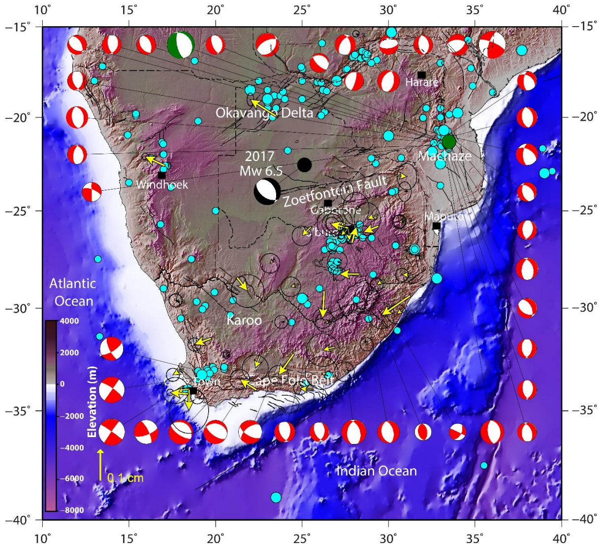
100 Figure 1: Seismotectonic background of southern Africa (light blue circles and red and white 101 CMT focal mechanism solutions (SM1)), as updated from Meghraoui et al., (2016). Black 102 circle is the location of the 3 April 2017 earthquake and its focal mechanism solution (black 103 and white, CMT-Harvard, https://www.globalcmt.org/CMTsearch.html ). 104 The green and white focal mechanism is of the 23 February 2006 Machaze earthquake (Mw 7.0, Mozambique, 105 green circle). GPS velocities (Nubia fixed, yellow arrow with 1\sigma error ellipse) are from Saria 106 et al. (2014).
