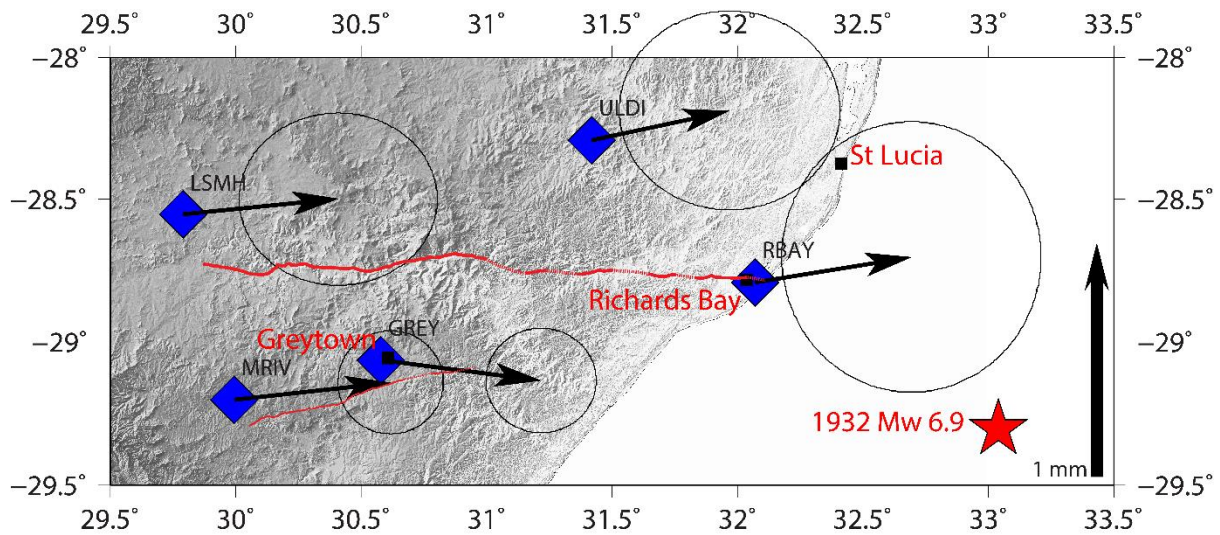
293 Figure 14. Focus on GPS velocities of stations around the Tugela fault scarp
