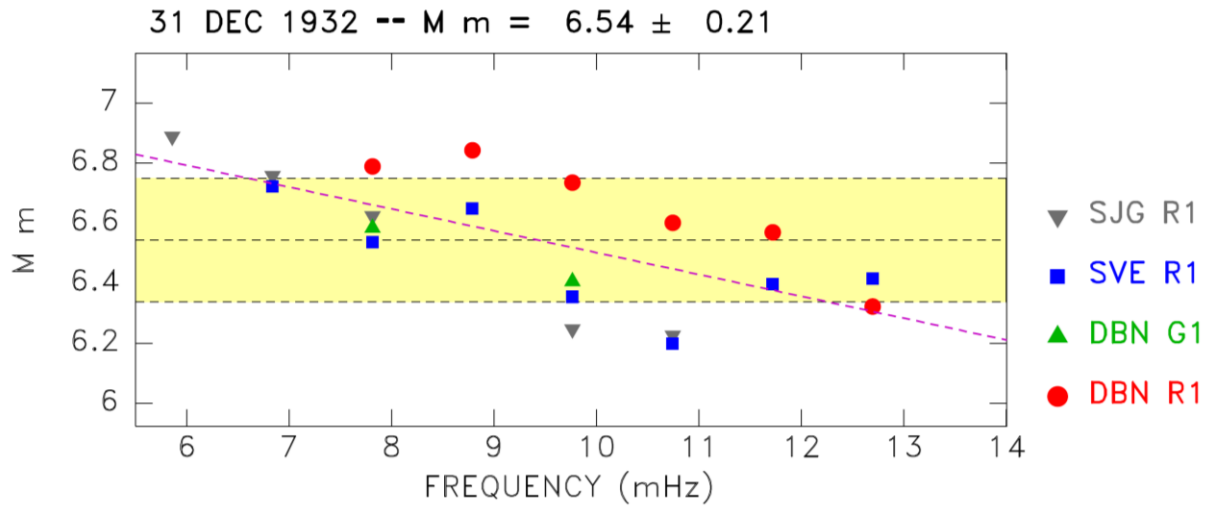
153 154 Figure 2. Mantle magnitude M_m = \log_{10}M_0 - 20 (Okal and Talandier, 1989), as a function of 155 frequency.
