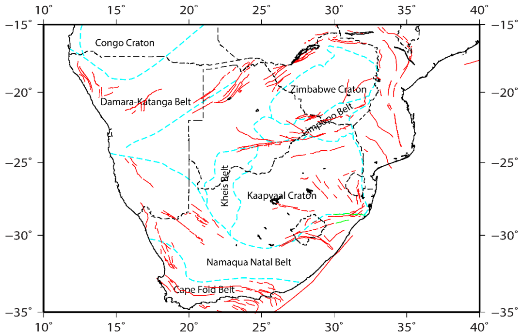
Figure 1. Southern African tectonic framework (Faults obtained from Meghraoui et al., 2016)
