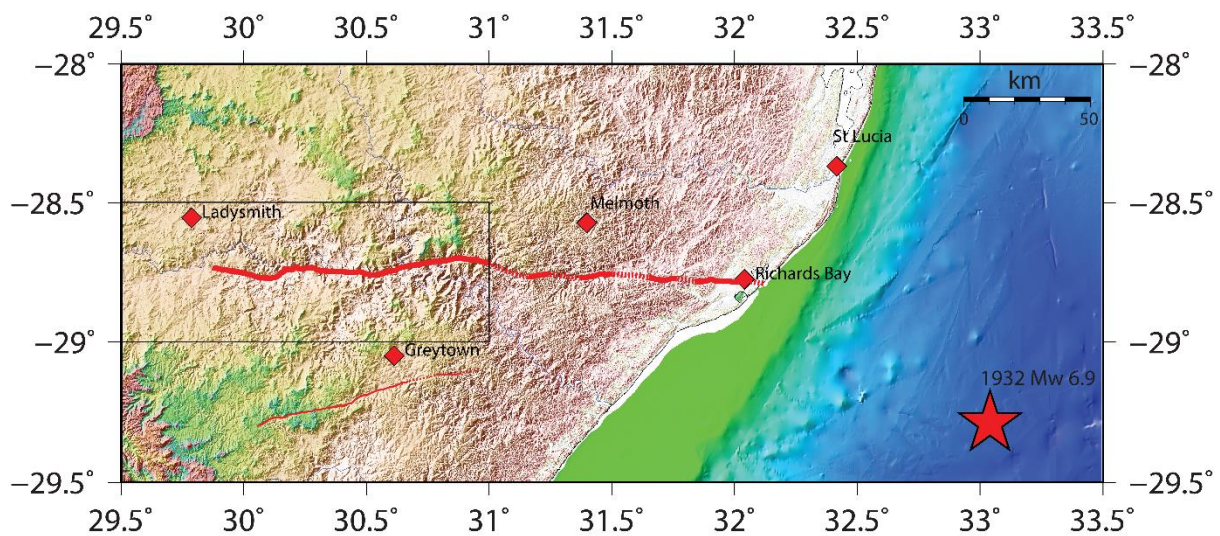
185 Figure 5: Tugela fault scarp highlighted with by a thick red line at areas where it is clearly 186 visible, the red star shows the epicentre of the 1932 M_w 6.9 St Lucia earthquake (ISC Bulletin). 187 The inset black block is the zoom in shown in Figure 4a.
