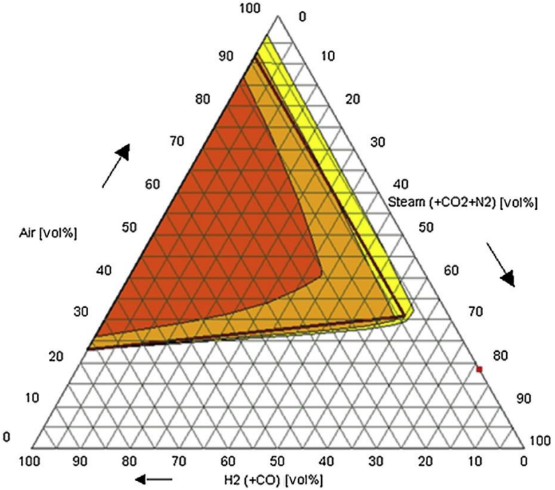
Figure 1: Shapiro diagram.
