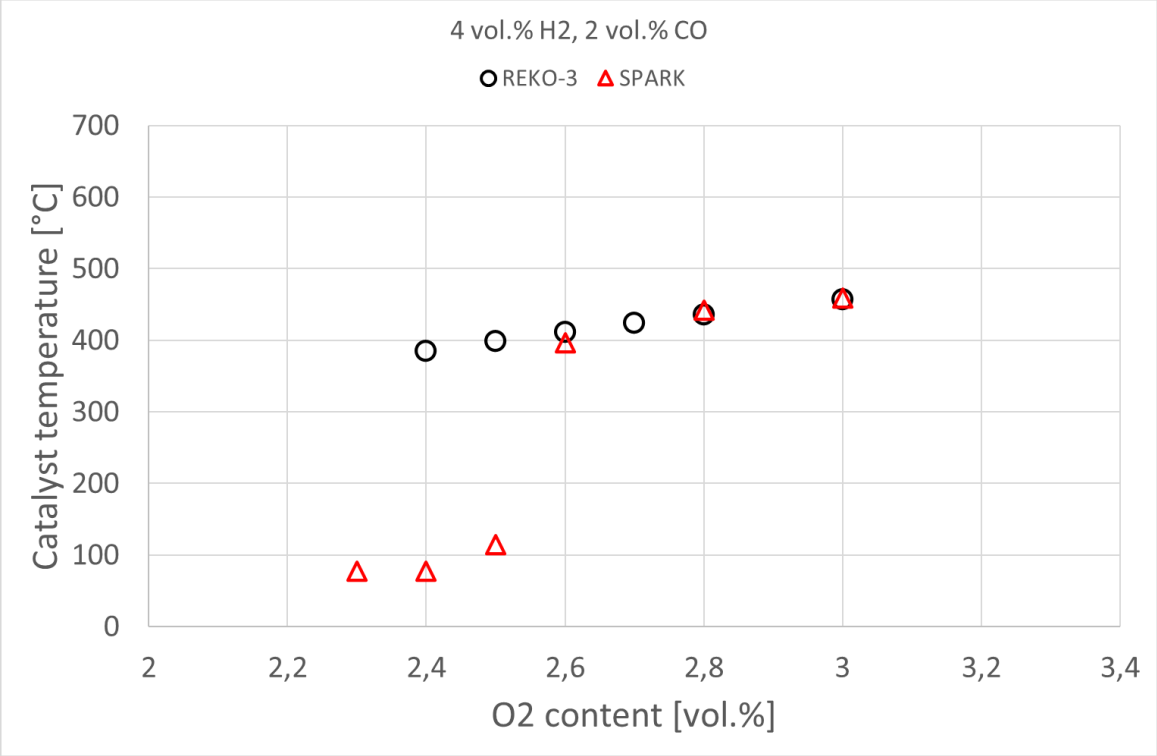
Figure 50: Catalyst temperature for a mixture with 4 vol.% H 2 , 2 vol.% CO, gas at 80°C and reduction of oxygen.
