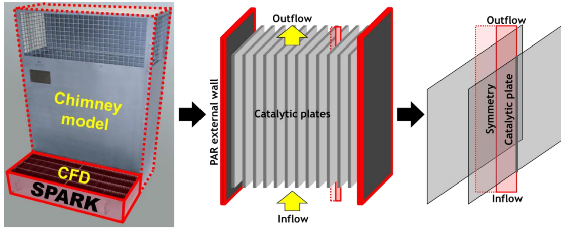
Figure 34: Recombiner configuration and numerical domain
