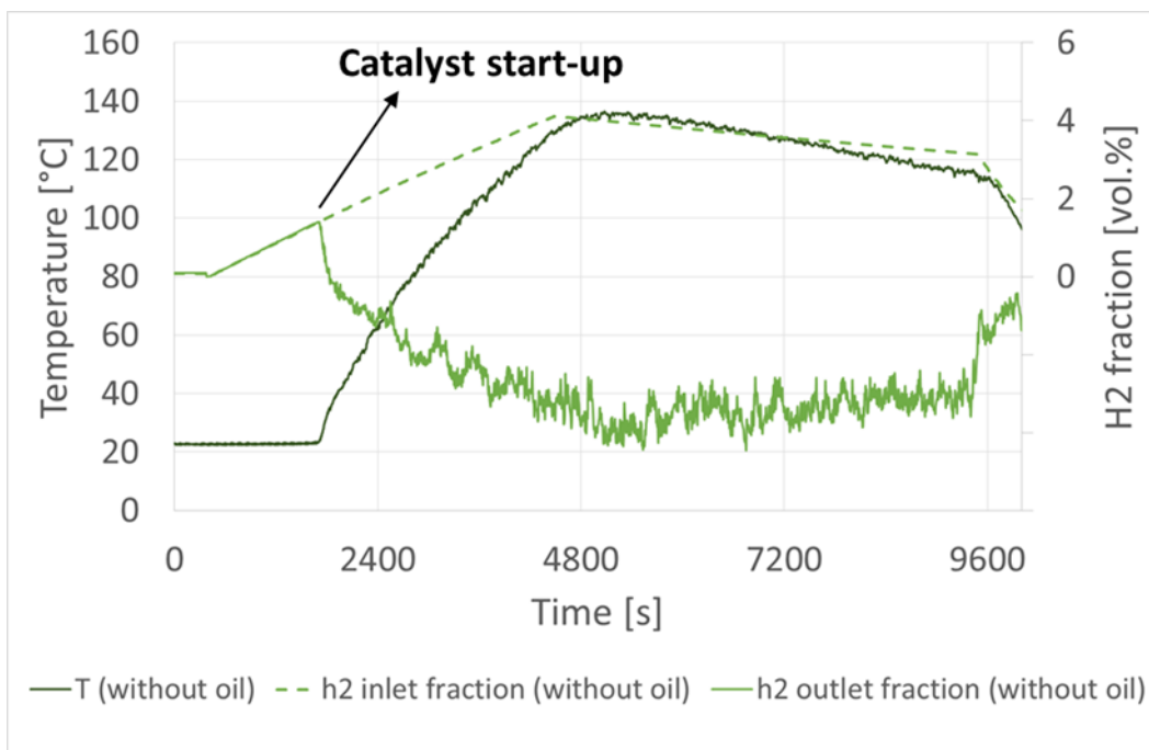
Figure 72: Behavior of catalyst without oil deposition under natural flow conditions (Reference test)
