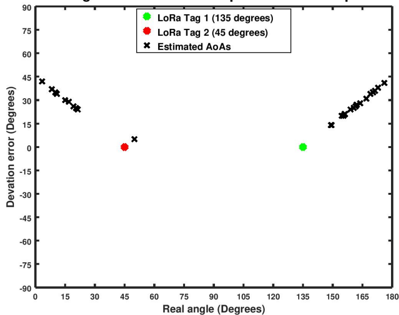
Two LoRa tags simultaneous reception with FFT equals to 2048
