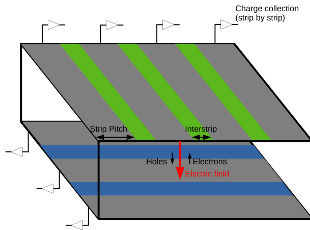
Figure 6.4: Principle of operation of a DSSD.
