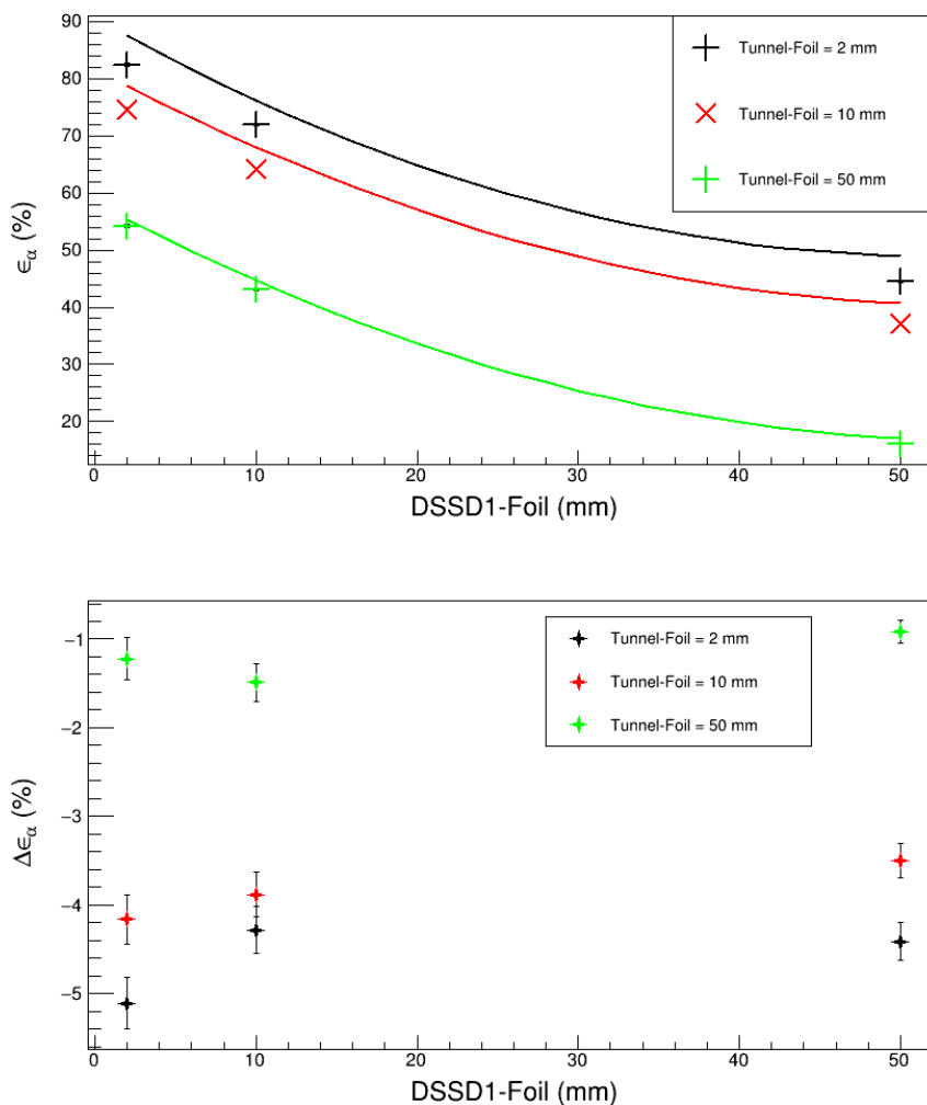
Figure 7.12: Top: Comparison between SEASON \alpha -particles simulated detection efficiencies without (full lines) and with (markers) the guard ring.
