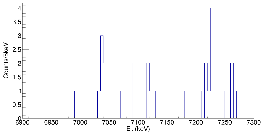
Figure B.21: \alpha -energy spectrum for \alpha -particles detected in coincidence with a \gamma -ray with 26.4 \text{ keV} < E_\gamma < 27.4 \text{ keV} .
