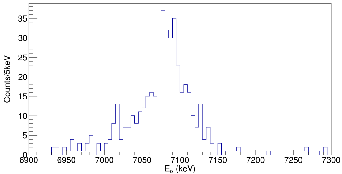
Figure B.7: \alpha -energy spectrum for \alpha -particles detected in coincidence with a \gamma -ray with 87.7 \text{ keV} < E_\gamma < 89.7 \text{ keV} .
