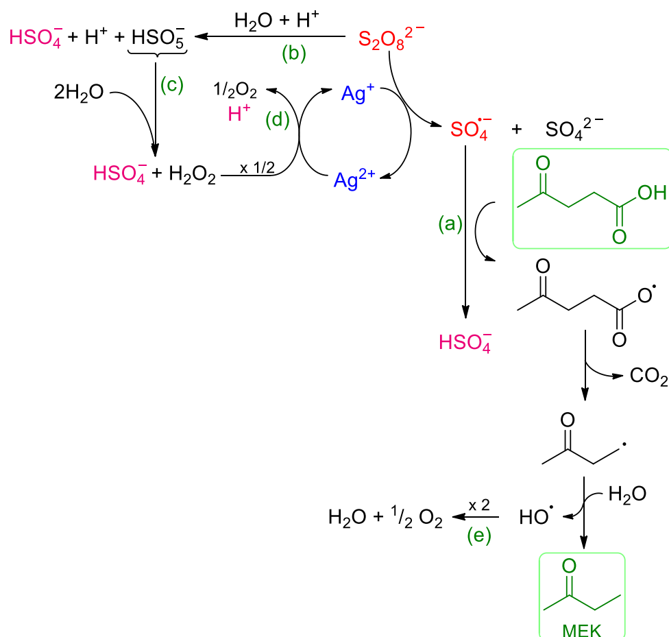
Scheme 26. Proposed mechanism
