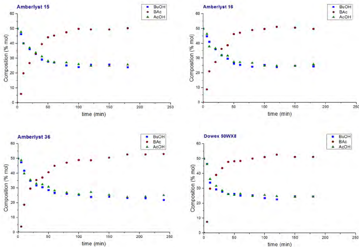
Figure 27. Kinetic study of the synthesis of butyl acetate from n -butanol and acetic acid (molar ratio 1:1) at 100°C in the presence of different ion exchange resins: A15, A16, A36 and D50 (catalyst loading: 5% w/w relative to n -butanol).
