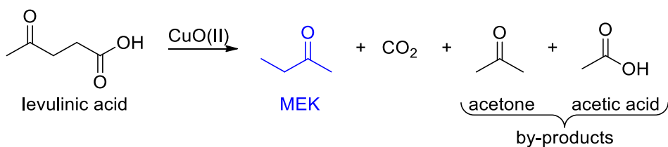
Scheme 22. Decarboxylation of levulinic acid using CuO as co-reagent (Gong et al, 2010) 437
