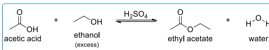
Scheme 1. Fischer esterification reaction for ethyl acetate synthesis
