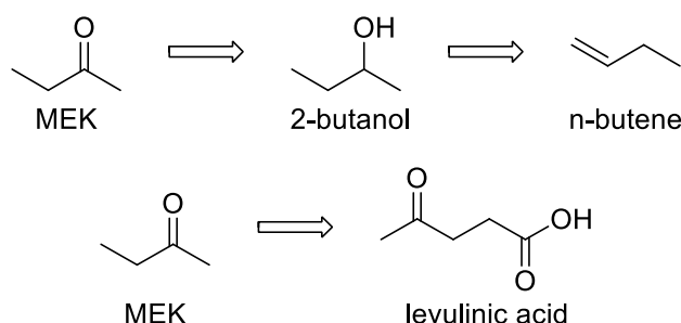
Figure 18. Identified chemical pathways for MEK synthesis
