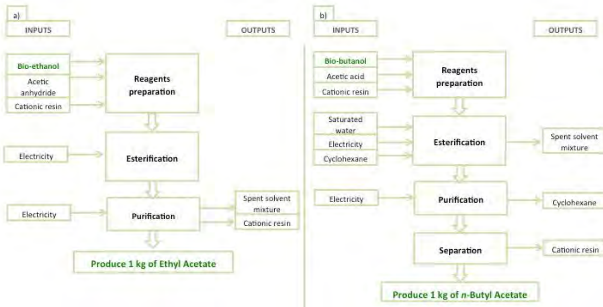
Figure 49. Process flowchart of the synthesis of ethyl and butyl acetates using bioethanol and bio-butanol, respectively
