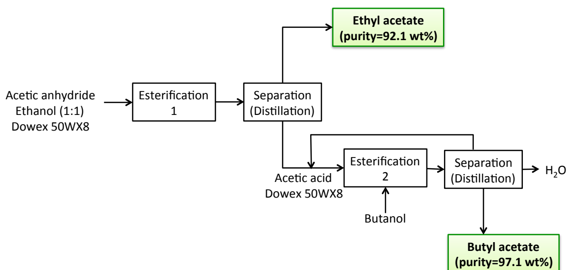
Figure 84. Coproduction process developed in this thesis work
