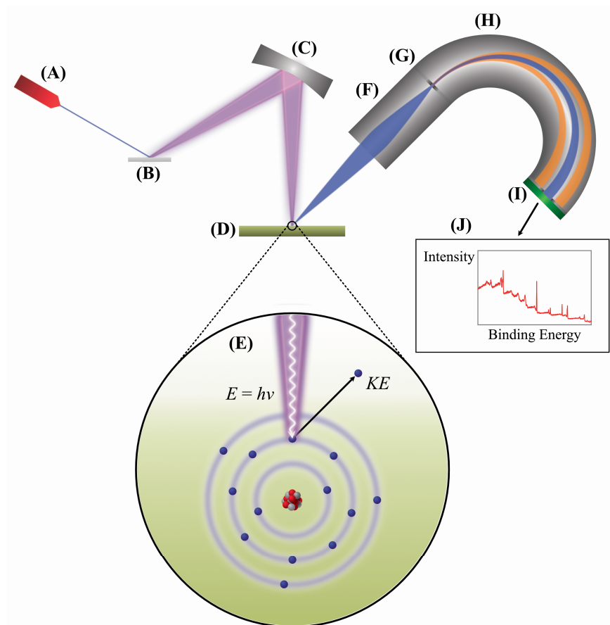
Figure 2.3: Schematic illustration of the setup for XPS analysis. The electron and X-ray beam path and important interactions with the material are described in the text. (A) Electron source; (B) metal anode producing X-rays; (C) monochromator focussing X-rays on the sample; (D) sample; (E) photoelectron emission process; (F) column slowing down and focussing photoelectrons; (G) entrance slit of hemispherical analyser; (H) hemispherical analyser; (I) detector; (J) photoelectron spectrum.
