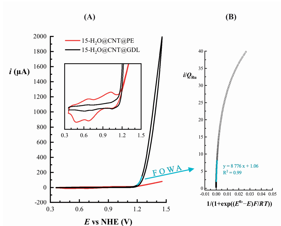
Figure 3.3: (A) Comparison of the CVs of 15-H 2 O@CNT on PE and on GDL. Both were taken in 1.0 M phosphate buffer (pH 7) with a scan rate of 10 mV s -1 . Data on PE was taken from Paper II and fully i R compensated. 109 The CV of the catalyst on GDL was 85 % i R compensated. The inset shows the reversible redox waves of the ruthenium centres and the lower loading of catalyst on the GDL. (B) With FOWA the TOF max of 15-H 2 O@CNT@GDL was estimated as 8 776 s -1 .
