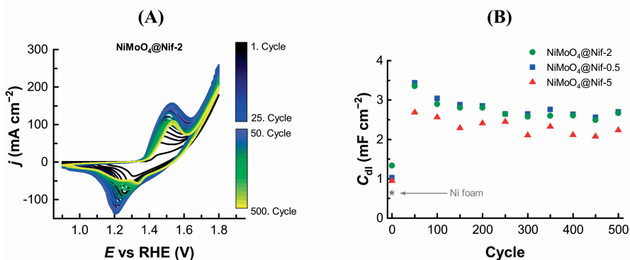
Figure 5.5: Electrochemical analysis of the nickel molybdate hydrate decorated nickel foams. (A) Cyclic voltammogram (CV) in 1 M KOH with 10 \text{ mV s}^{-1} . (B) The double layer capacitance ( C_{dl} ) over the 500 cycles indicate a stable high electrochemical surface area. Adapted from ACS Nano 2021, 15, 8, 13504 – 13515. Copyright 2021 The Authors. Published by American Chemical Society and licensed under CC BY 4.0.
