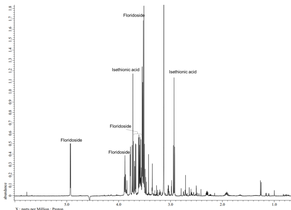
Figure 7: Annotated chromatograms of Fraction F1 (100% H 2 O) of A. armata with the ^1H -NMR spectrometer (0-5.5 ppm).
