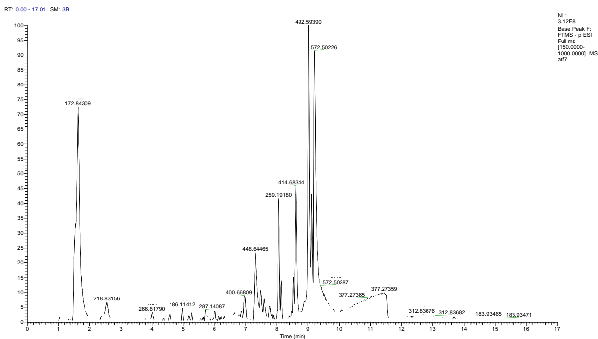
Figure 8: Chromatograms of the most active fraction “F6” (40% H 2 O-MeOH) of A. armata (A) and A. taxiformis (B) analysed with the UHPLC-ESI-HRMS spectrometer.
