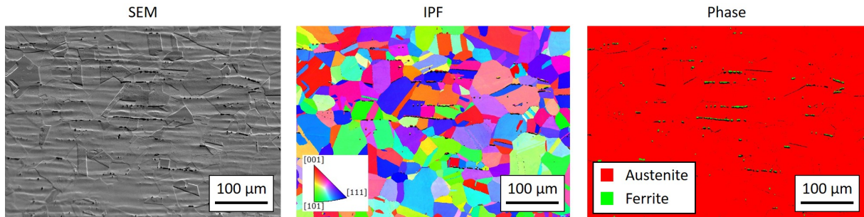
Figure 2.3: SEM observation, IPF map and phase map of the SS316L substrate.
