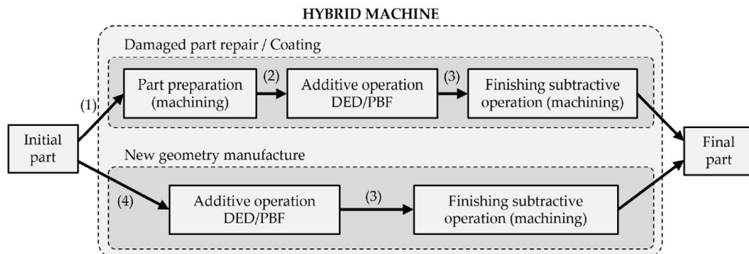
Figure 1.39: Flow chart and interactions in hybrid process for the damaged part repair or new part fabrication [123].
