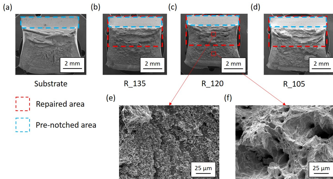
Figure 4.14: SEM micrographs of the Charpy test specimens after failure: (a) substrate, (b) R135, (c) R120, and (d) R105 with enlarged view from R120 highlighting (e) ductile screw failure and (f) ductile MVC failure.
