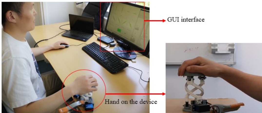
Figure 3.4 – Experiment setup
